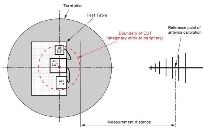
Figure C.1 – Measurement distance
