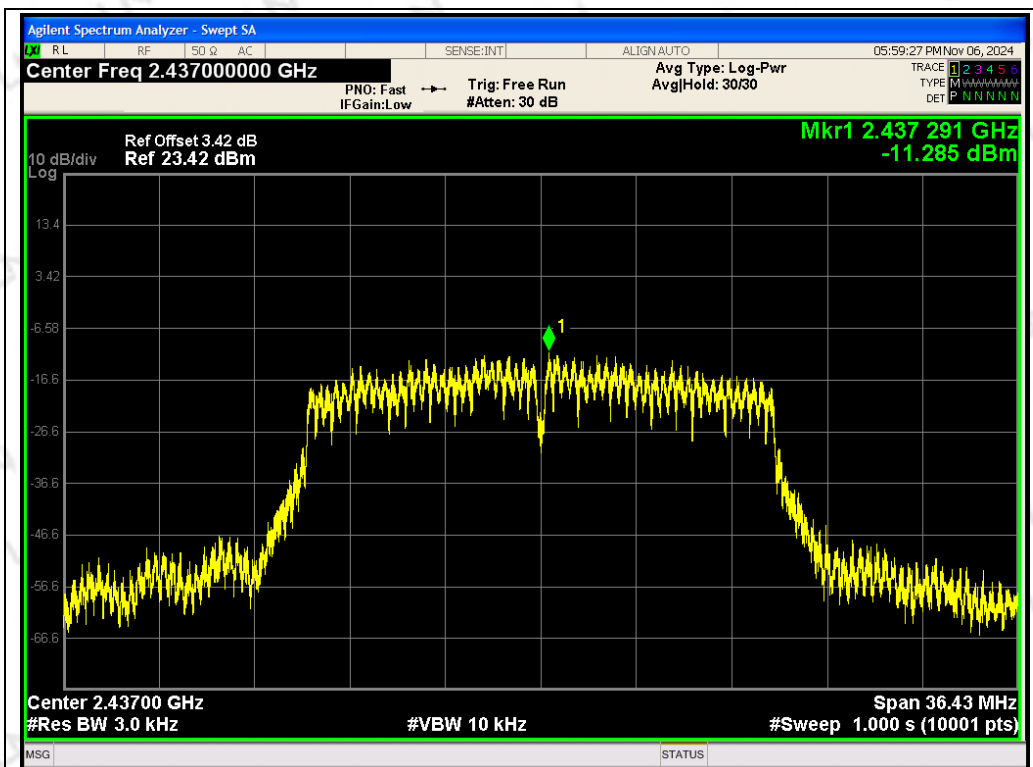
ANT 2 TX 802.11n/HT20 CH06: 2437MHz
