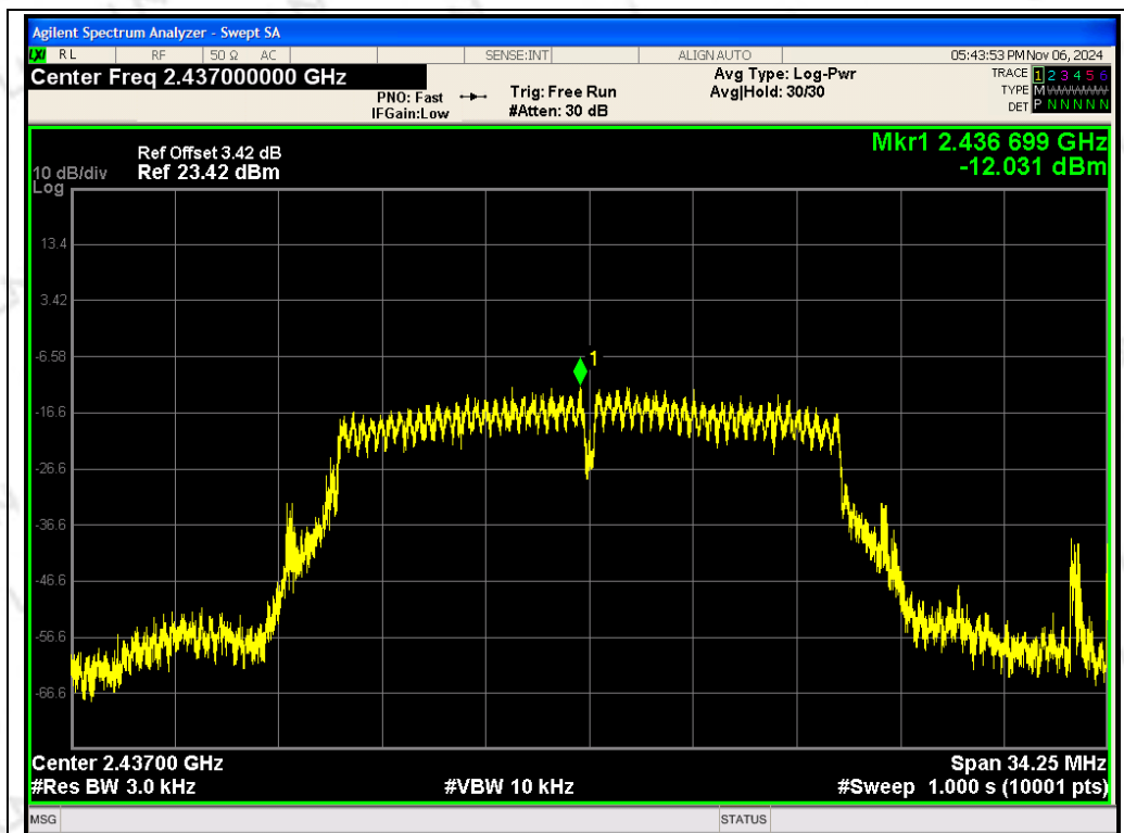
ANT 1 TX 802.11g CH06: 2437MHz
