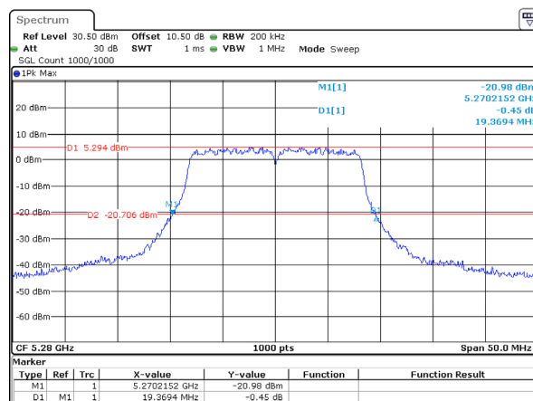
802.11a_5280MHz_Chain 2
