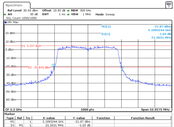
802.11ax20_5200MHz_RU_Full_Chain 2
