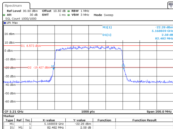
802.11ax80_5210MHz_RU_Full_Chain 3
