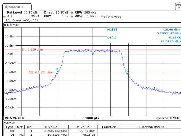
802.11a_5260MHz_Chain 2
