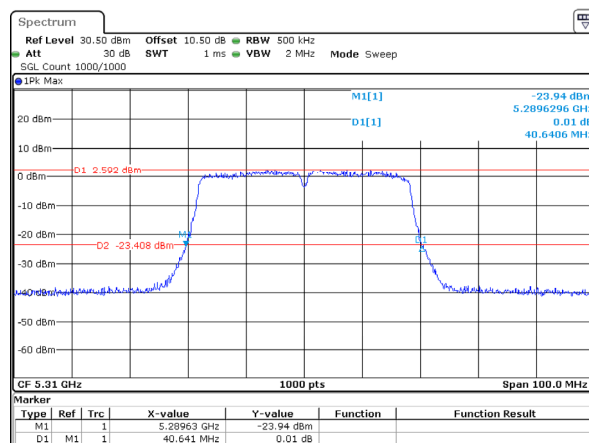
802.11ac40_5310MHz_Chain 0
