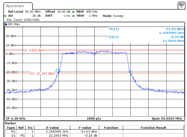
802.11ax20_5180MHz_RU_Full_Chain 3
