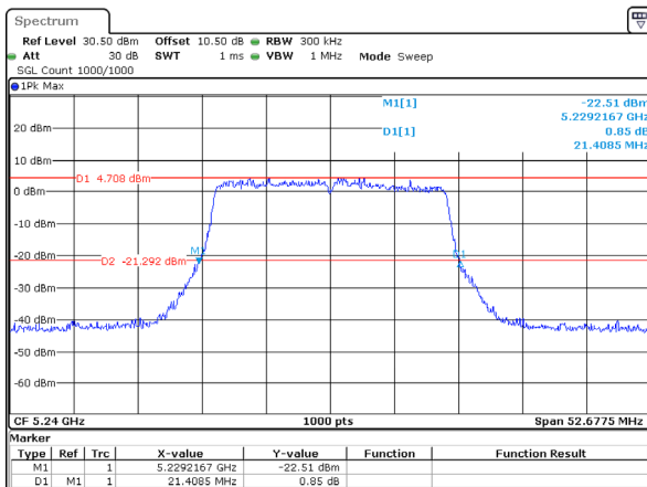
802.11ax20_5240MHz_RU_Full_Chain 2
