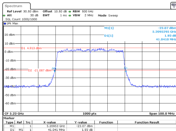
802.11ax40_5230MHz_RU_Full_Chain 3
