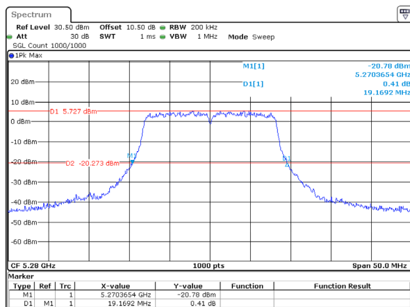
802.11a_5280MHz_Chain 3
