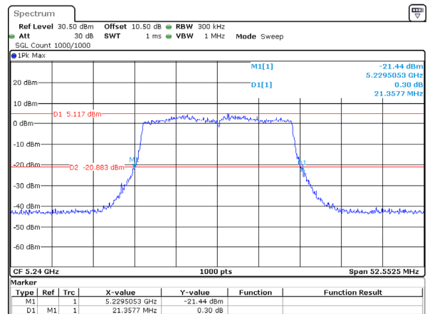
802.11ax20_5240MHz_RU_Full_Chain 3
