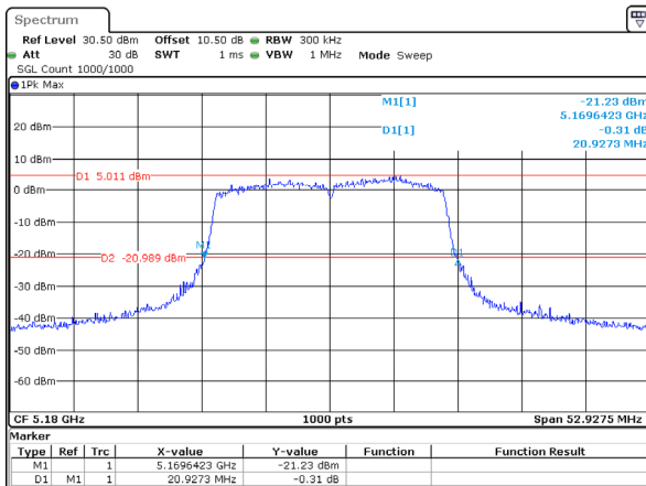
802.11ax20_5180MHz_RU_Full_Chain 2
