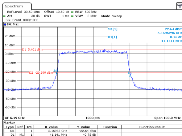
802.11ax40_5190MHz_RU_Full_Chain 3
