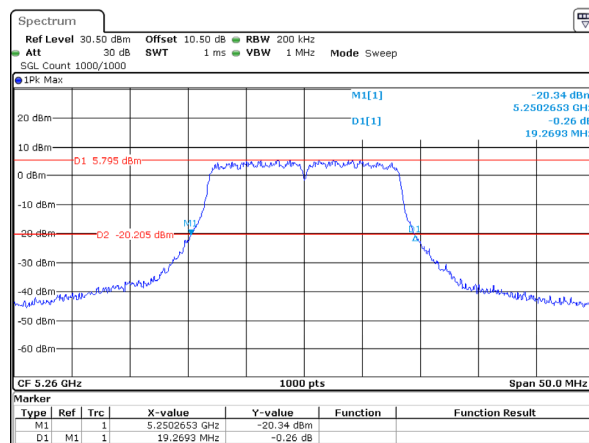
802.11a_5260MHz_Chain 3
