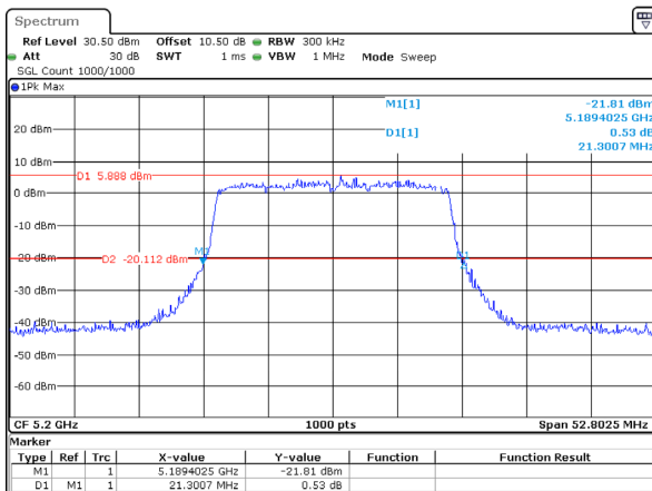
802.11ax20_5200MHz_RU_Full_Chain 3
