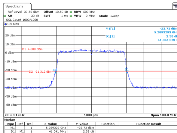
802.11ax40_5310MHz_RU_Full_Chain 1
