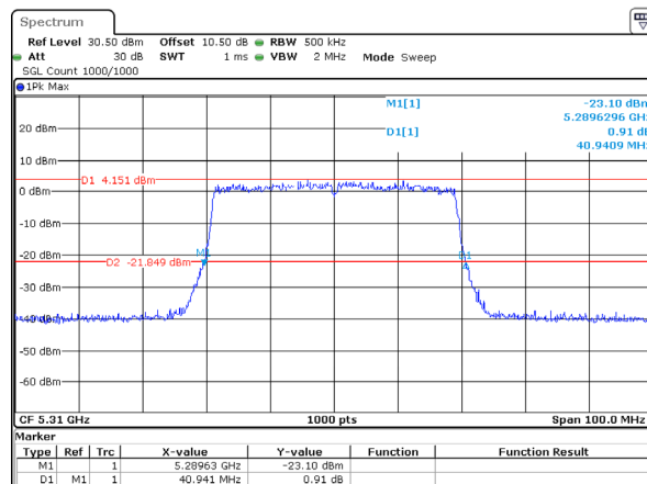
802.11ax40_5310MHz_RU_Full_Chain 0
