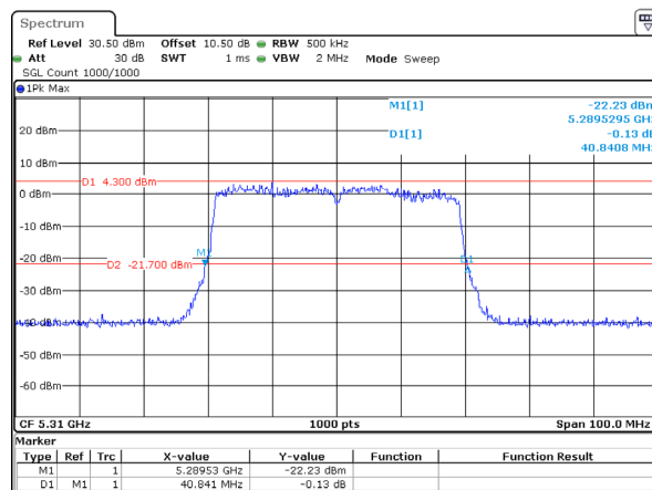
802.11ax40_5310MHz_RU_Full_Chain 2
