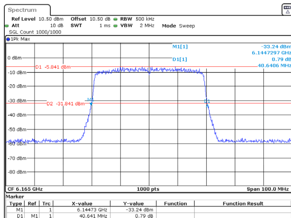
802.11ax40_6165MHz_RU_Full_Chain 1 40.641MHz
