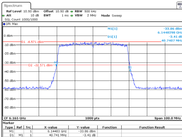
802.11ax40_6165MHz_RU_Full_Chain 3 40.741MHz
