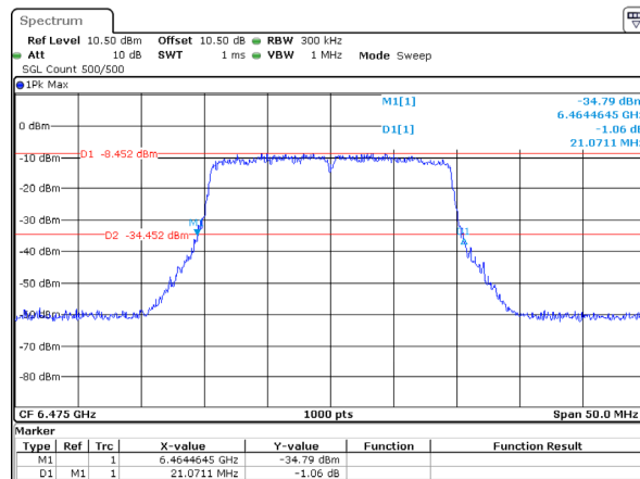
802.11ax20_6475MHz_RU_Full_Chain 2 21.071MHz
