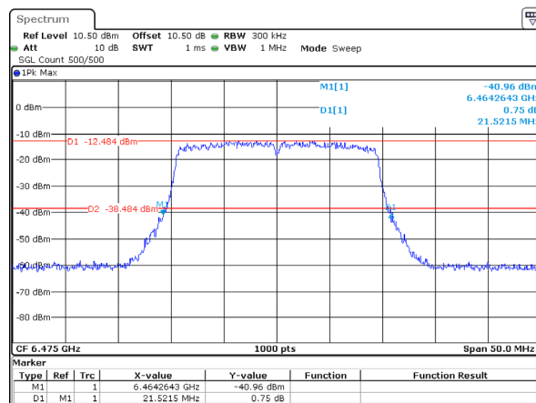
802.11ax20_6475MHz_RU_Full_Chain 0 21.522MHz
