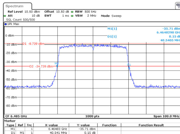
802.11ax40_6485MHz_RU_Full_Chain 1 40.541MHz
