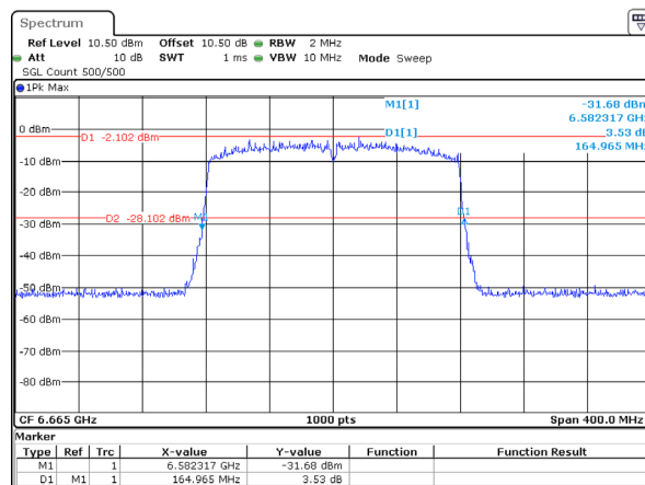
802.11ax160_6665MHz_RU_Full_Chain 3 164.965MHz
