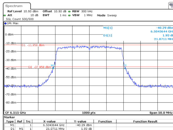
802.11ax20_6515MHz_RU_Full_Chain 1 21.071MHz
