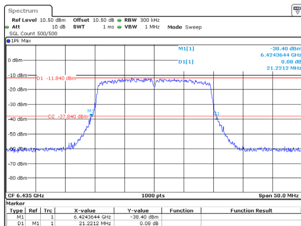
802.11ax20_6435MHz_RU_Full_Chain 0 21.221MHz
