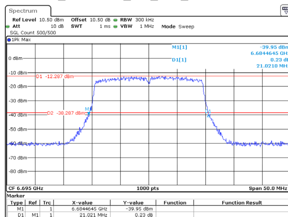
802.11ax20_6695MHz_RU_Full_Chain 0 21.021MHz
