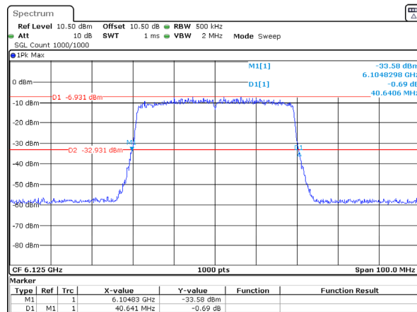
802.11ax40_6125MHz_RU_Full_Chain 1 40.641MHz
