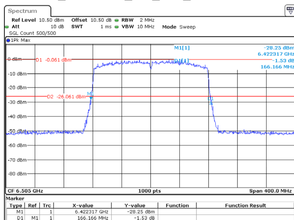
802.11ax160_6505MHz_RU_Full_Chain 2 166.166MHz
