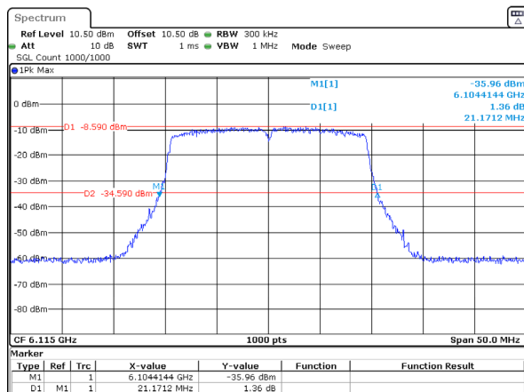
802.11ax20_6115MHz_RU_Full_Chain 2 21.171MHz
