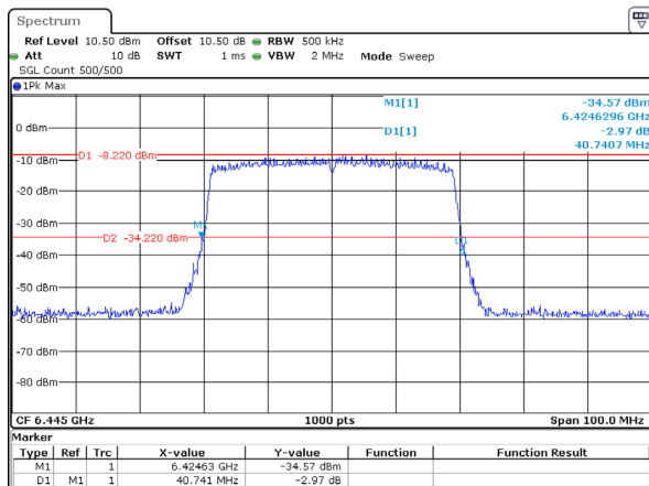
802.11ax40_6445MHz_RU_Full_Chain 0 40.741MHz
