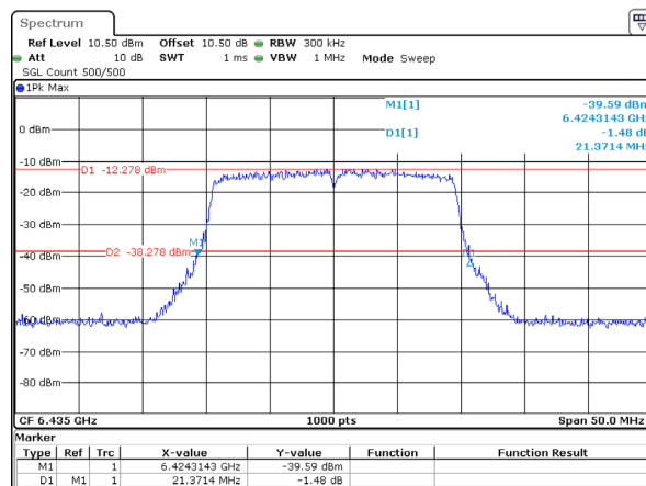
802.11ax20_6435MHz_RU_Full_Chain 1 21.371MHz
