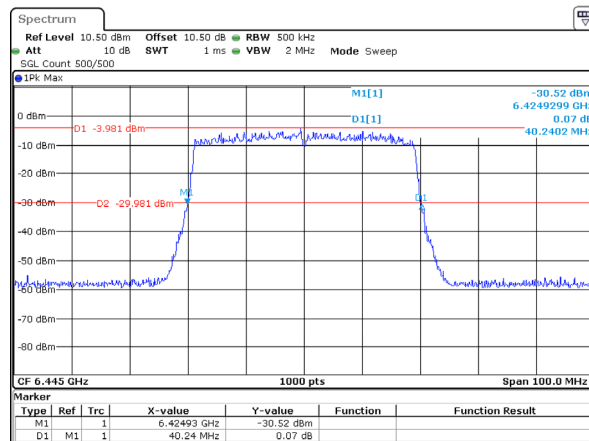
802.11ax40_6445MHz_RU_Full_Chain 2 40.240MHz
