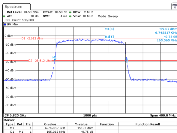
802.11ax160_6825MHz_RU_Full_Chain 1 165.365MHz
