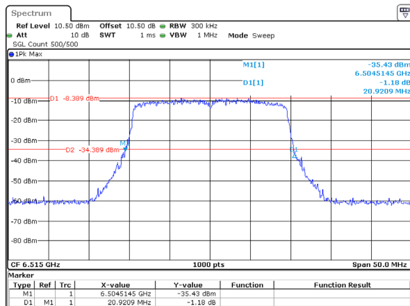
802.11ax20_6515MHz_RU_Full_Chain 2 20.921MHz
