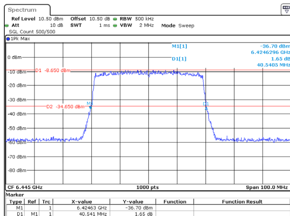
802.11ax40_6445MHz_RU_Full_Chain 1 40.541MHz
