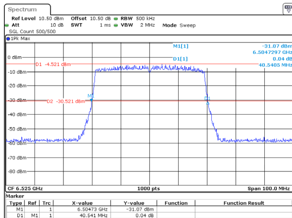
802.11ax40_6525MHz_RU_Full_Chain 2 40.541MHz
