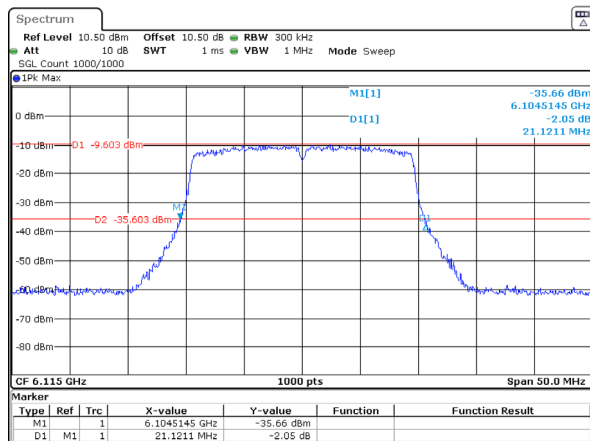
802.11ax20_6115MHz_RU_Full_Chain 0 21.121MHz
