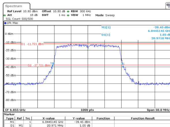
802.11ax20_6855MHz_RU_Full_Chain 1 20.971MHz
