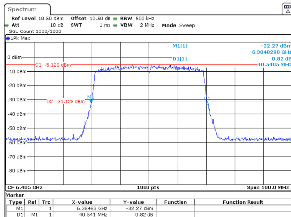
802.11ax40_6405MHz_RU_Full_Chain 2 40.541MHz
