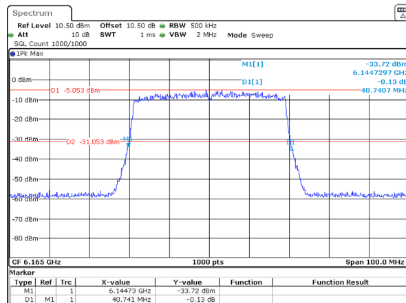
802.11ax40_6165MHz_RU_Full_Chain 0 40.741MHz
