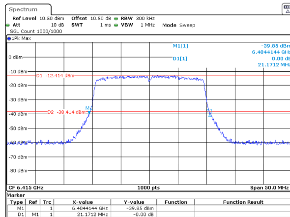
802.11ax20_6415MHz_RU_Full_Chain 3 21.171MHz
