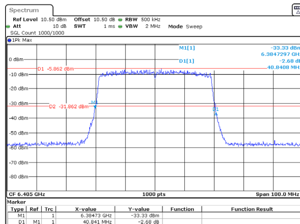
802.11ax40_6405MHz_RU_Full_Chain 1 40.841MHz
