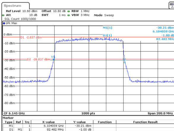
802.11ax80_6145MHz_RU_Full_Chain 1 82.482MHz
