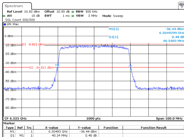
802.11ax40_6525MHz_RU_Full_Chain 1 40.340MHz
