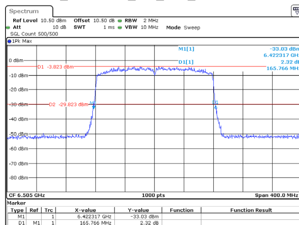
802.11ax160_6505MHz_RU_Full_Chain 3 165.766MHz
