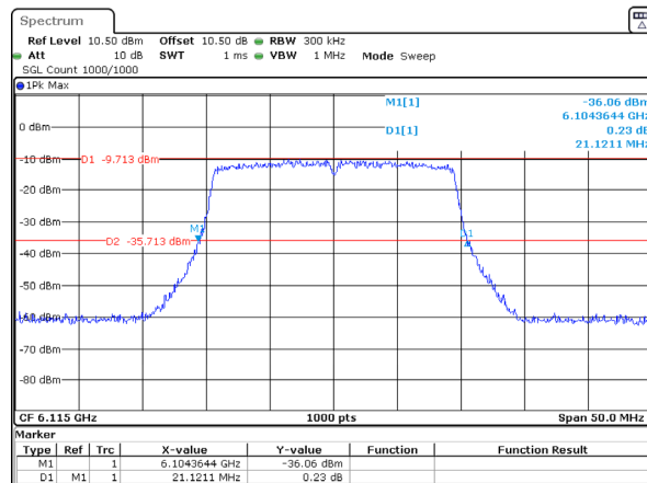
802.11ax20_6115MHz_RU_Full_Chain 1 21.121MHz
