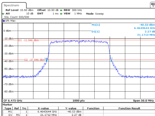
802.11ax20_6475MHz_RU_Full_Chain 3 21.171MHz
