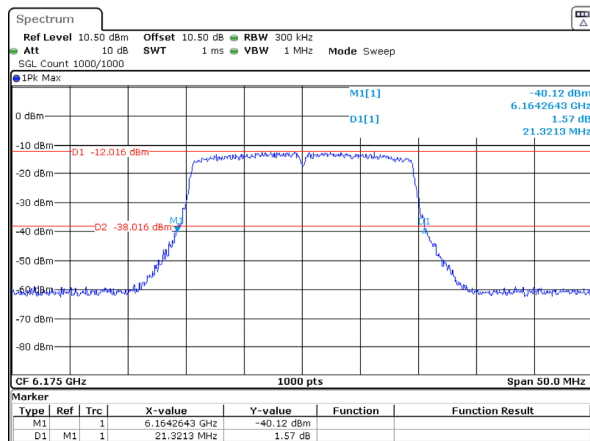
802.11ax20_6175MHz_RU_Full_Chain 3 21.321MHz
