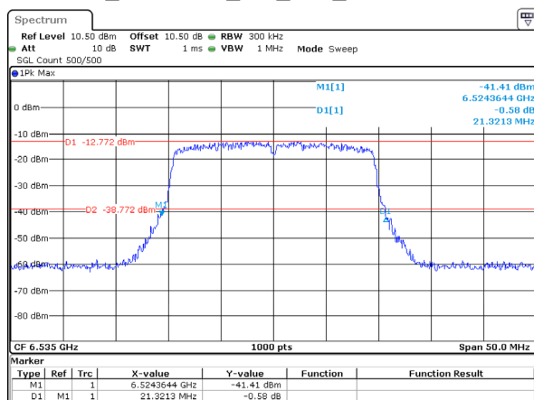
802.11ax20_6535MHz_RU_Full_Chain 0 21.321MHz
