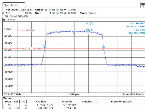
802.11ax160_6825MHz_RU_Full_Chain 2 165.365MHz
