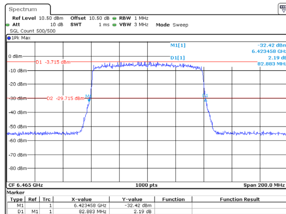
802.11ax80_6465MHz_RU_Full_Chain 1 82.883MHz
