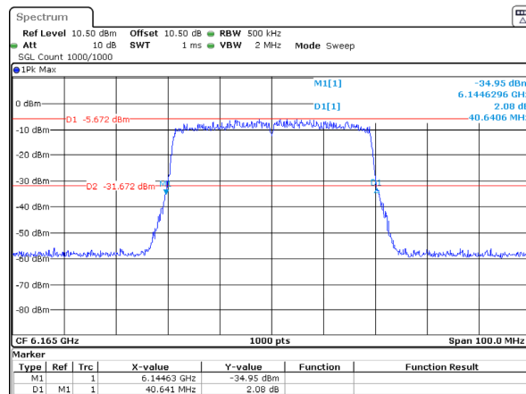
802.11ax40_6165MHz_RU_Full_Chain 2 40.641MHz
