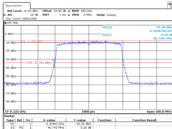
802.11ax40_6125MHz_RU_Full_Chain 3 40.741MHz
