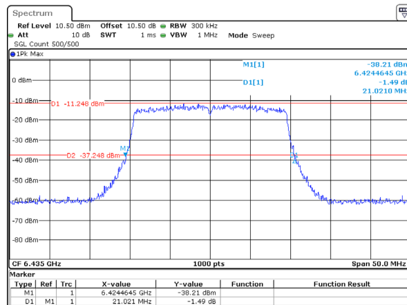
802.11ax20_6435MHz_RU_Full_Chain 3 21.021MHz
