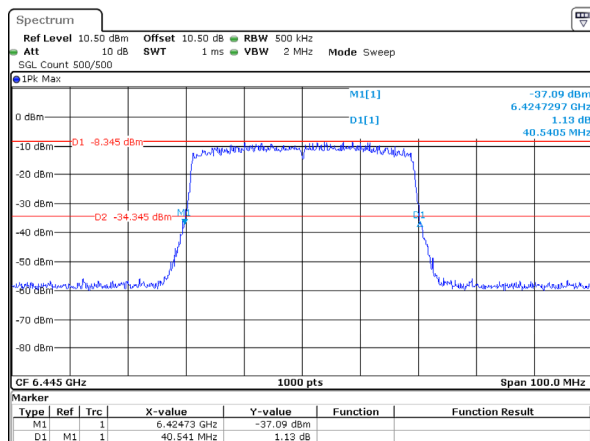
802.11ax40_6445MHz_RU_Full_Chain 3 40.541MHz
