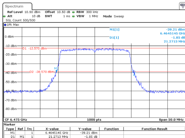
802.11ax20_6475MHz_RU_Full_Chain 1 21.271MHz
