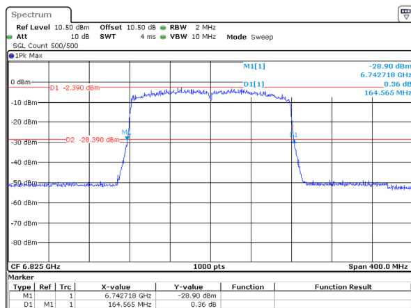
802.11ax160_6825MHz_RU_Full_Chain 3 164.565MHz
