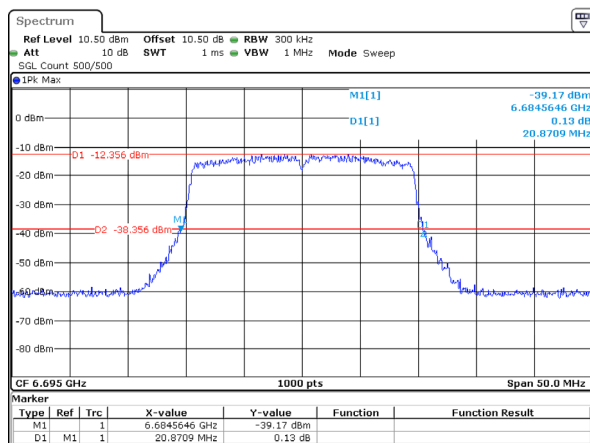
802.11ax20_6695MHz_RU_Full_Chain 1 20.871MHz
