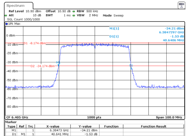
802.11ax40_6405MHz_RU_Full_Chain 3 40.641MHz
