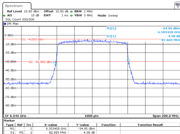
802.11ax80_6545MHz_RU_Full_Chain 1 82.683MHz
