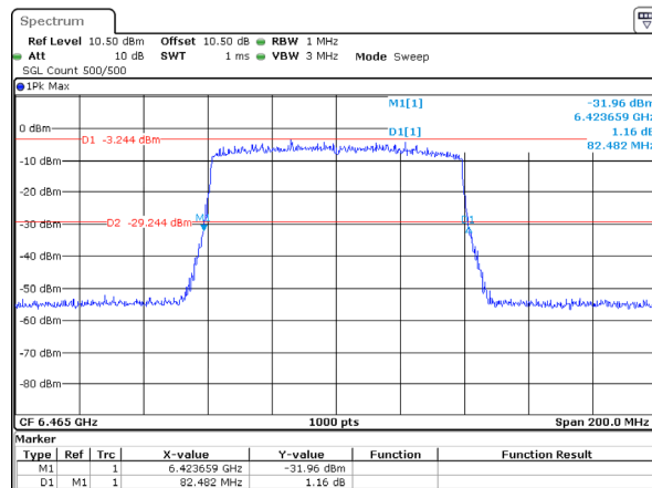
802.11ax80_6465MHz_RU_Full_Chain 0 82.482MHz
