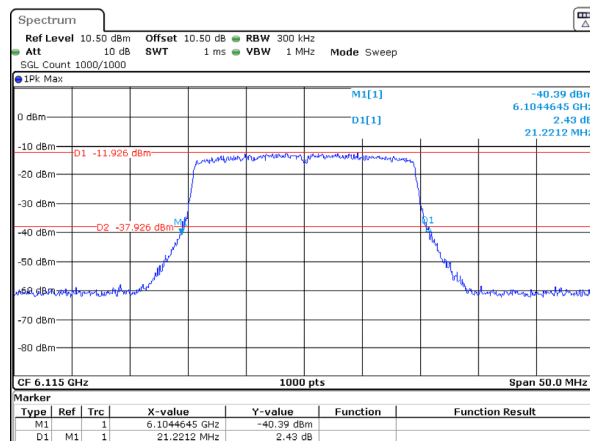
802.11ax20_6115MHz_RU_Full_Chain 3 21.221MHz
