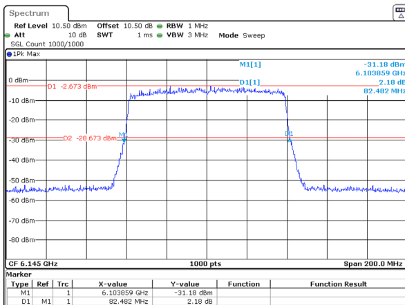
802.11ax80_6145MHz_RU_Full_Chain 0 82.482MHz
