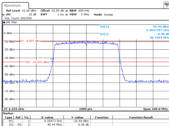
802.11ax40_6525MHz_RU_Full_Chain 0 40.440MHz
