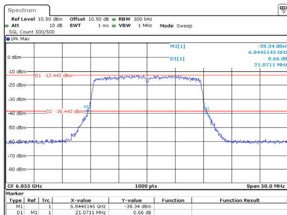
802.11ax20_6855MHz_RU_Full_Chain 0 21.071MHz
