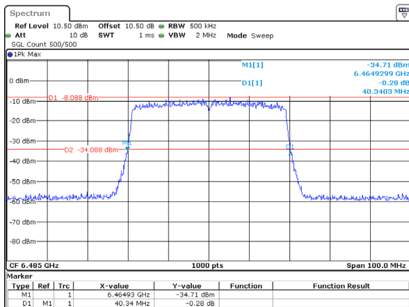
802.11ax40_6485MHz_RU_Full_Chain 0 40.340MHz
