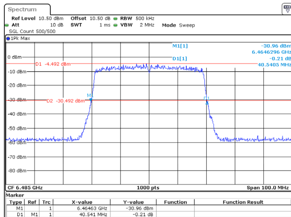
802.11ax40_6485MHz_RU_Full_Chain 2 40.541MHz
