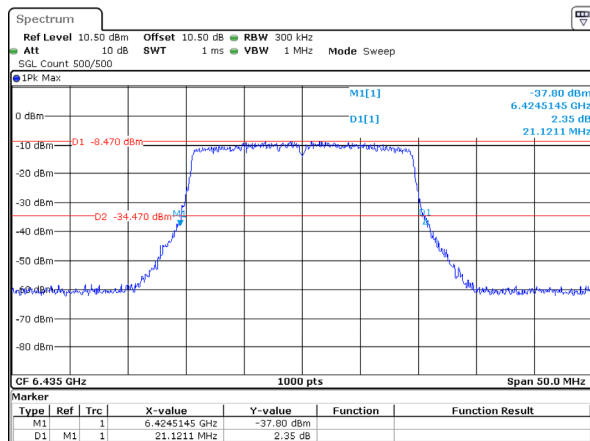
802.11ax20_6435MHz_RU_Full_Chain 2 21.121MHz
