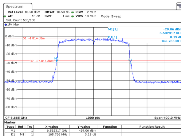
802.11ax160_6665MHz_RU_Full_Chain 2 165.766MHz
