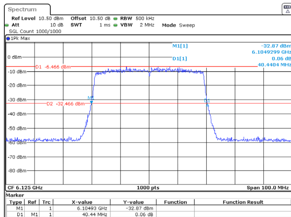
802.11ax40_6125MHz_RU_Full_Chain 2 40.440MHz
