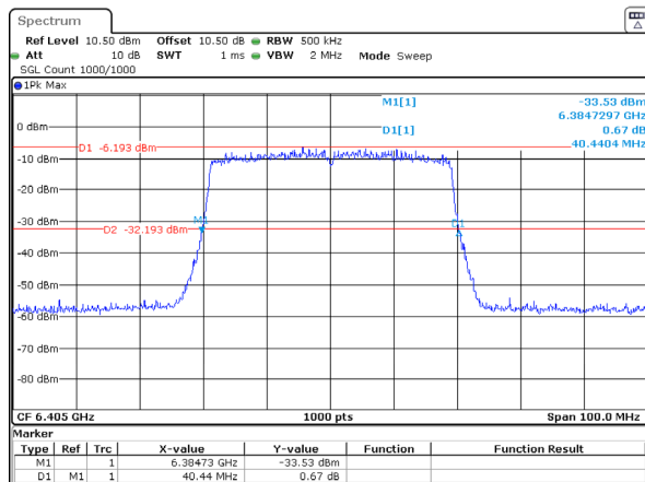
802.11ax40_6405MHz_RU_Full_Chain 0 40.440MHz
