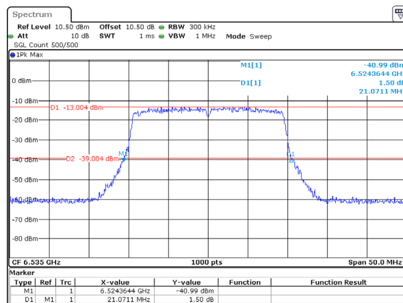
802.11ax20_6535MHz_RU_Full_Chain 1 21.071MHz
