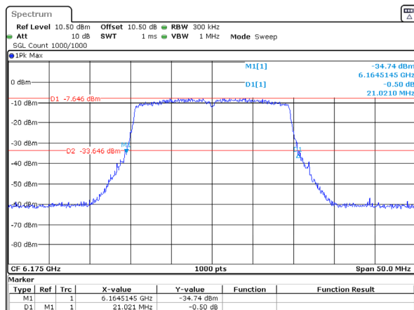
802.11ax20_6175MHz_RU_Full_Chain 2 21.021MHz
