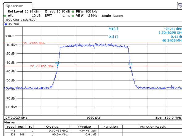
802.11ax40_6525MHz_RU_Full_Chain 3 40.340MHz
