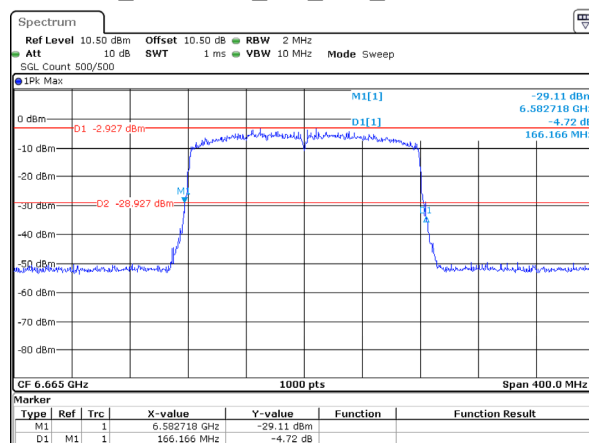
802.11ax160_6665MHz_RU_Full_Chain 1 166.166MHz
