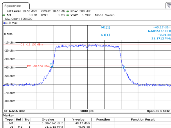
802.11ax20_6515MHz_RU_Full_Chain 3 21.171MHz
