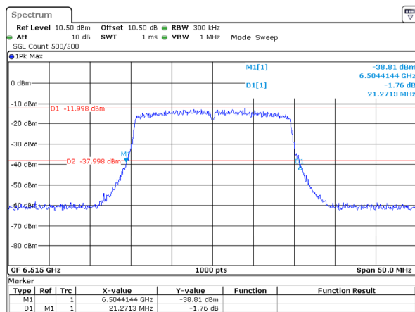
802.11ax20_6515MHz_RU_Full_Chain 0 21.271MHz
