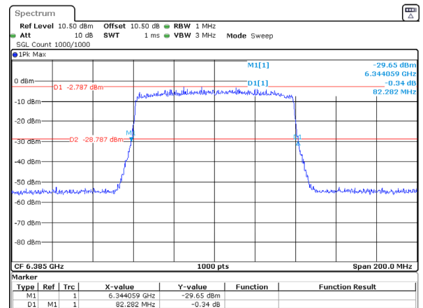
802.11ax80_6385MHz_RU_Full_Chain 1 82.282MHz
