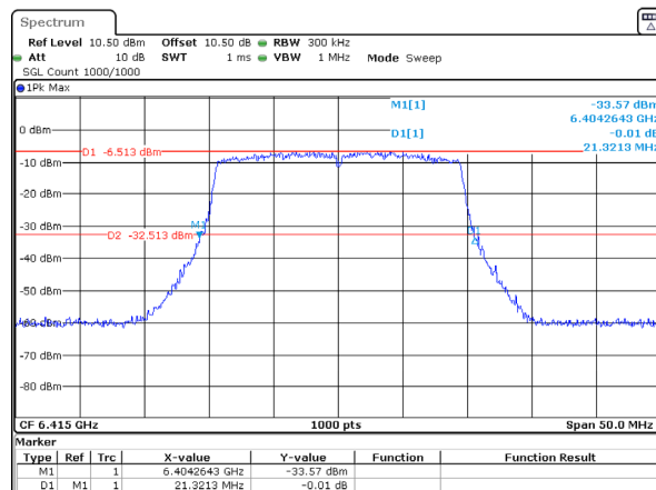
802.11ax20_6415MHz_RU_Full_Chain 2 21.321MHz
