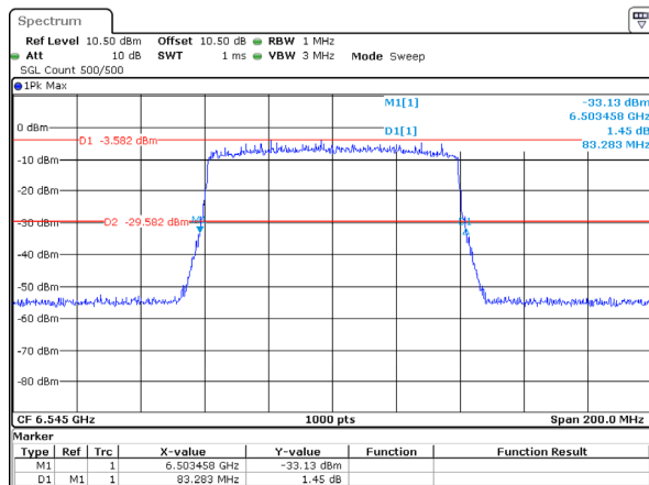
802.11ax80_6545MHz_RU_Full_Chain 0 83.283MHz
