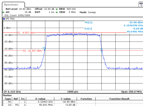
802.11ax40_6125MHz_RU_Full_Chain 0 40.641MHz
