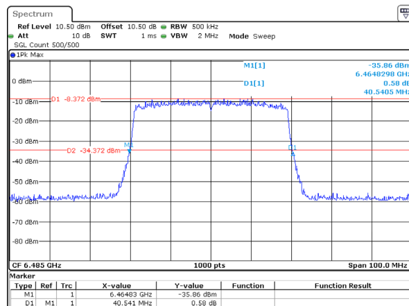
802.11ax40_6485MHz_RU_Full_Chain 3 40.541MHz
