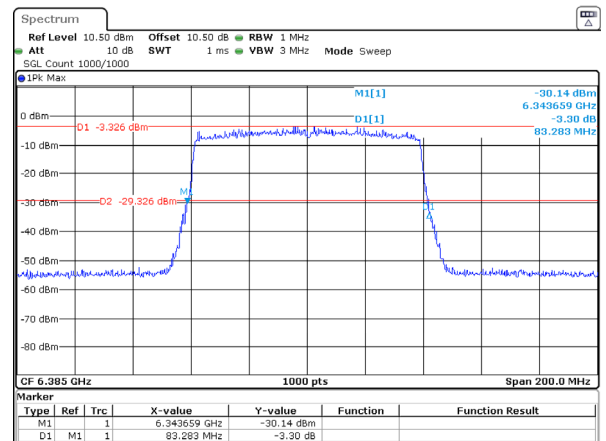
802.11ax80_6385MHz_RU_Full_Chain 0 83.283MHz
