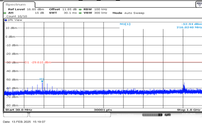
SRD 2.4G_Ant1_2474_30-1000
