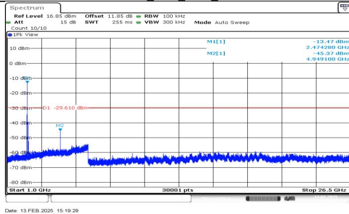
SRD 2.4G_Ant1_2474_1000-26500
