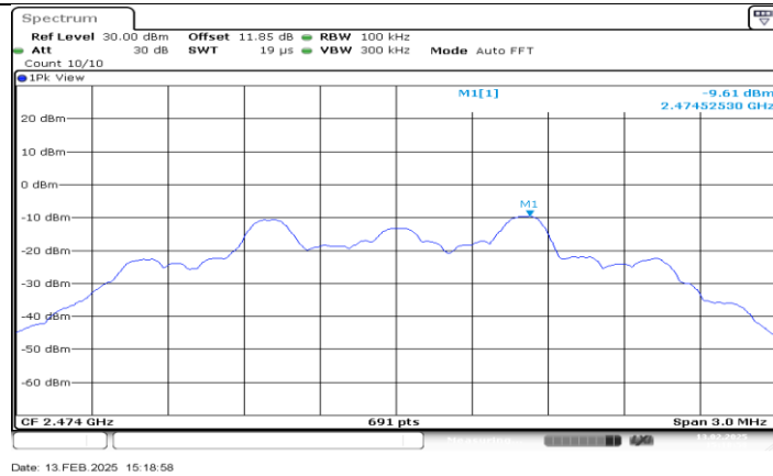
SRD 2.4G_Ant1_2474_0-Reference
