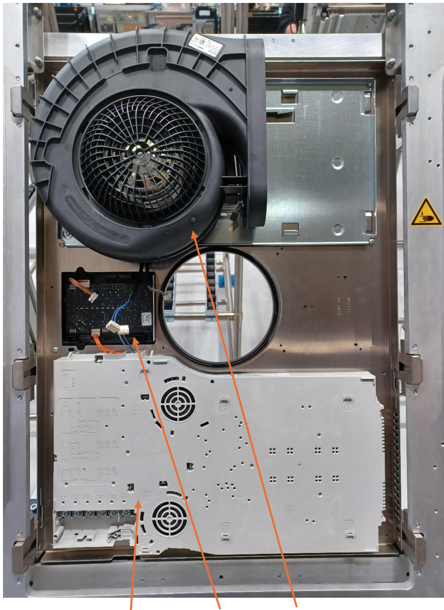
Internal view generator, touch control and blower
