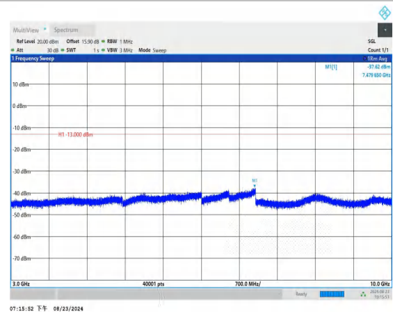
Band12_3MHz_QPSK_23165_1RB#0_3000~10000_3000~1000
