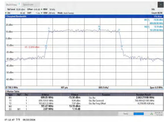
Band12-3MHz-16QAM-23025-15RB#0-PASS
