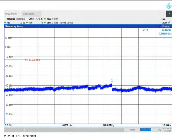
Band12_10MHz_QPSK_23130_1RB#0_3000~10000_3000~10000
