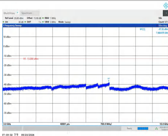
Band12_1.4MHz_QPSK_23017_1RB#0_3000~10000_3000~10
