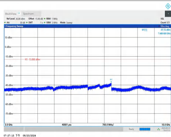
Band12_10MHz_QPSK_23060_1RB#0_3000~10000_3000~1000
