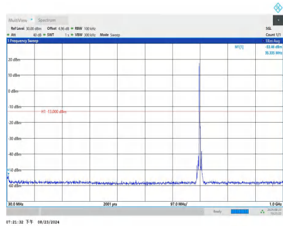
Band12_5MHz_QPSK_23095_1RB#0_30~1000_30~1000
