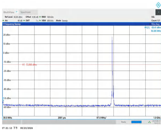
Band12_5MHz_QPSK_23035_1RB#0_30~1000_30~1000
