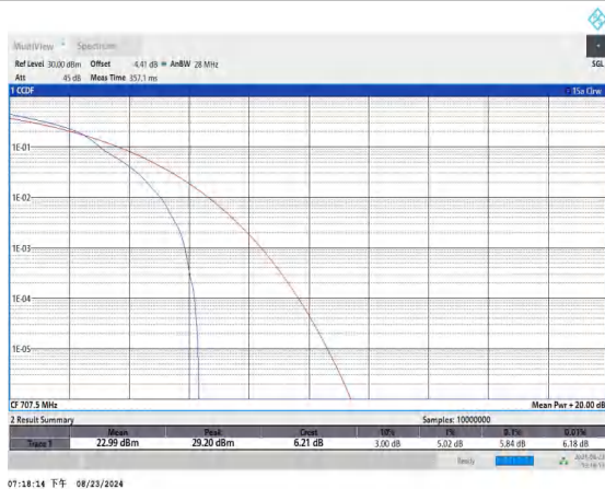
Band12-3MHz-16QAM-23095-1RB#0-PASS
