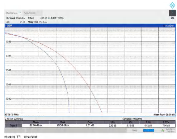
Band12-5MHz-16QAM-23035-25RB#0-PASS
