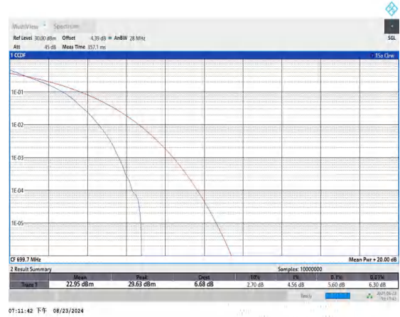
Band12-1.4MHz-QPSK-23017-6RB#0-PASS
