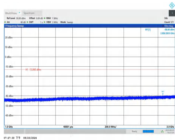
Band12_10MHz_QPSK_23095_1RB#0_1000~3000_1000~3000
