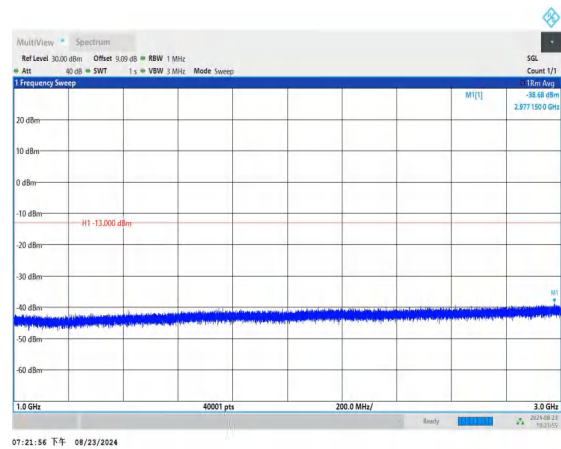
Band12_5MHz_QPSK_23155_1RB#0_1000~3000_1000~3000
