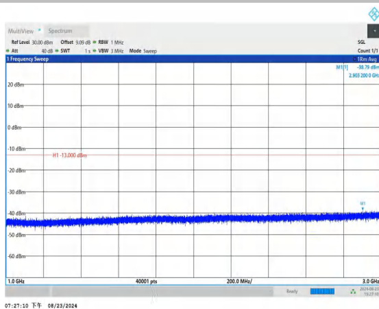
Band12_10MHz_QPSK_23060_1RB#0_1000~3000_1000~3000
