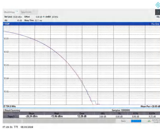
Band12-10MHz-QPSK-23060-1RB#0-PASS
