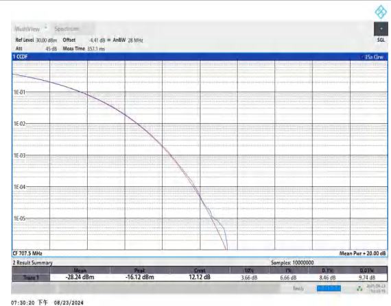
Band12-10MHz-QPSK-23095-50RB#0-PASS
