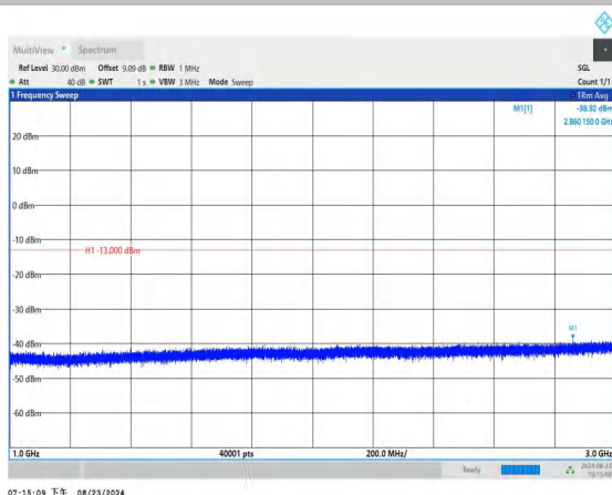
Band12_3MHz_QPSK_23025_1RB#0_1000~3000_1000~3000
