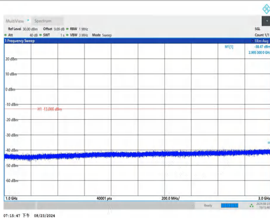
Band12_3MHz_QPSK_23165_1RB#0_1000~3000_1000~3000
