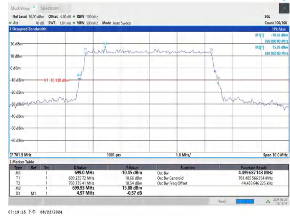
Band12-5MHz-16QAM-23035-25RB#0-PASS
