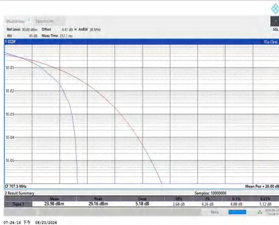
Band12-5MHz-QPSK-23095-1RB#0-PASS
