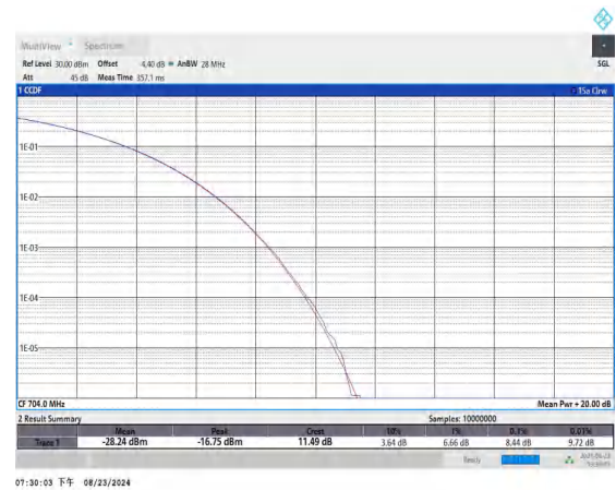
Band12-10MHz-16QAM-23060-50RB#0-PASS
