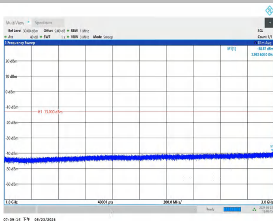
Band12_1.4MHz_QPSK_23095_1RB#0_1000~3000_1000~300
