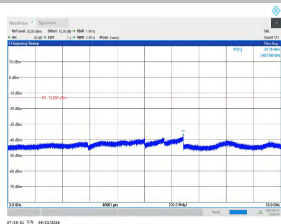
Band12_1.4MHz_QPSK_23095_1RB#0_3000~10000_3000~10
