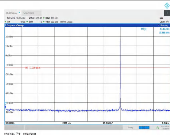
Band12_1.4MHz_QPSK_23095_1RB#0_30~1000_30~1000
