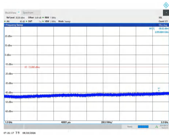
Band12_5MHz_QPSK_23035_1RB#0_1000~3000_1000~3000
