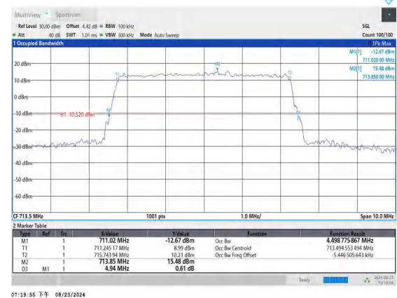
Band12-5MHz-16QAM-23155-25RB#0-PASS
