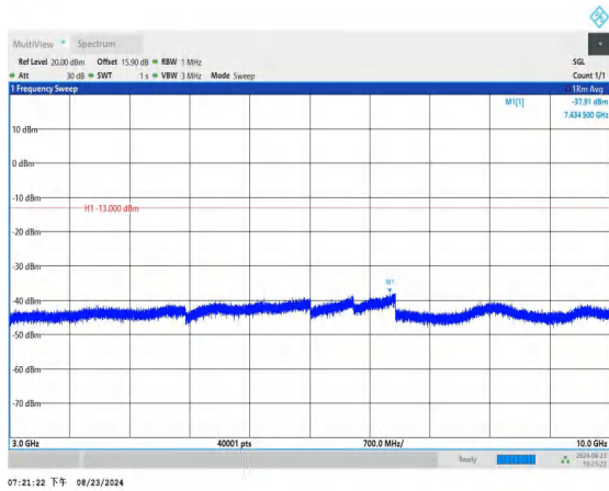
Band12_5MHz_QPSK_23035_1RB#0_3000~10000_3000~1000
