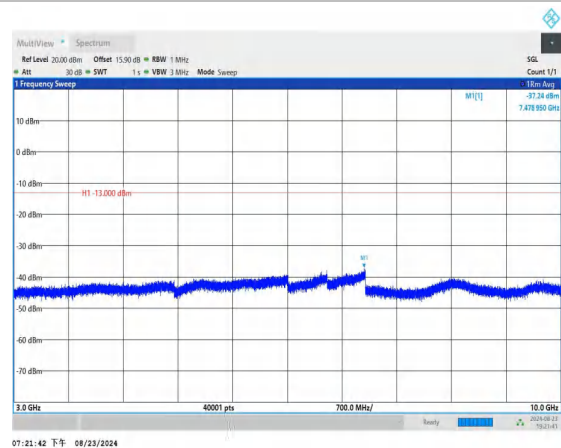
Band12_5MHz_QPSK_23095_1RB#0_3000~10000_3000~1000
