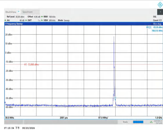
Band12_3MHz_QPSK_23025_1RB#0_30~1000_30~1000
