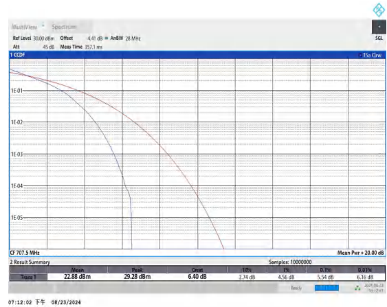
Band12-1.4MHz-QPSK-23095-6RB#0-PASS
