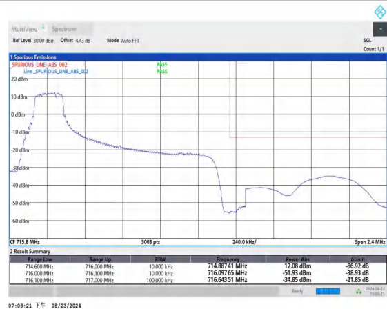
Band12_1.4MHz_QPSK_23173_1RB#0
