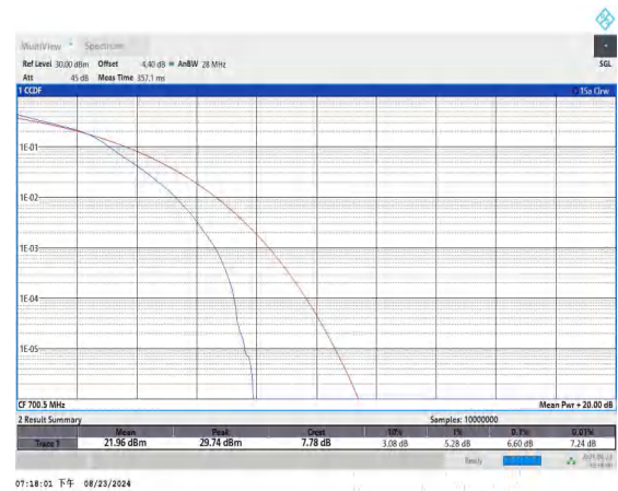
Band12-3MHz-16QAM-23025-15RB#0-PASS
