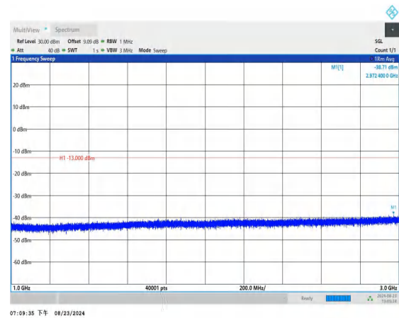
Band12_1.4MHz_QPSK_23173_1RB#0_1000~3000_1000~300
