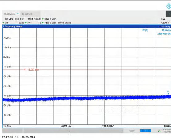
Band12_10MHz_QPSK_23130_1RB#0_1000~3000_1000~3000
