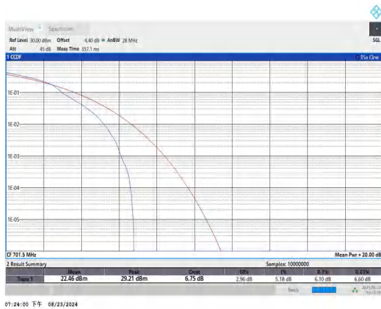
Band12-5MHz-16QAM-23035-1RB#0-PASS
