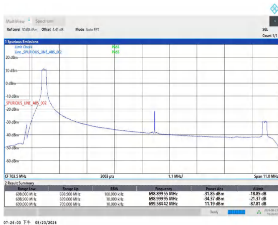
Band12_10MHz_QPSK_23060_1RB#0
