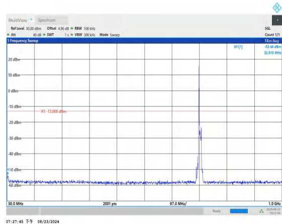
Band12_10MHz_QPSK_23130_1RB#0_30~1000_30~1000
