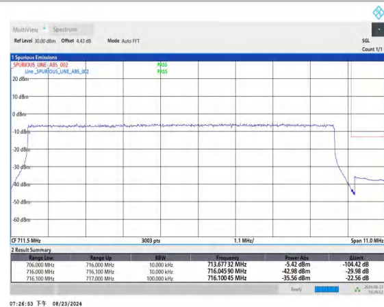
Band12_10MHz_QPSK_23130_50RB#0
