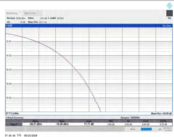
Band12-10MHz-QPSK-23130-50RB#0-PASS
