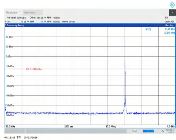
Band12_3MHz_QPSK_23165_1RB#0_30~1000_30~1000
