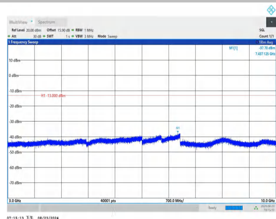
Band12_3MHz_QPSK_23025_1RB#0_3000~10000_3000~1000
