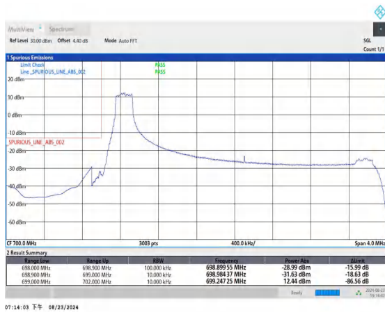
Band12_3MHz_QPSK_23025_1RB#0
