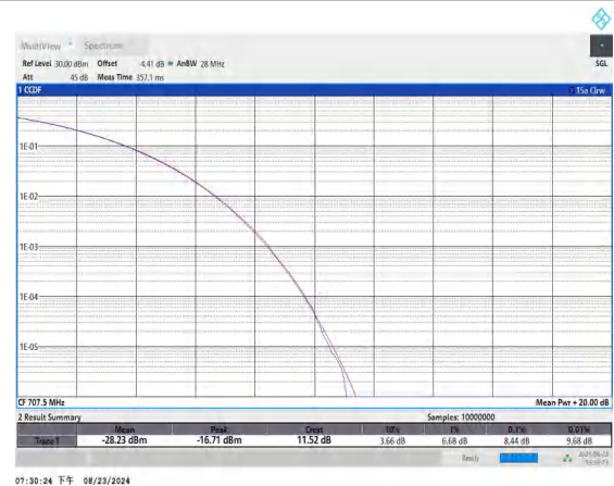
Band12-10MHz-16QAM-23095-50RB#0-PASS
