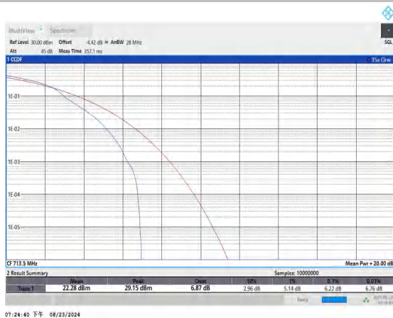
Band12-5MHz-16QAM-23155-1RB#0-PASS
