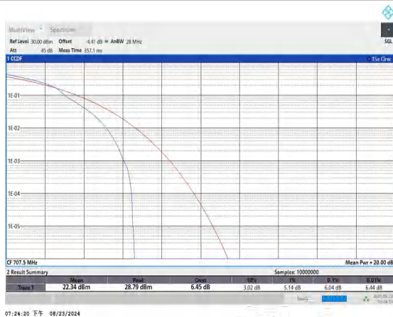
Band12-5MHz-16QAM-23095-1RB#0-PASS
