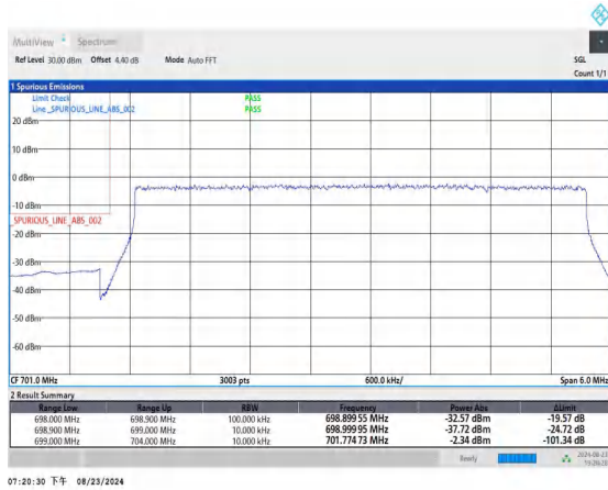
Band12_5MHz_QPSK_23035_25RB#0
