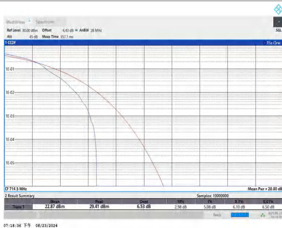
Band12-3MHz-16QAM-23165-1RB#0-PASS
