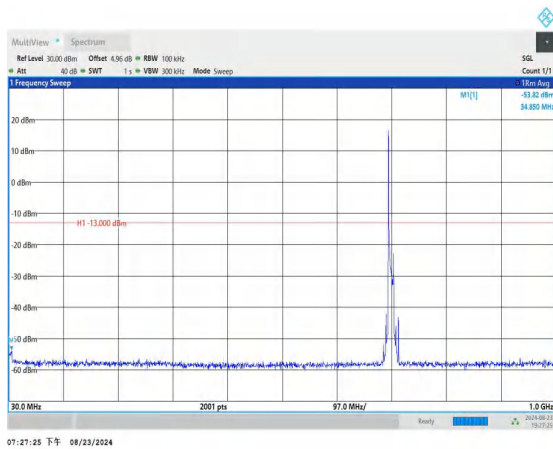
Band12_10MHz_QPSK_23095_1RB#0_30~1000_30~1000
