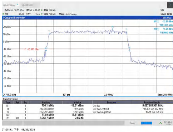
Band12-10MHz-QPSK-23130-50RB#0-PASS
