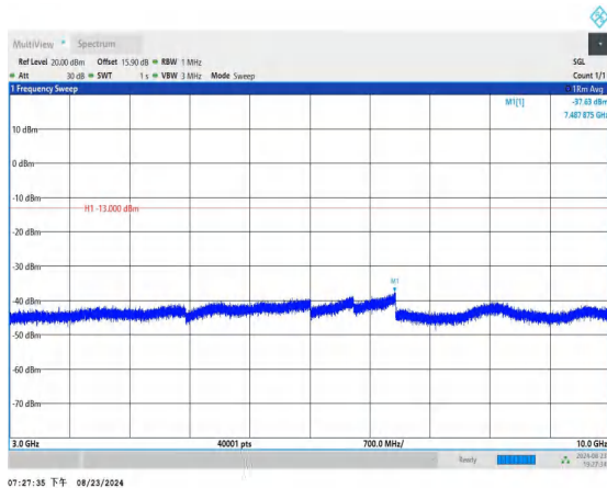
Band12_10MHz_QPSK_23095_1RB#0_3000~10000_3000~10000
