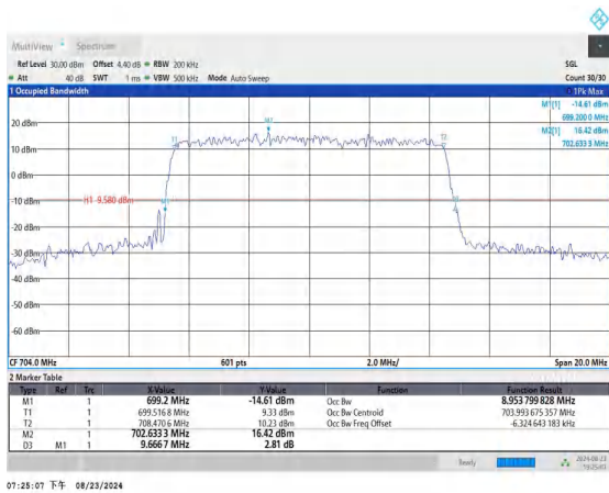
Band12-10MHz-QPSK-23060-50RB#0-PASS
