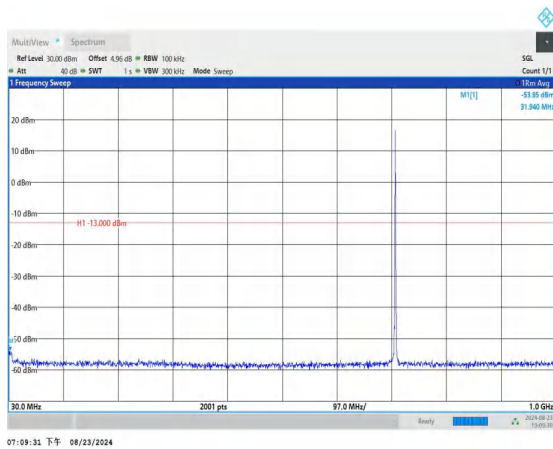
Band12_1.4MHz_QPSK_23173_1RB#0_30~1000_30~1000
