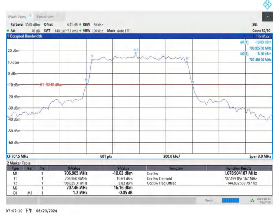
Band12-1.4MHz-QPSK-23095-6RB#0-PASS
