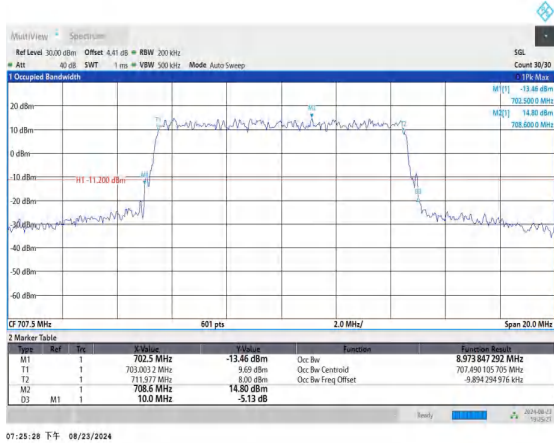
Band12-10MHz-16QAM-23095-50RB#0-PASS
