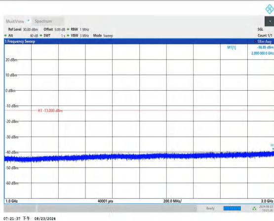
Band12_5MHz_QPSK_23095_1RB#0_1000~3000_1000~3000
