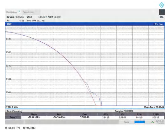
Band12-10MHz-QPSK-23060-50RB#0-PASS
