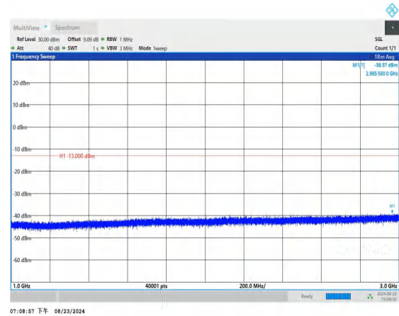
Band12_1.4MHz_QPSK_23017_1RB#0_1000~3000_1000~300
