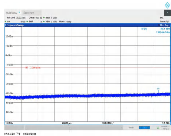
Band12_3MHz_QPSK_23095_1RB#0_1000~3000_1000~3000
