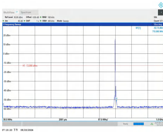
Band12_3MHz_QPSK_23095_1RB#0_30~1000_30~1000
