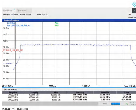
Band12_10MHz_QPSK_23060_50RB#0
