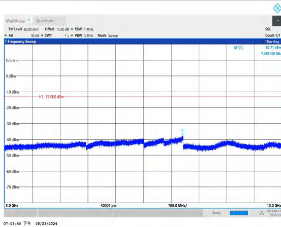
Band12_1.4MHz_QPSK_23173_1RB#0_3000~10000_3000~10
