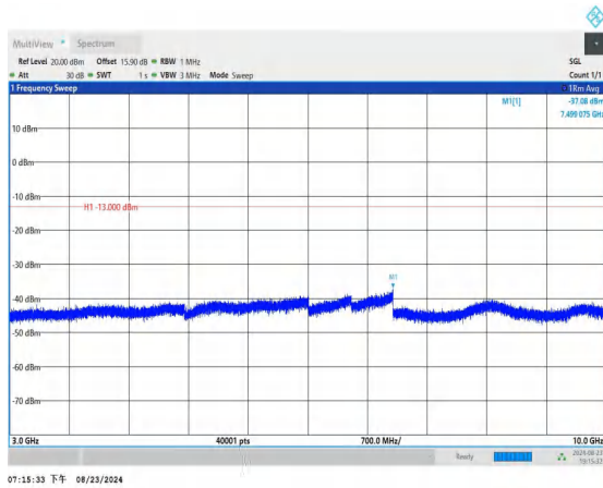
Band12_3MHz_QPSK_23095_1RB#0_3000~10000_3000~1000
