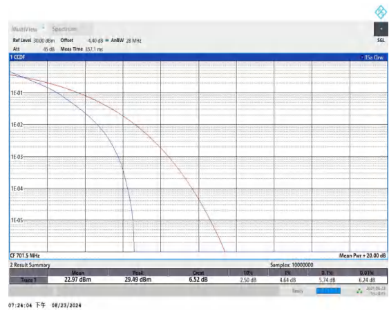
Band12-5MHz-QPSK-23035-25RB#0-PASS
