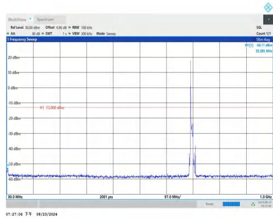
Band12_10MHz_QPSK_23060_1RB#0_30~1000_30~1000
