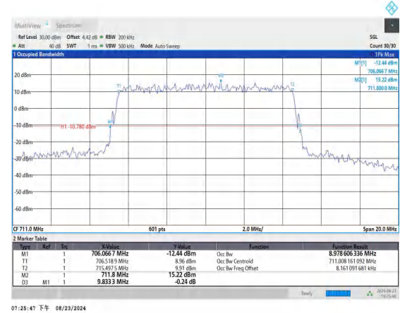
Band12-10MHz-16QAM-23130-50RB#0-PASS
