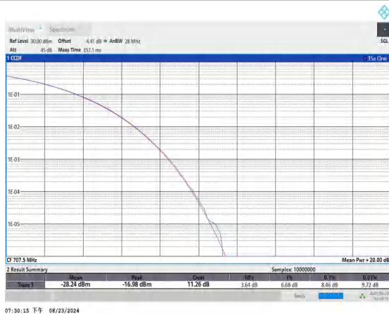
Band12-10MHz-16QAM-23095-1RB#0-PASS
