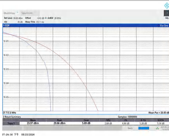
Band12-5MHz-QPSK-23155-1RB#0-PASS
