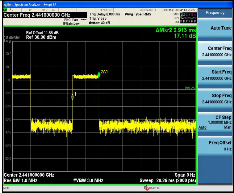
3DH5-Ant1-Hop-PASS
