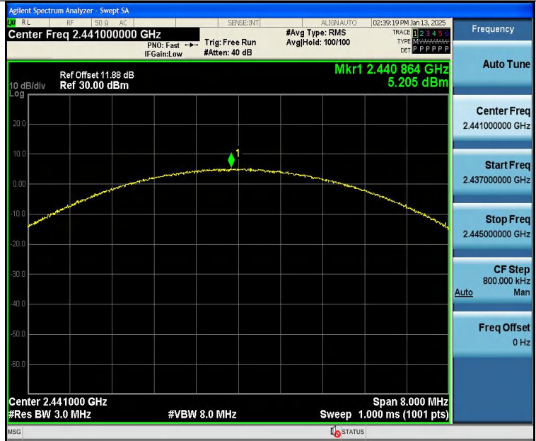
3DH5-Ant1-2441-PASS
