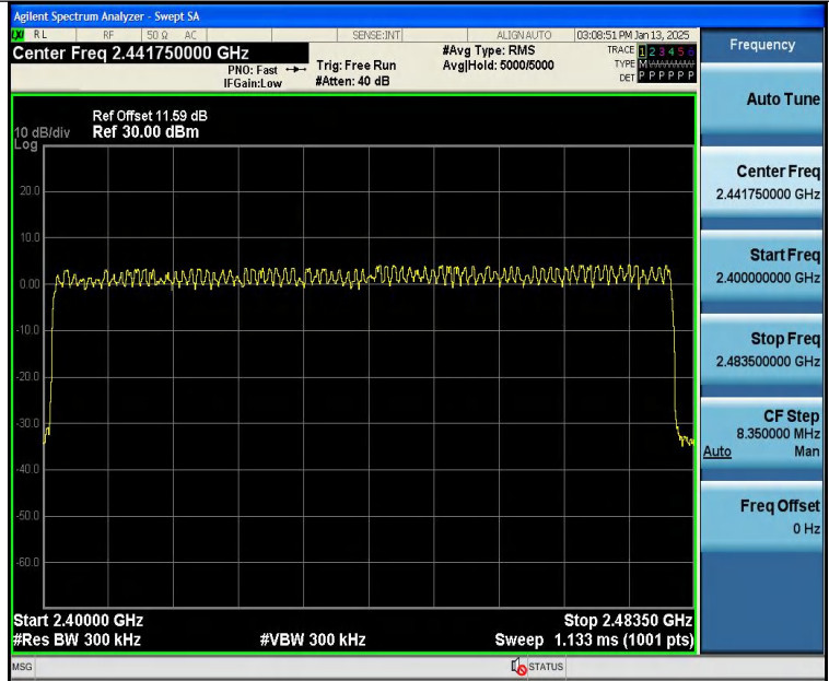
2DH5-Ant1-Hop-PASS
