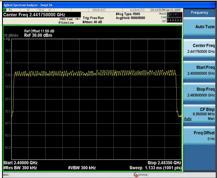
3DH5-Ant1-Hop-PASS
