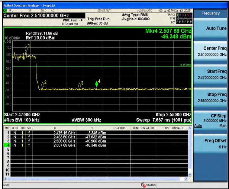
2DH5-Ant1-Hop_2480-PASS
