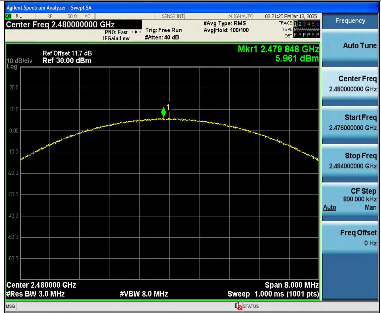
3DH5-Ant1-2480-PASS
