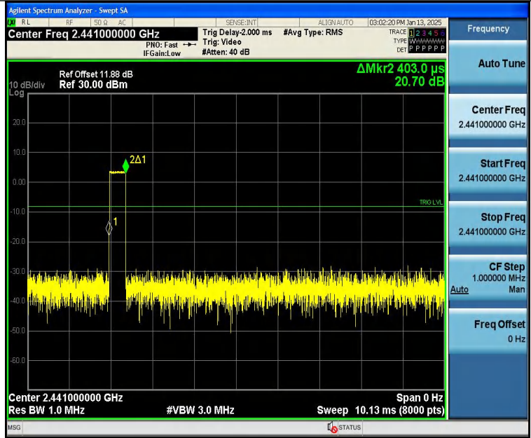
DH1-Ant1-Hop-PASS
