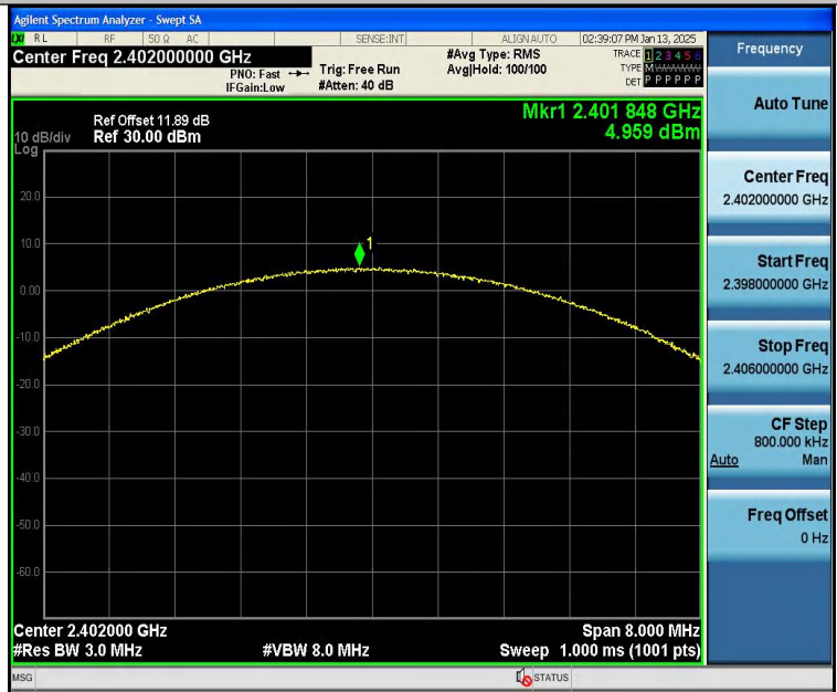
3DH5-Ant1-2402-PASS
