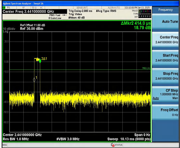
2DH1-Ant1-Hop-PASS
