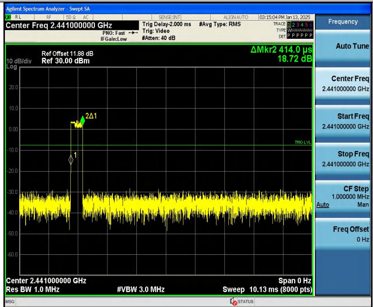
3DH1-Ant1-Hop-PASS
