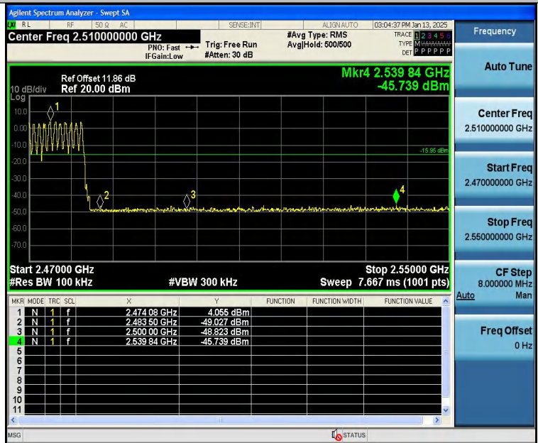
DH5-Ant1-Hop_2480-PASS
