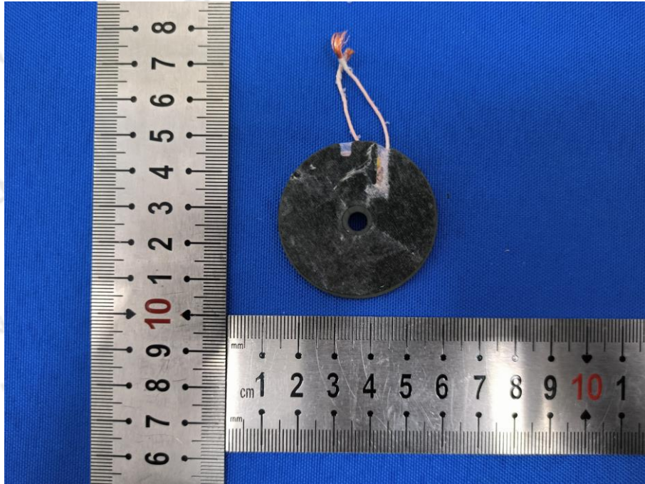
Coil Antenna-Watch
