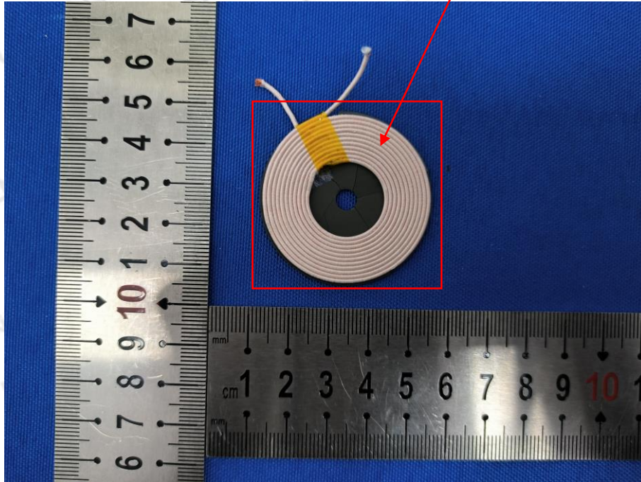
Coil Antenna-Phone
