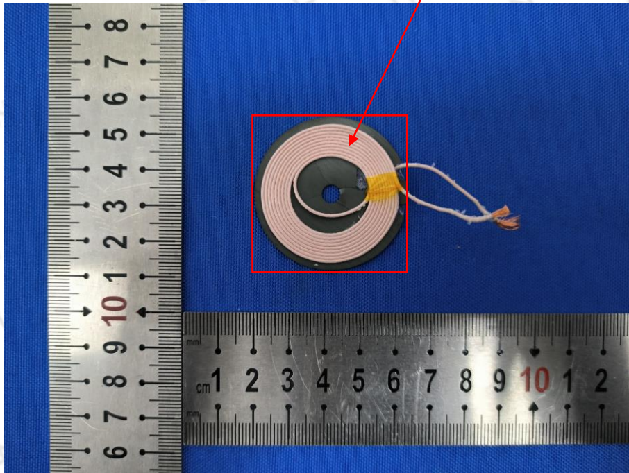
Coil Antenna-Earphone
