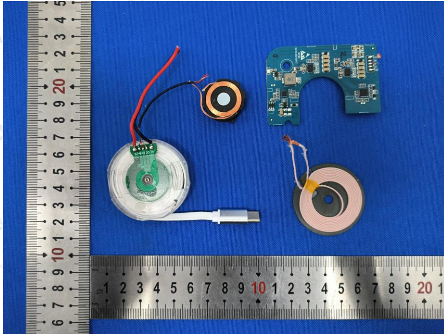
Coil Antenna-Earphone
