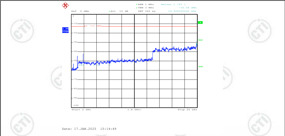
Band2-15MHz-16QAM-18675-1RB#0-Range3:2000~20000MHz
