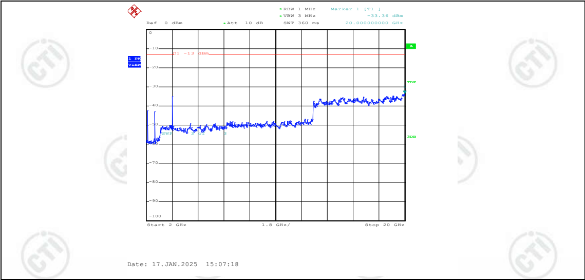
Band2-1.4MHz-16QAM-19193-1RB#0-Range3:2000~20000MHz
