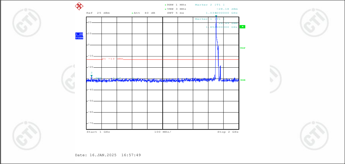
Band2-15MHz-QPSK-18675-1RB#0-Range2:1000~2000MHz
