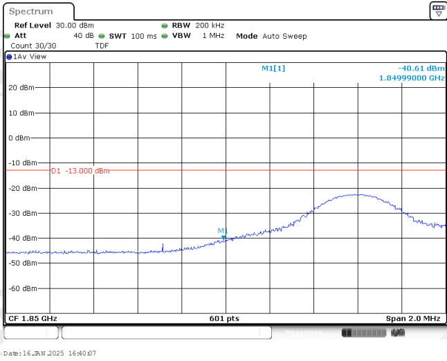
Band2-10MHz-QPSK-18650-1RB#49
