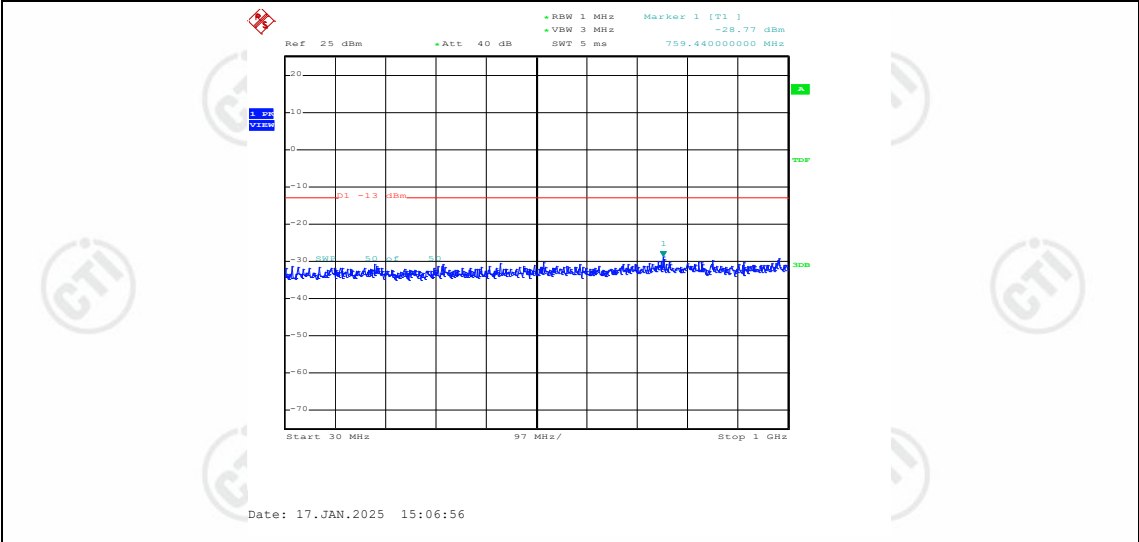
Band2-1.4MHz-16QAM-19193-1RB#0-Range1:30~1000MHz
