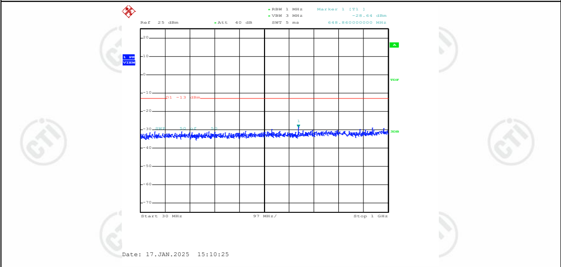
Band2-5MHz-16QAM-18625-1RB#0-Range1:30~1000MHz
