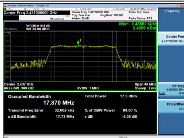
11N20SISO-Ant1-2437
