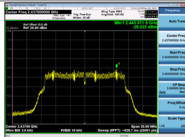
11G-Ant1-2437-PASS
