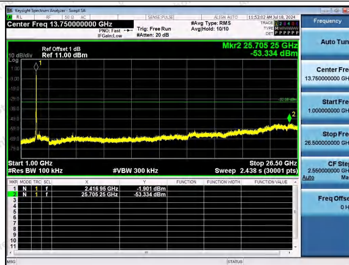
11N40MIMO-Ant1-2422-1000~26500-PASS
