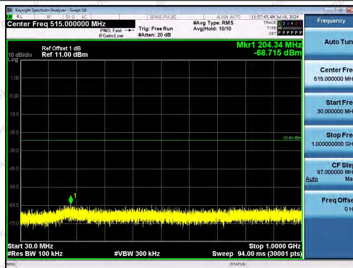
11N40MIMO-Ant1-2437-30~1000-PASS
