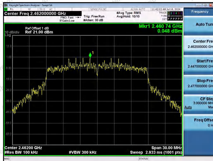
11N20MIMO-Ant1-2462-0~Reference-PASS
