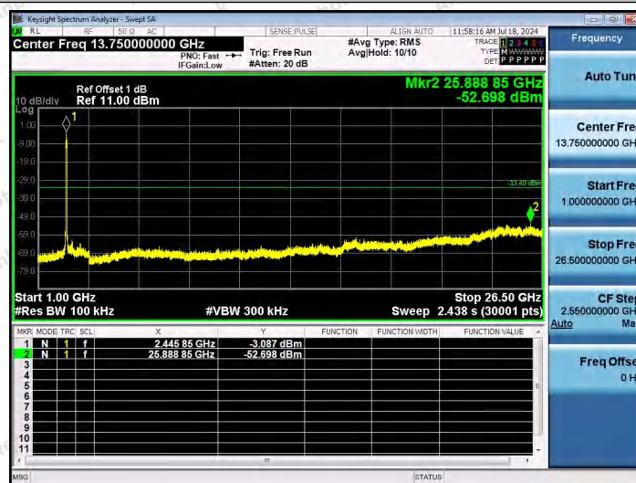
11N40MIMO-Ant1-2437-1000~26500-PASS
