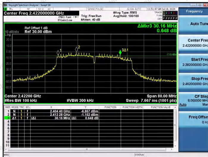
11N40MIMO-Ant1-2422-PASS
