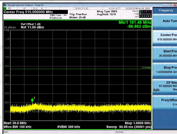
11N40MIMO-Ant1-2422-30~1000-PASS
