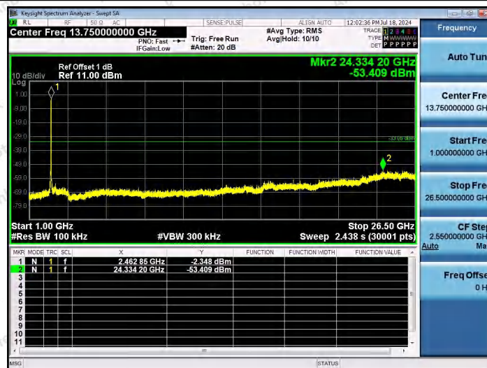
11N40MIMO-Ant1-2452-1000~26500-PASS
