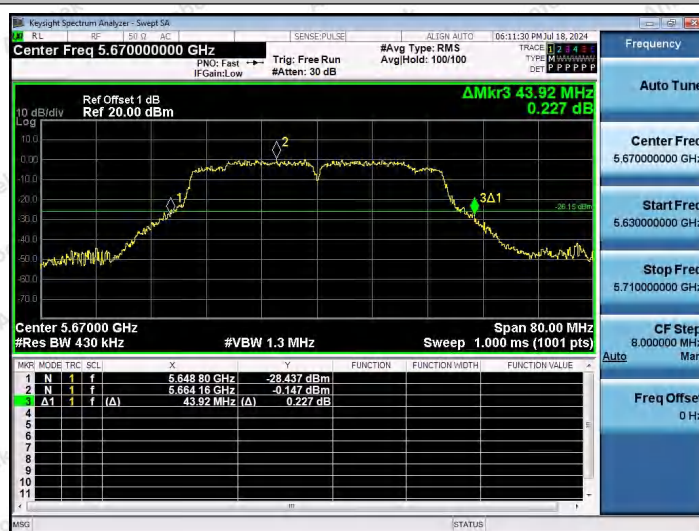
11AC40SISO-Ant1-5670
