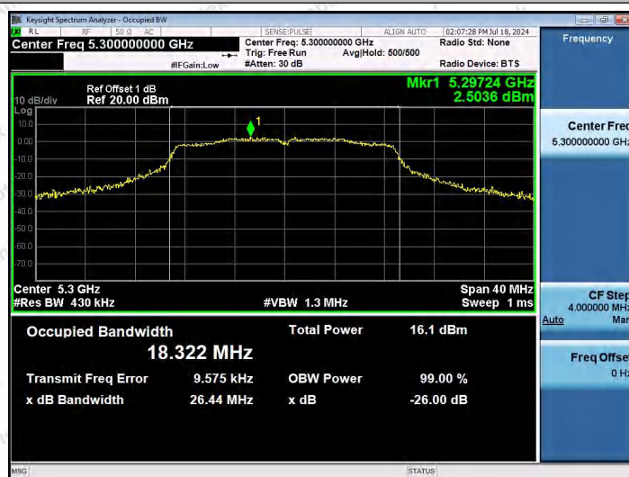
11AC20SISO-Ant1-5300
