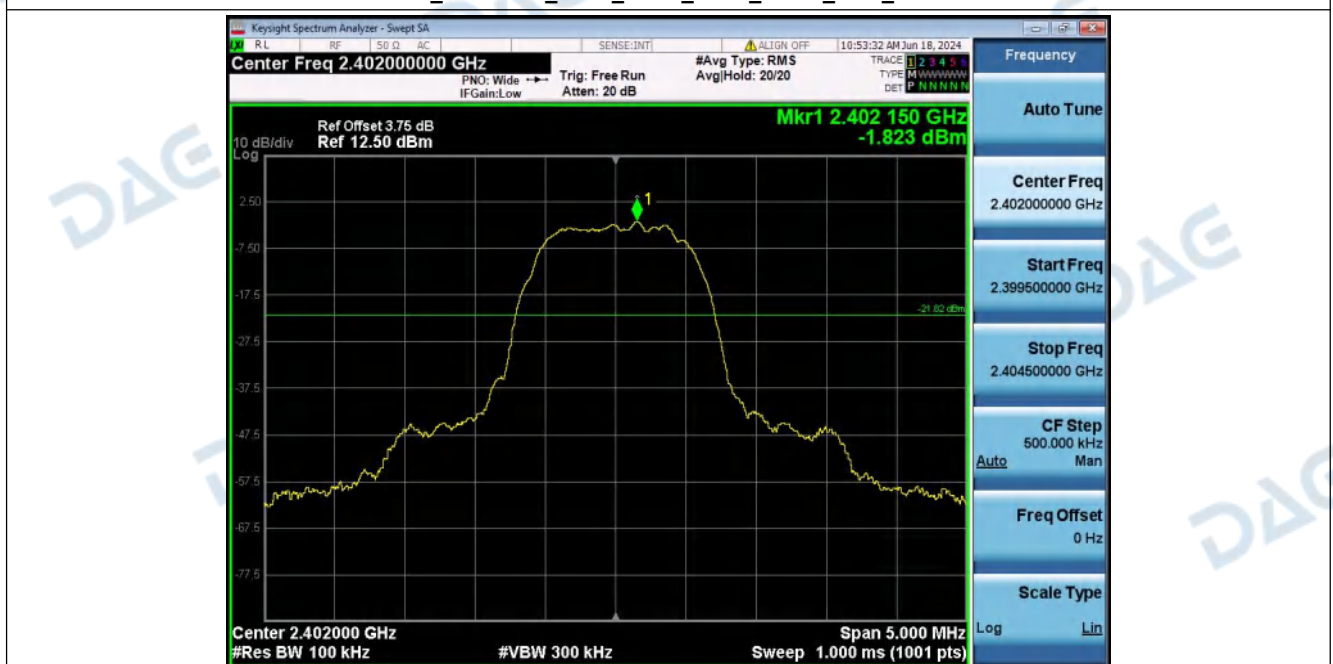
2_Spurious_Emissions_NVNT_ANT1_3-DH5_2402_00
