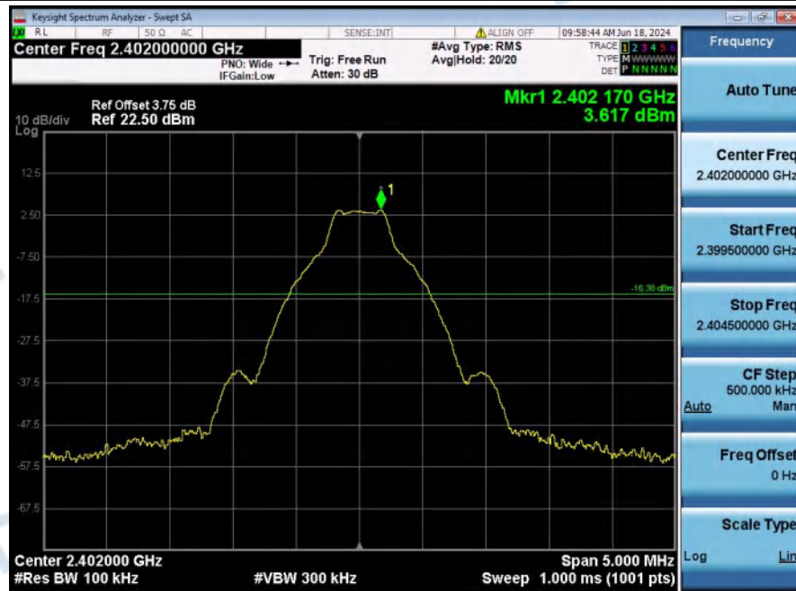
2_Bandedge_NVNT_ANT1_1-DH5_2402_00
