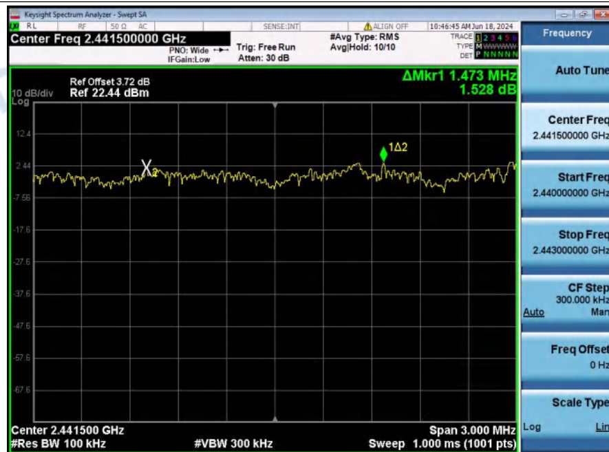
Carrier_Frequencies_Separation_(Hopping)_NVNT_ANT1_2-DH5_Hopping
