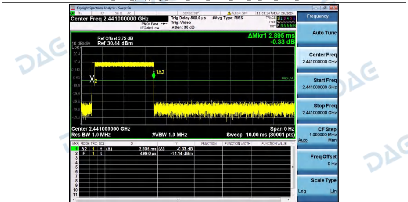
Dwell_Time_(Hopping)_NVNT_ANT1_3-DH5_2441_00_Accumulated
