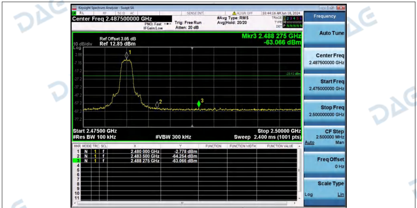
1_Reference_Level_Hopping_NVNT_ANT1_2-DH5_Hopping
