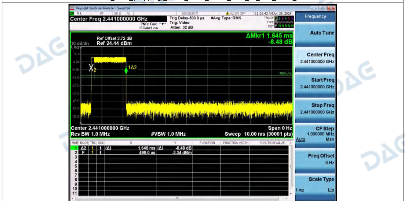
Dwell_Time_(Hopping)_NVNT_ANT1_2-DH3_2441_00_Accumulated
