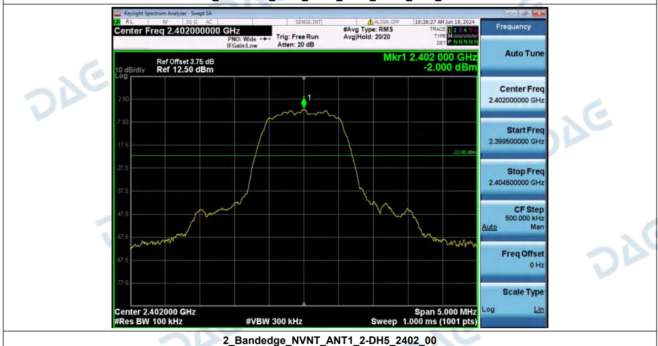
1_Reference_Level_NVNT_ANT1_2-DH5_2402_00
