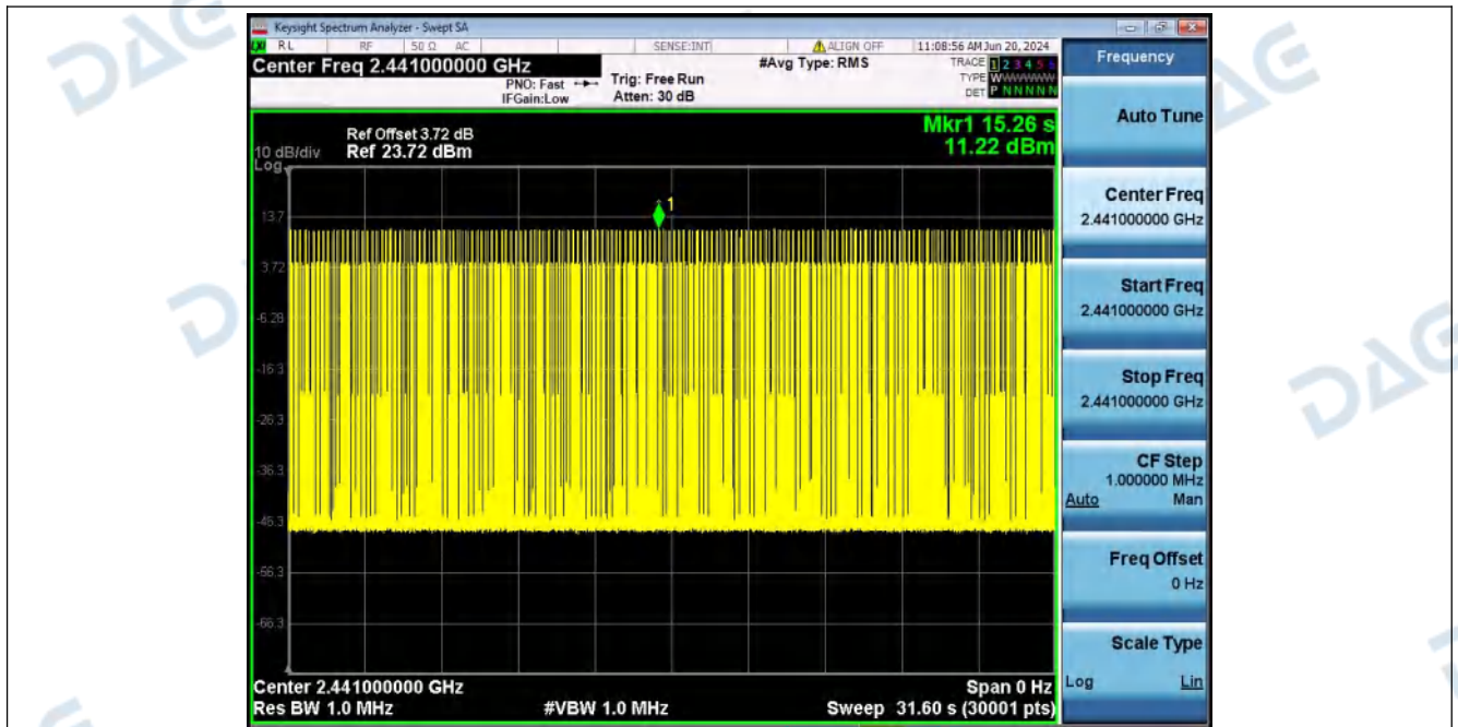
Dwell_Time_(Hopping)_NVNT_ANT1_3-DH3_2441_00_One_Burst_Time
