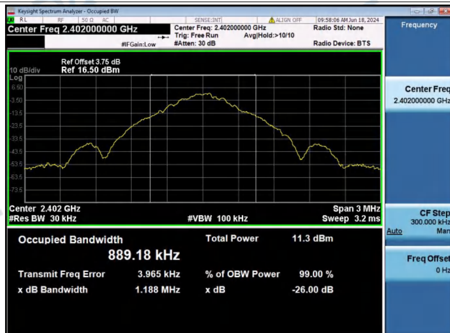
99%_Occupied_Bandwidth_NVNT_ANT1_1-DH5_2402_00
