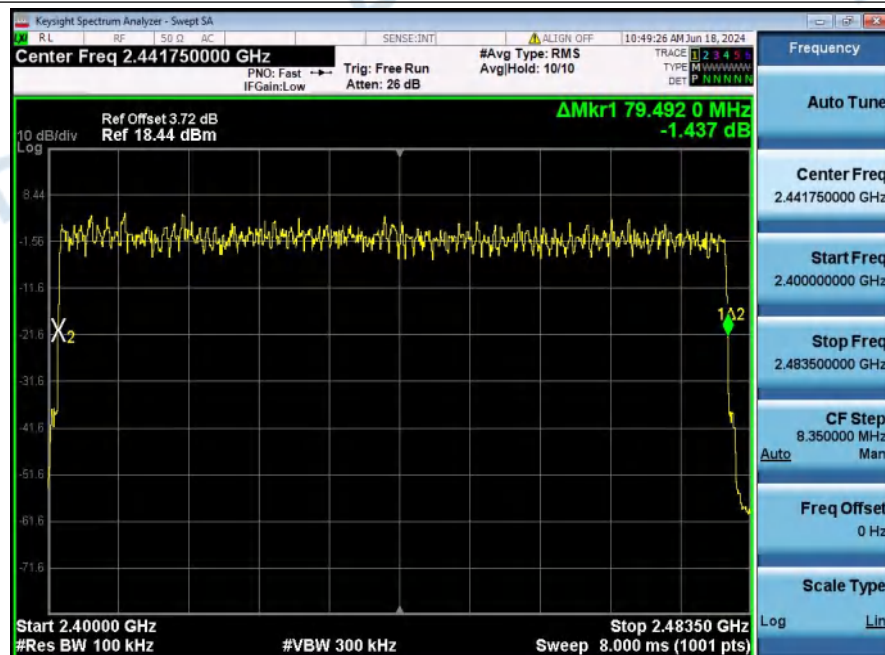
Number_of_Hopping_Channel_(Hopping)_NVNT_ANT1_2-DH5_Hopping
