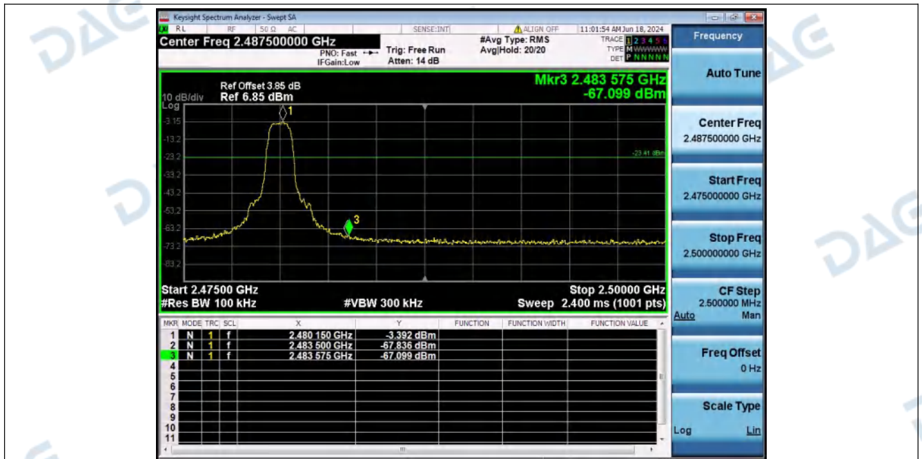
1_Reference_Level_Hopping_NVNT_ANT1_3-DH5_Hopping
