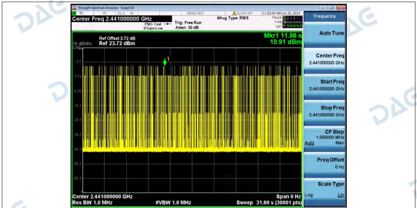
Dwell_Time_(Hopping)_NVNT_ANT1_1-DH1_2441_00_One_Burst_Time
