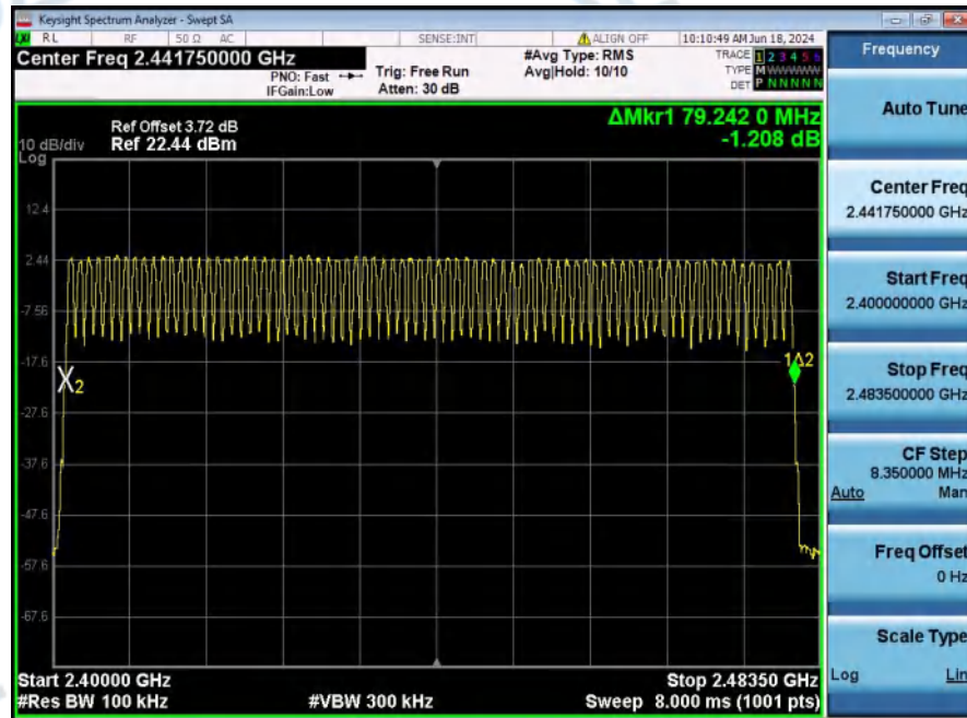
Number_of_Hopping_Channel_(Hopping)_NVNT_ANT1_1-DH5_Hopping
