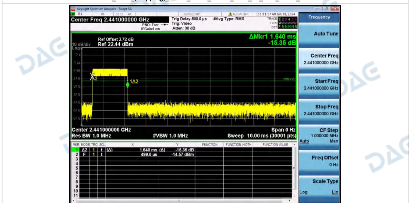
Dwell_Time_(Hopping)_NVNT_ANT1_1-DH3_2441_00_Accumulated
