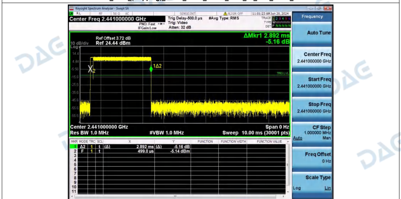
Dwell_Time_(Hopping)_NVNT_ANT1_2-DH5_2441_00_Accumulated
