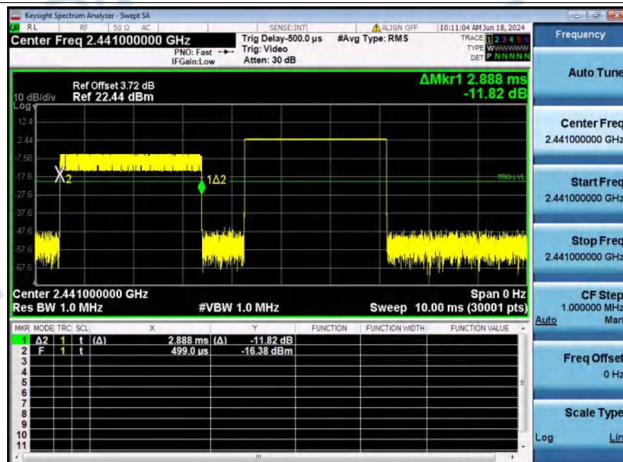
Dwell_Time_(Hopping)_NVNT_ANT1_1-DH5_2441_00_Accumulated
