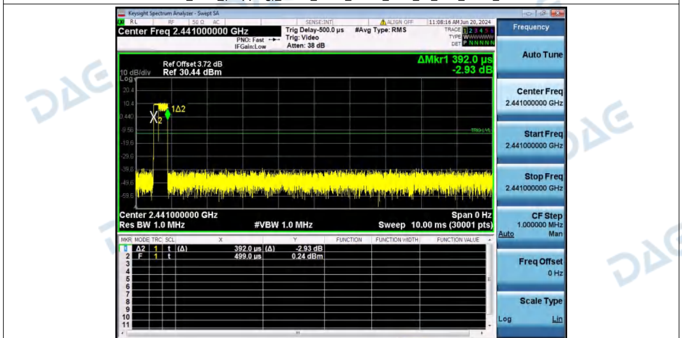
Dwell_Time_(Hopping)_NVNT_ANT1_3-DH1_2441_00_Accumulated
