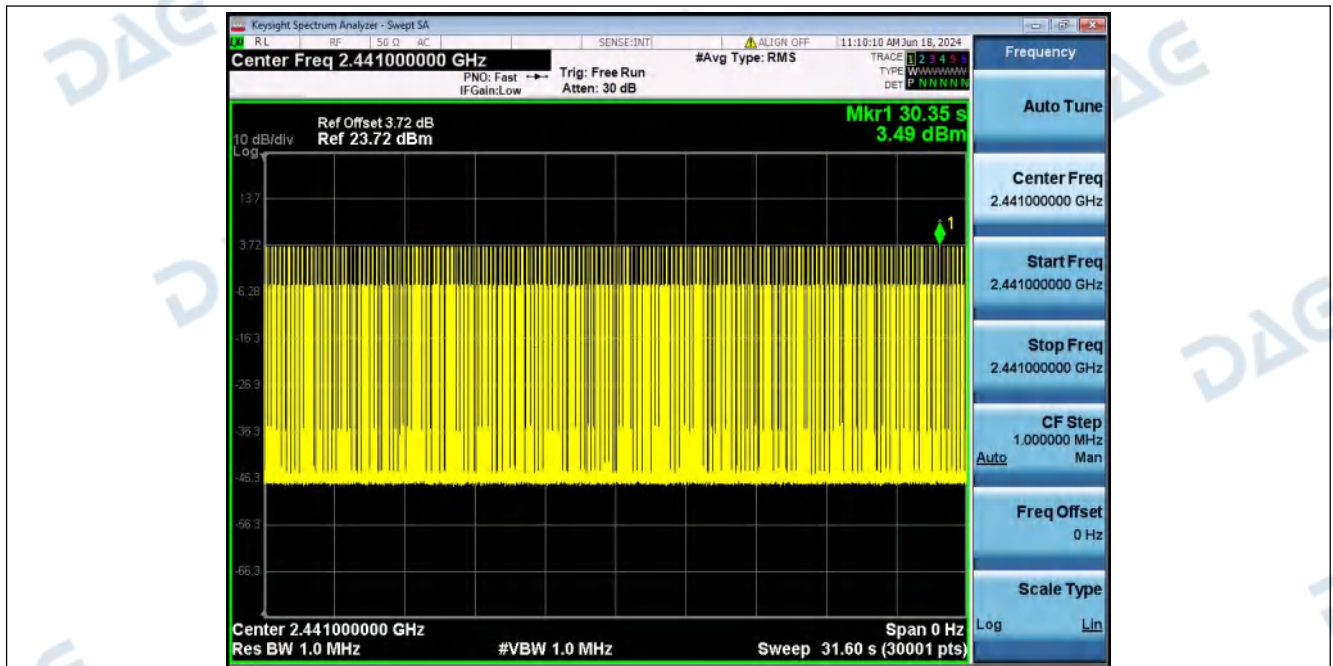
Dwell_Time_(Hopping)_NVNT_ANT1_1-DH3_2441_00_One_Burst_Time
