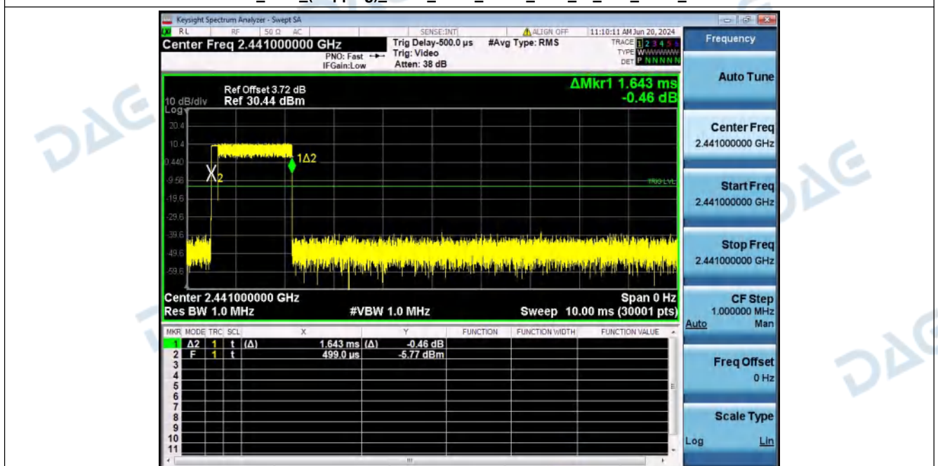
Dwell_Time_(Hopping)_NVNT_ANT1_3-DH3_2441_00_Accumulated
