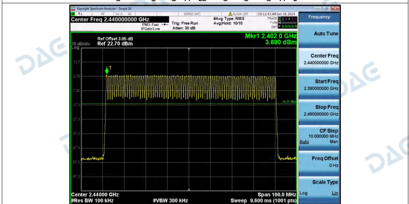
2_Band_Edge_(Hopping)_NVNT_ANT1_1-DH5_Hopping
