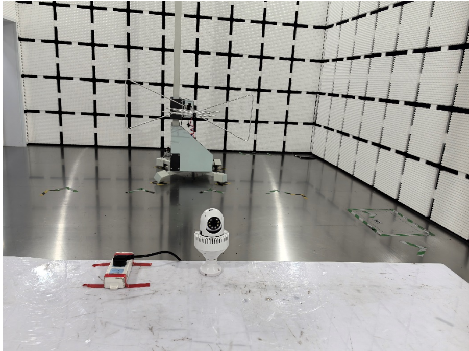
Radiated Emission
