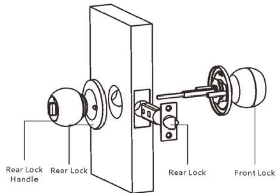
Door Lock Installation Diagram
