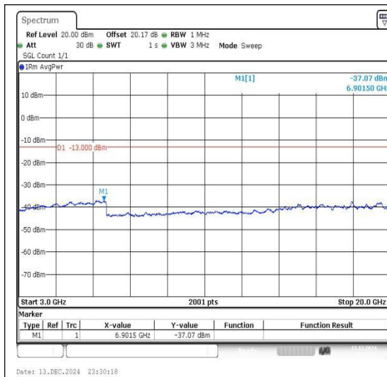
Band4_20MHz_QPSK_20050_1RB#0_3000~20000_3000~20000
