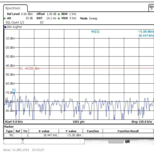
Band4_20MHz_16QAM_20050_1RB#0_0.009~0.15_0.009~0.15
