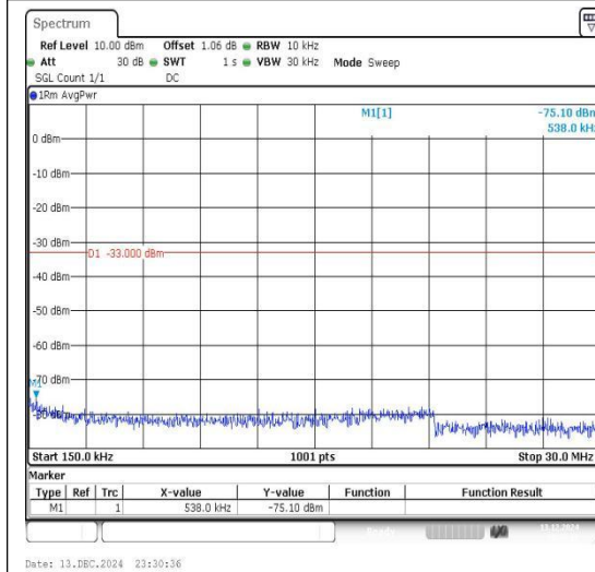
Band4_20MHz_QPSK_20050_1RB#0_3000~20000_0.15~30
