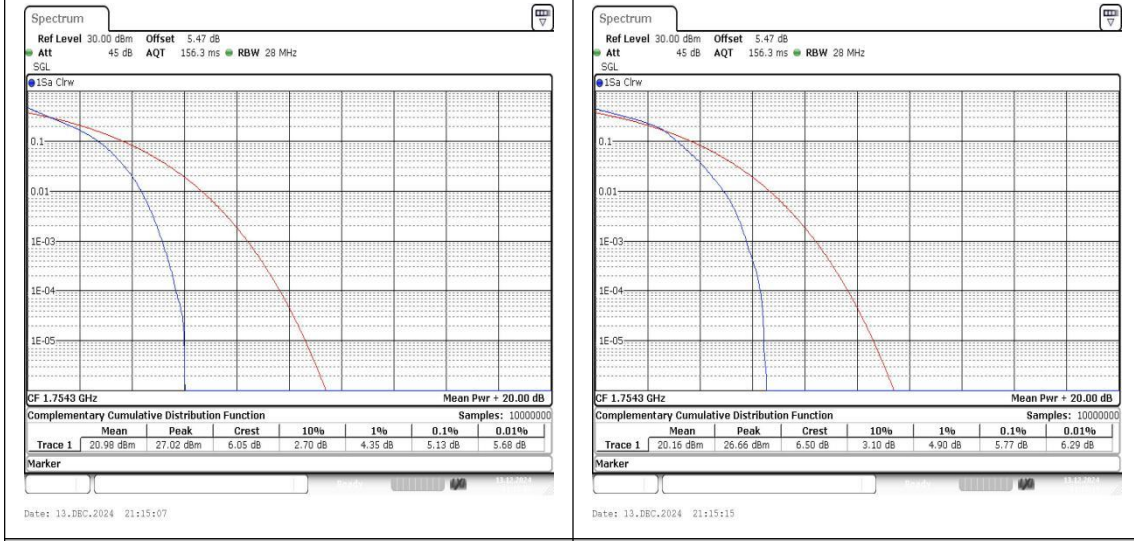
Band4-1.4MHz-QPSK-20393-6RB#0-PASS Band4-1.4MHz-16QAM-20393-6RB#0-PASS
