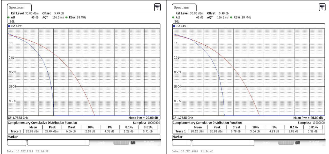
Band4-3MHz-QPSK-20385-15RB#0-PASS Band4-3MHz-16QAM-20385-15RB#0-PASS
