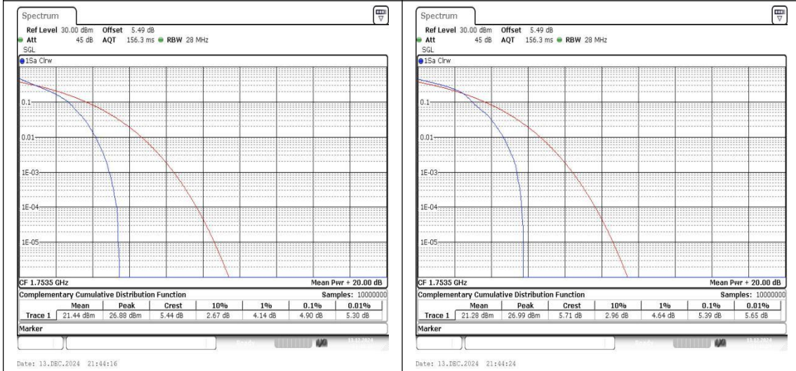
Band4-3MHz-QPSK-20385-1RB#0-PASS Band4-3MHz-16QAM-20385-1RB#0-PASS
