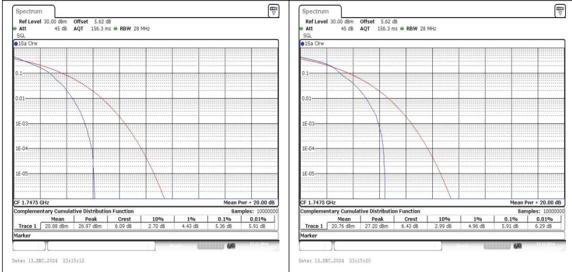
Band4-15MHz-QPSK-20325-1RB#0-PASS Band4-15MHz-16QAM-20325-1RB#0-PASS
