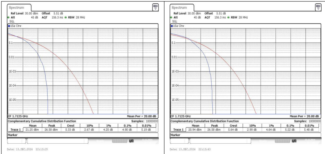
Band4-5MHz-QPSK-19975-1RB#0-PASS Band4-5MHz-16QAM-19975-1RB#0-PASS
