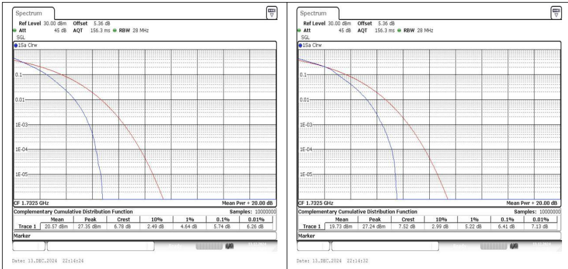
Band4-5MHz-QPSK-20175-25RB#0-PASS Band4-5MHz-16QAM-20175-25RB#0-PASS
