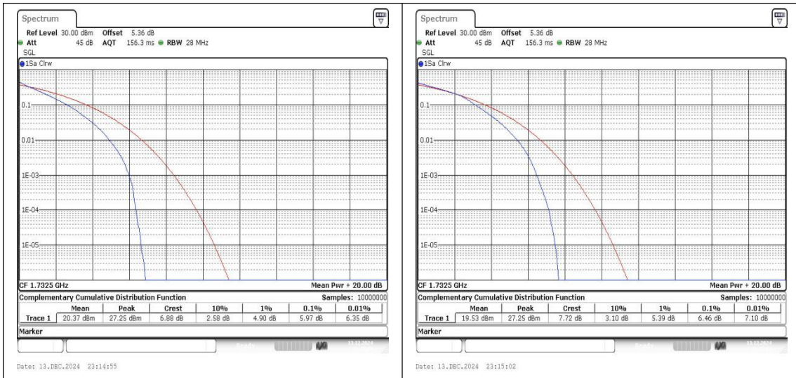
Band4-15MHz-QPSK-20175-75RB#0-PASS Band4-15MHz-16QAM-20175-75RB#0-PASS
