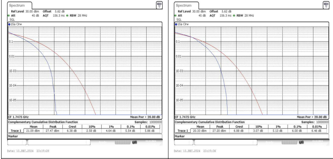
Band4-15MHz-QPSK-20325-75RB#0-PASS Band4-15MHz-16QAM-20325-75RB#0-PASS
