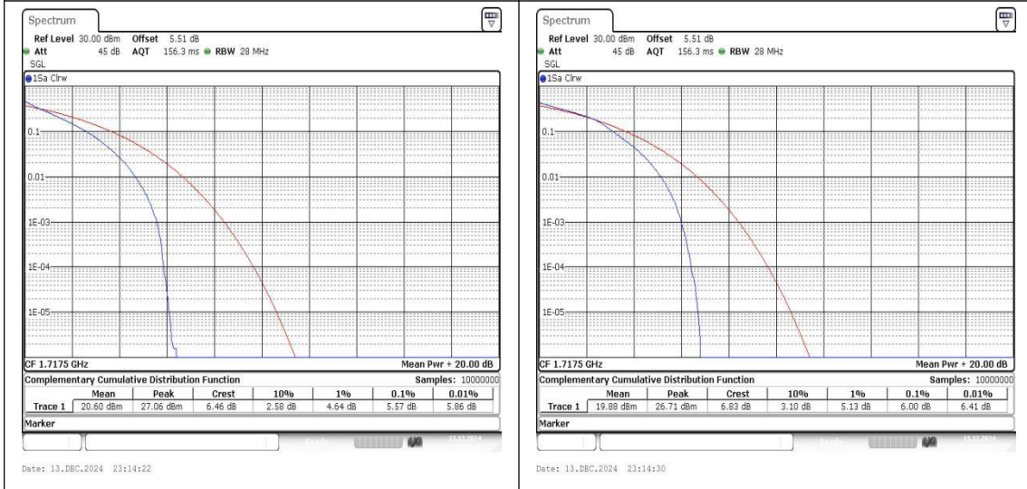
Band4-15MHz-QPSK-20025-75RB#0-PASS Band4-15MHz-16QAM-20025-75RB#0-PASS
