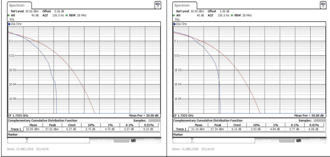
Band4-5MHz-QPSK-20175-1RB#0-PASS Band4-5MHz-16QAM-20175-1RB#0-PASS
