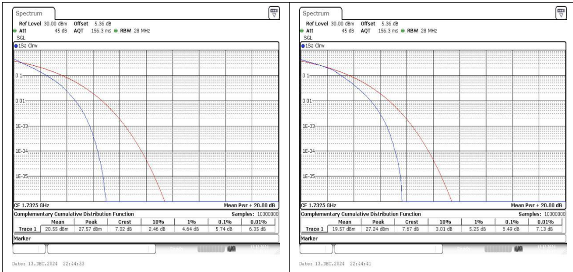
Band4-10MHz-QPSK-20175-50RB#0-PASS Band4-10MHz-16QAM-20175-50RB#0-PASS
