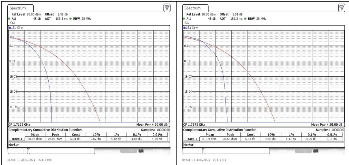
Band4-15MHz-QPSK-20025-1RB#0-PASS Band4-15MHz-16QAM-20025-1RB#0-PASS
