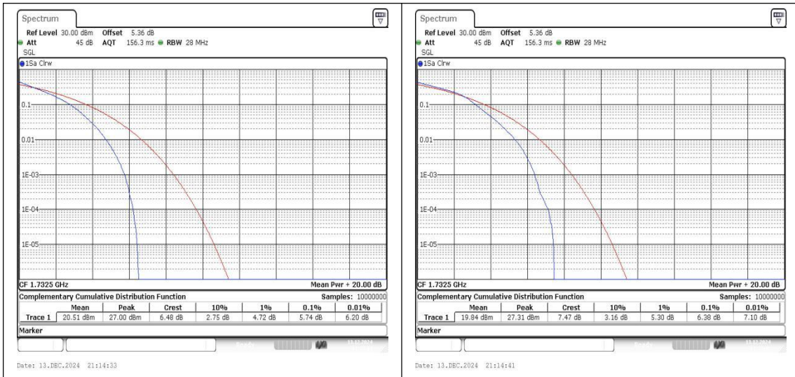
Band4-1.4MHz-QPSK-20175-6RB#0-PASS Band4-1.4MHz-16QAM-20175-6RB#0-PASS
