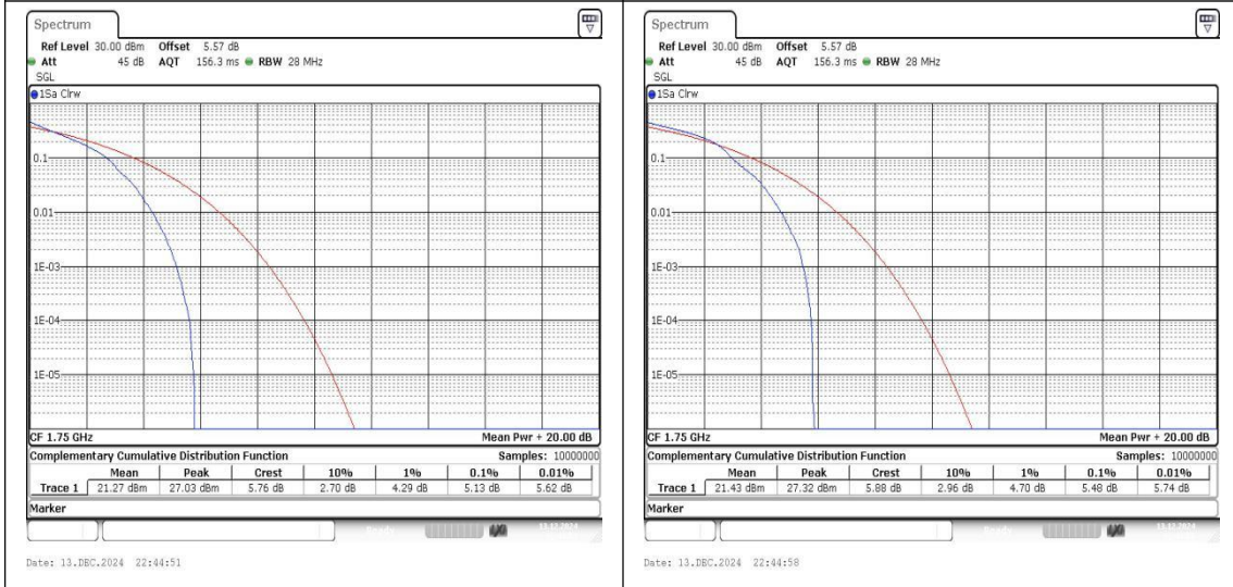
Band4-10MHz-QPSK-20350-1RB#0-PASS Band4-10MHz-16QAM-20350-1RB#0-PASS
