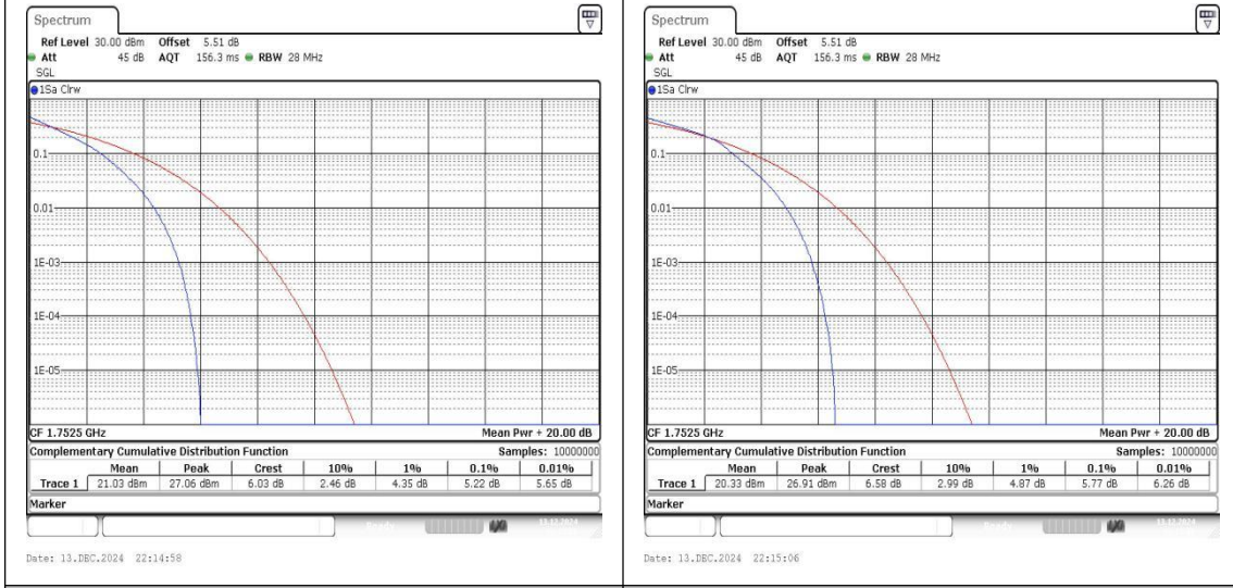
Band4-5MHz-QPSK-20375-25RB#0-PASS Band4-5MHz-16QAM-20375-25RB#0-PASS
