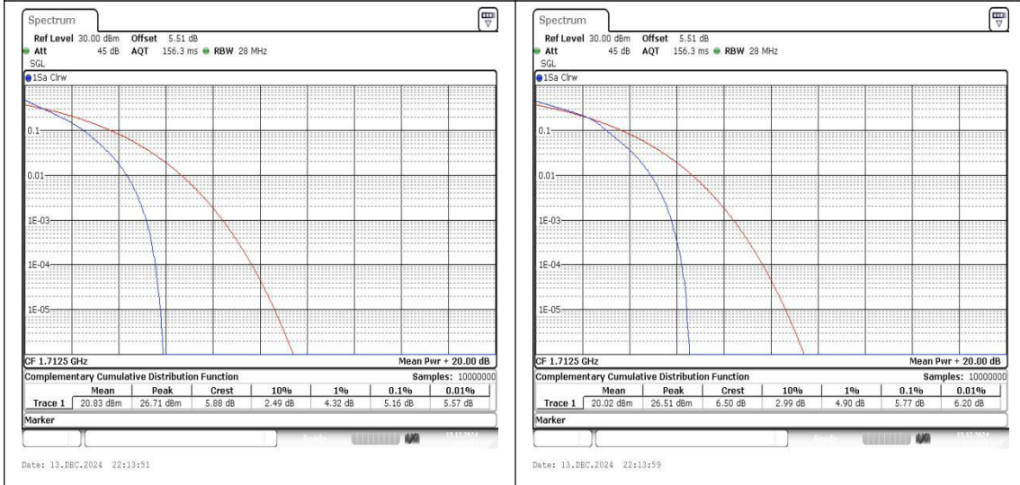
Band4-5MHz-QPSK-19975-25RB#0-PASS Band4-5MHz-16QAM-19975-25RB#0-PASS
