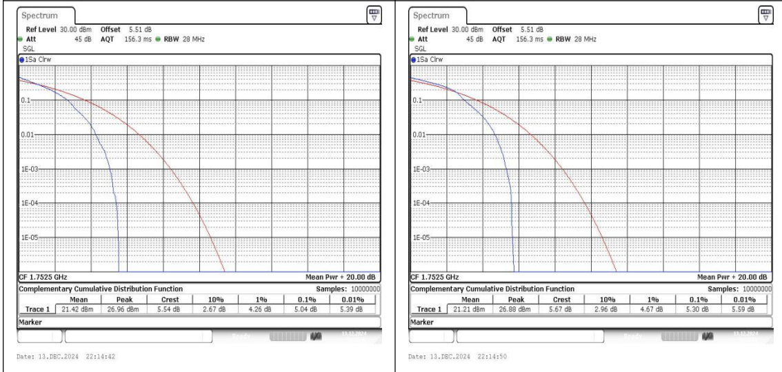
Band4-5MHz-QPSK-20375-1RB#0-PASS Band4-5MHz-16QAM-20375-1RB#0-PASS
