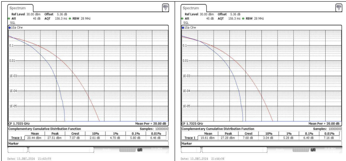
Band4-3MHz-QPSK-20175-15RB#0-PASS Band4-3MHz-16QAM-20175-15RB#0-PASS
