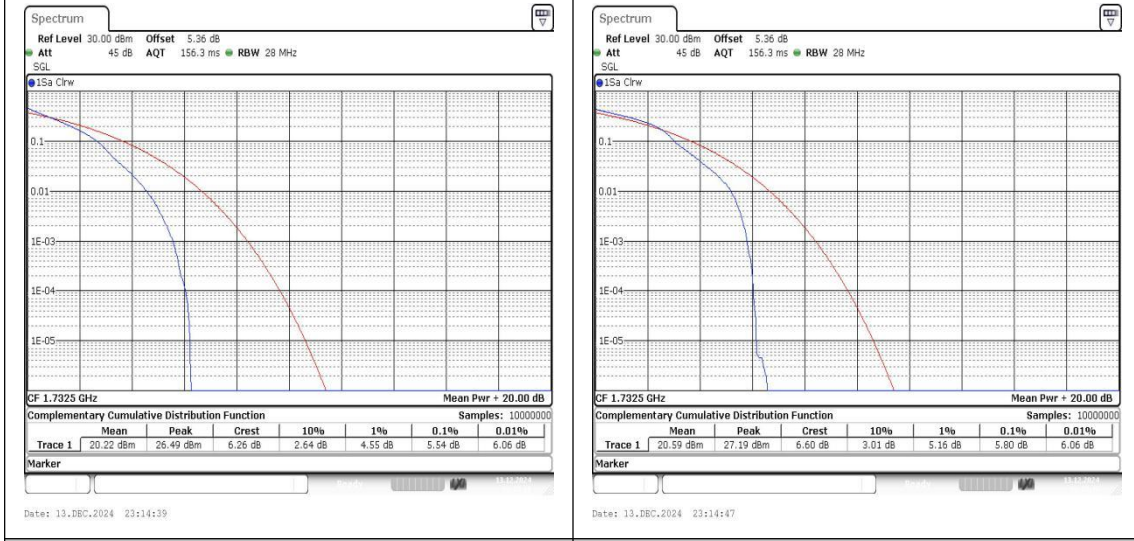
Band4-15MHz-QPSK-20175-1RB#0-PASS Band4-15MHz-16QAM-20175-1RB#0-PASS
