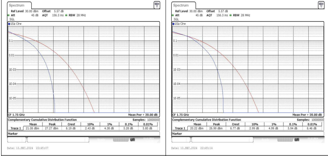
Band4-10MHz-QPSK-20350-50RB#0-PASS Band4-10MHz-16QAM-20350-50RB#0-PASS
