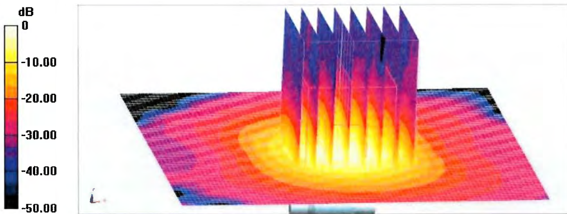
0 dB = 19.6 W/kg = 12.92 dBW/kg
