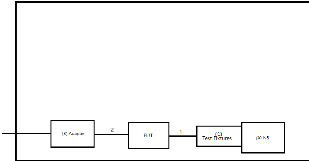
Radiated Emissions
