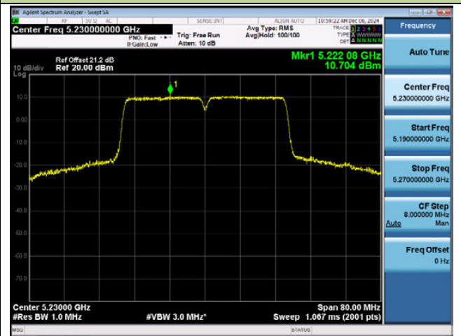
Channel 46 (5230MHz)
