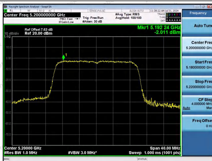
11AX20MIMO-Ant2-5200-PASS
