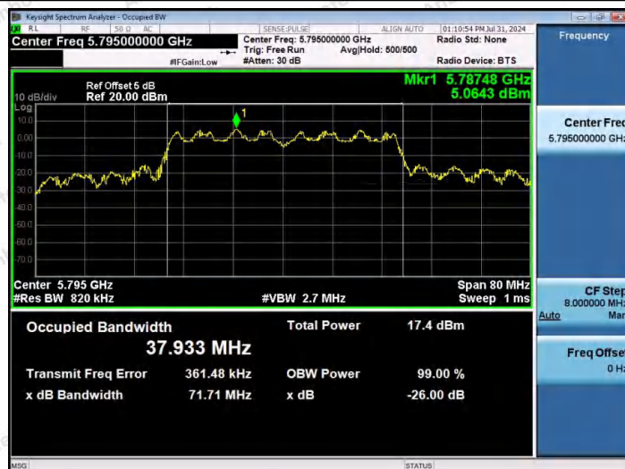
11AC40MIMO-Ant2-5795
