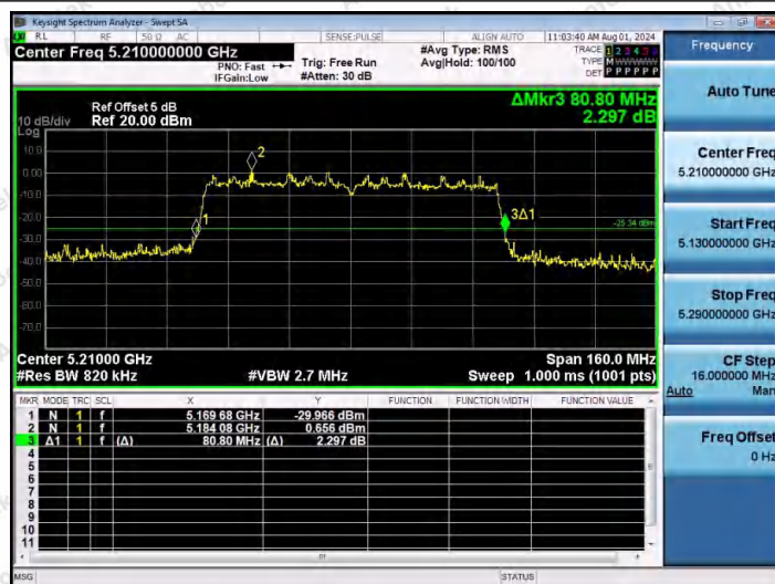
11AC80MIMO-Ant1-51210
