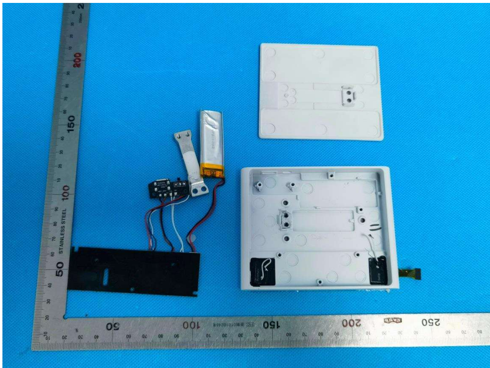
Model: AKU-MINI-WHT OPEN VIEW OF EUT (FIGURE 1)
