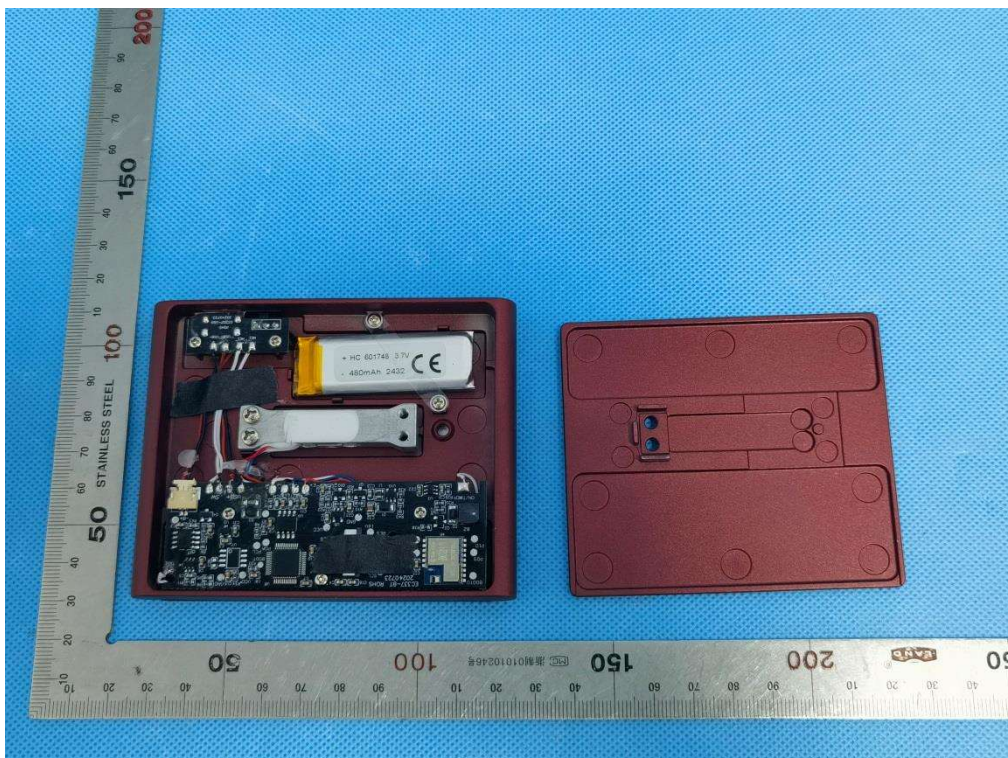
Model: AKU-MINI-RED OPEN VIEW OF EUT (FIGURE 1)
