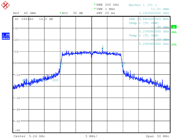
802.11ax20_5240MHz_RU_Full 19.880MHz
