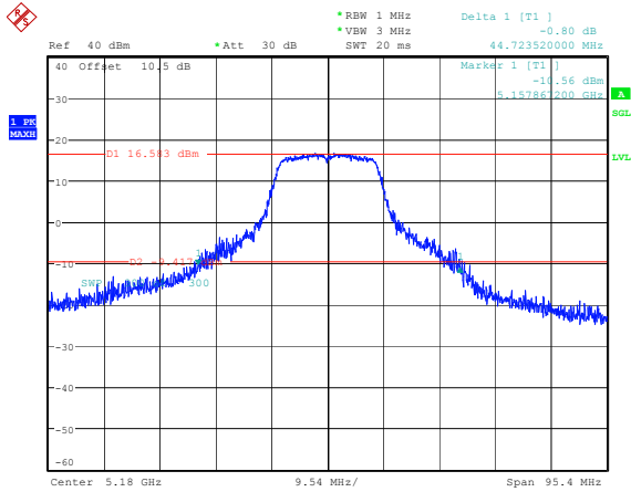
802.11n20_5180MHz 44.724MHz
