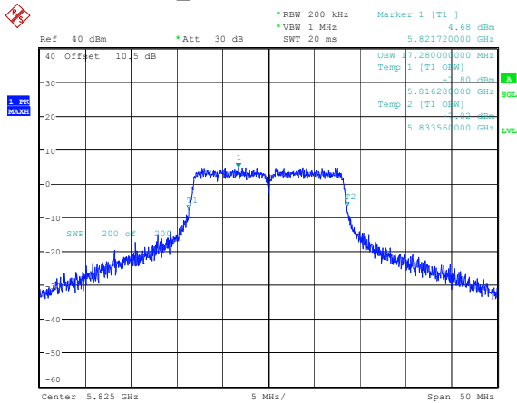
802.11a_5825MHz 17.280MHz
