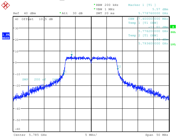
802.11a_5785MHz 17.400MHz
