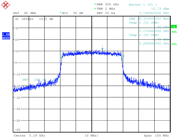
802.11ax40_5190MHz_RU_Full 38.320MHz
