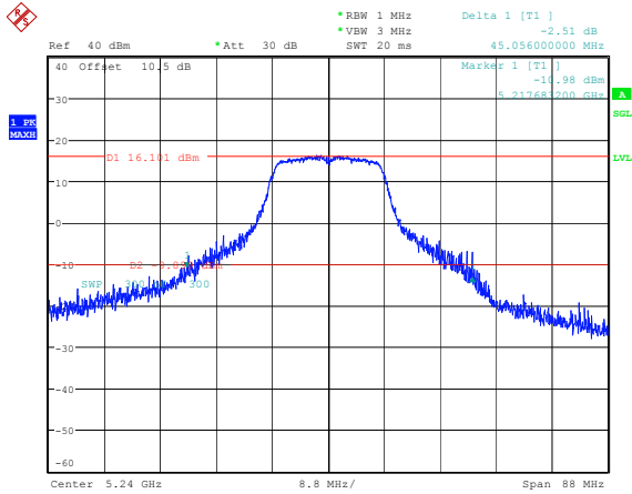
802.11n20_5240MHz 45.056MHz
