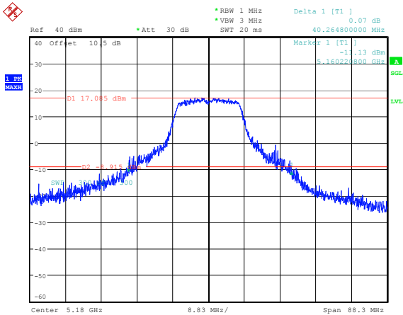
802.11a_5180MHz 40.265MHz
