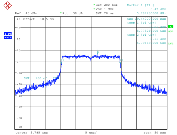
802.11ax20_5785MHz_RU_Full 19.440MHz
