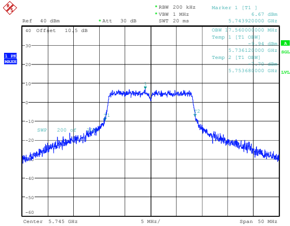
802.11a_5745MHz 17.560MHz
