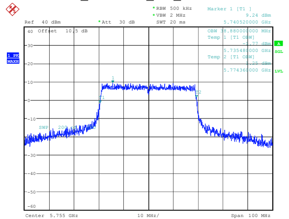
802.11ax40_5755MHz_RU_Full 38.880MHz
