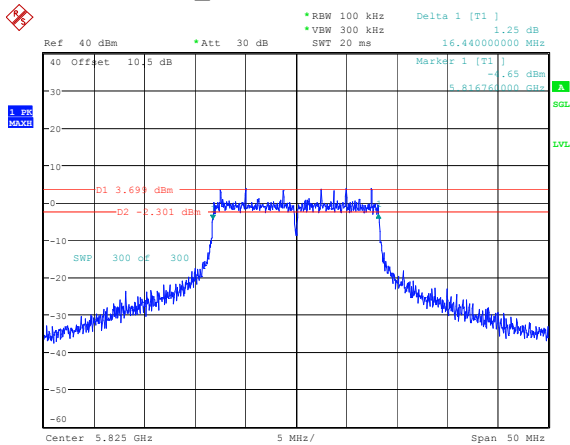
802.11a_5825MHz 16.440MHz
