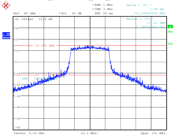
802.11ax40_5230MHz_RU_Full 79.124MHz
