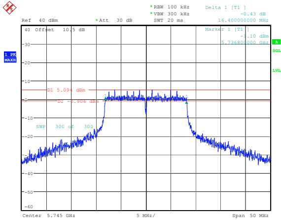
802.11a_5745MHz 16.400MHz
