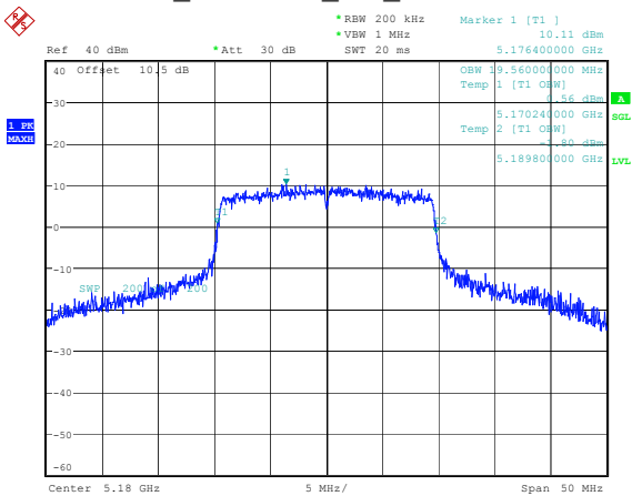
802.11ax20_5180MHz_RU_Full 19.560MHz
