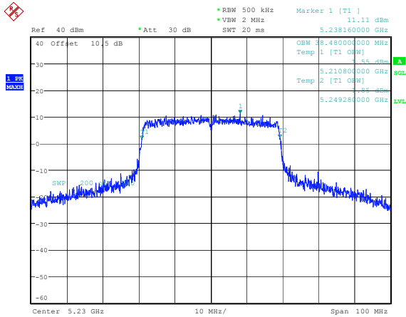
802.11ax40_5230MHz_RU_Full 38.480MHz
