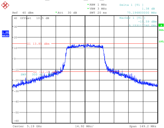
802.11ax40_5190MHz_RU_Full 75.197MHz
