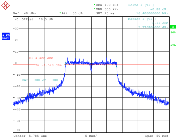
802.11a_5785MHz 16.400MHz
