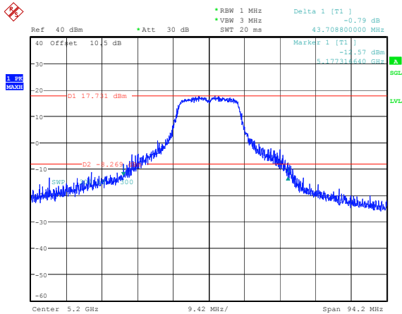
802.11a_5200MHz 43.709MHz
