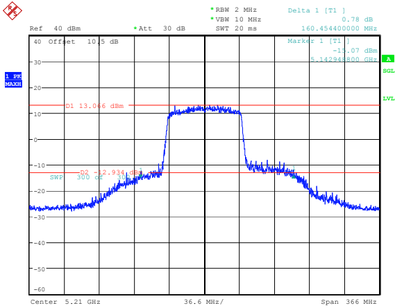
802.11ax80_5210MHz_RU_Full 160.454MHz
