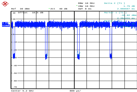
n20_5200MHz_Chain 0 1.951ms,2.067ms
