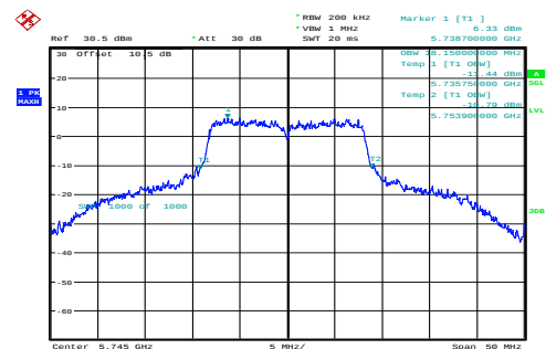
a_5745MHz_Chain 0 18.150MHz
