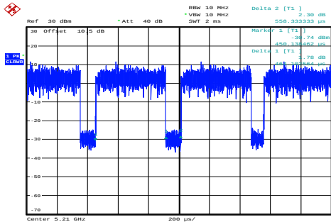
ac80_5210MHz_Chain 0 0.464ms,0.558ms
