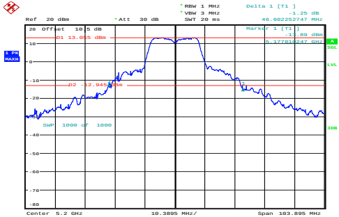
n20_5200MHz_Chain 0 46.602MHz
