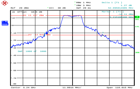
n20_5240MHz_Chain 0 52.095MHz
