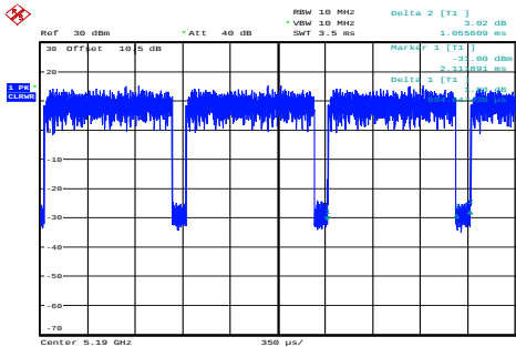
n40_5190MHz_Chain 0 0.955ms,1.056ms
