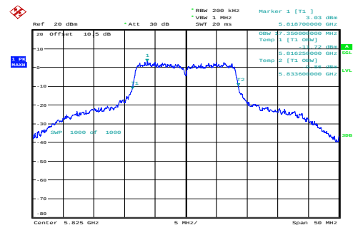
a_5825MHz_Chain 0 17.350MHz
