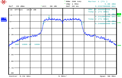
n20_5240MHz_Chain 0 18MHz
