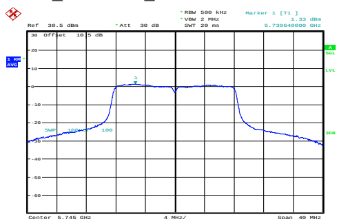
a_5745MHz_Chain 0 1.33dBm/MHz
