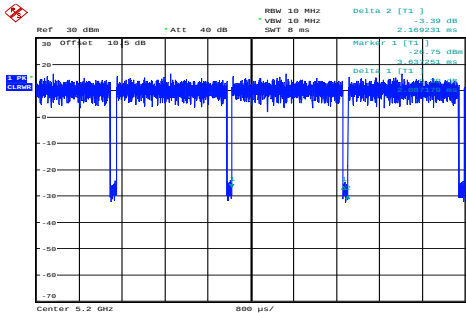
a_5200MHz_Chain 0 2.087ms,2.169ms
