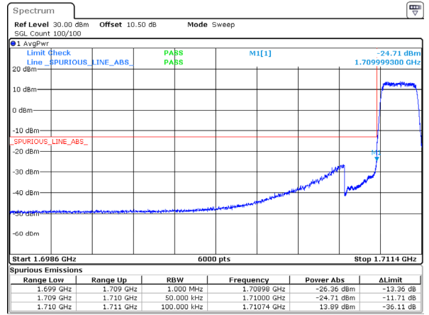
1.4MHz_Low_QPSK_6@0
