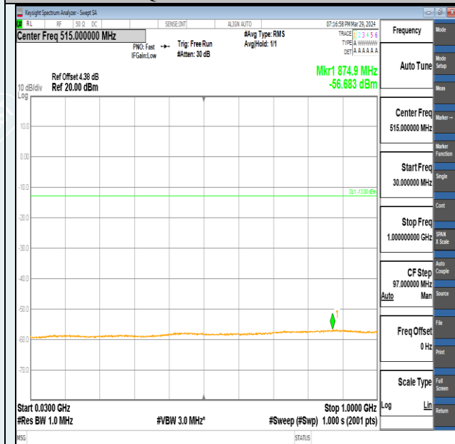
Band2-20MHz-QPSK-18700-1RB#99-30~1000-PASS
