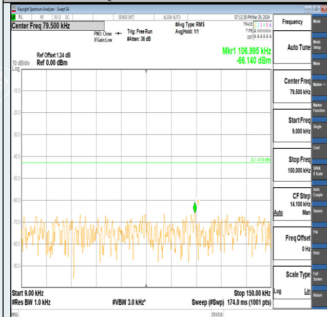
Band2-20MHz-QPSK-18700-100RB#0-0.009~0.15-PASS
