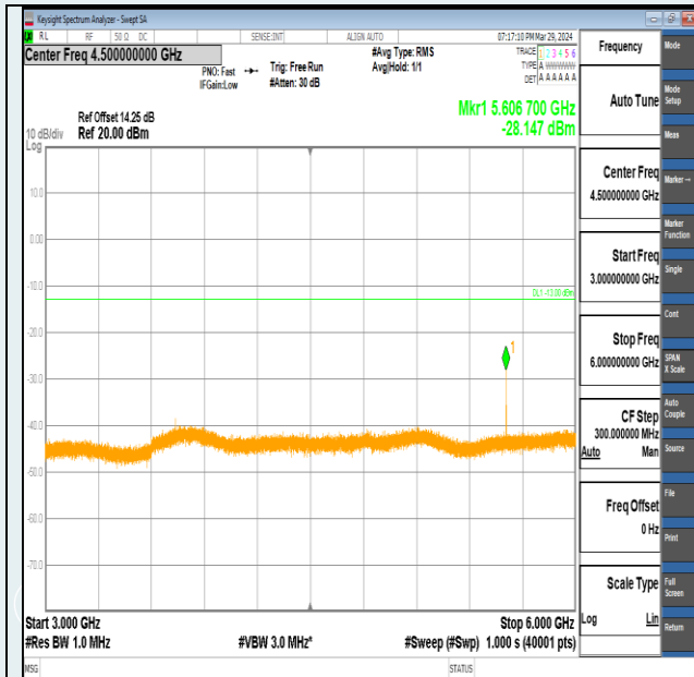
Band2-20MHz-QPSK-18700-1RB#99-3000~6000-PASS
