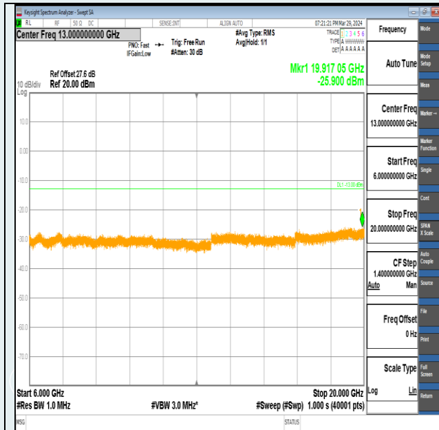
Band2-20MHz-QPSK-19100-1RB#0-6000~20000-PASS
