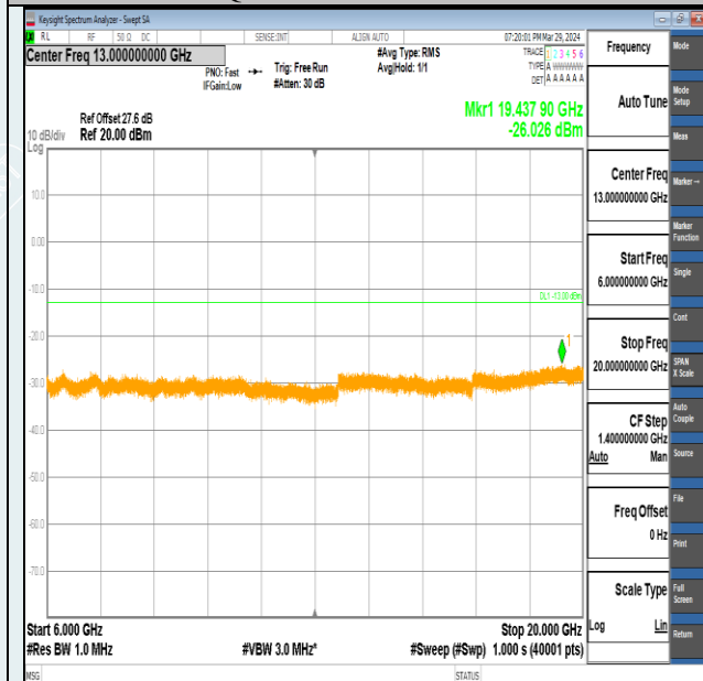
Band2-20MHz-QPSK-18900-1RB#99-6000~20000-PASS
