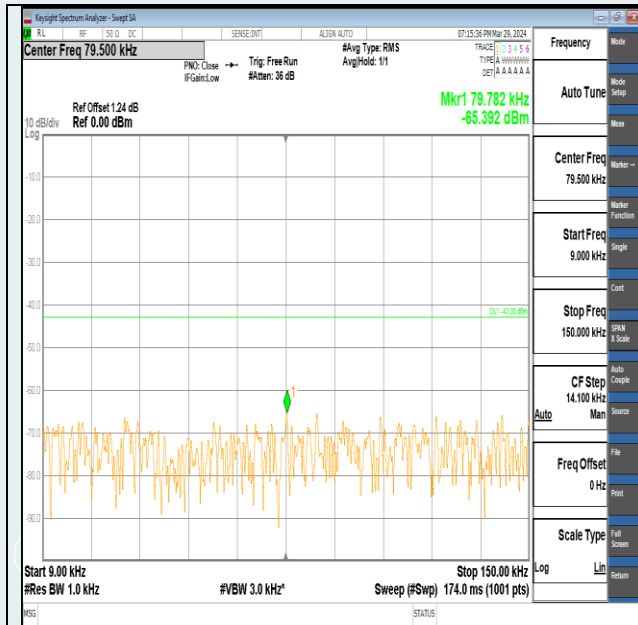
Band2-20MHz-QPSK-18700-1RB#0-0.009~0.15-PASS
