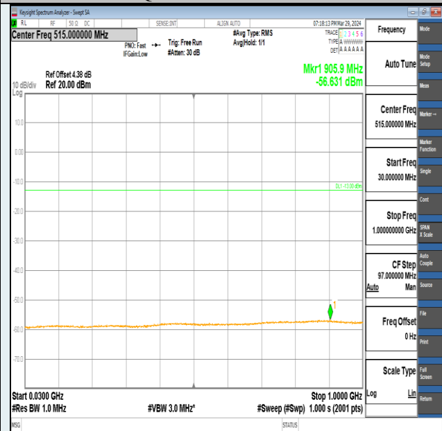
Band2-20MHz-QPSK-18900-1RB#0-30~1000-PASS
