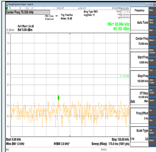
Band2-20MHz-QPSK-19100-100RB#0-0.009~0.15-PASS
