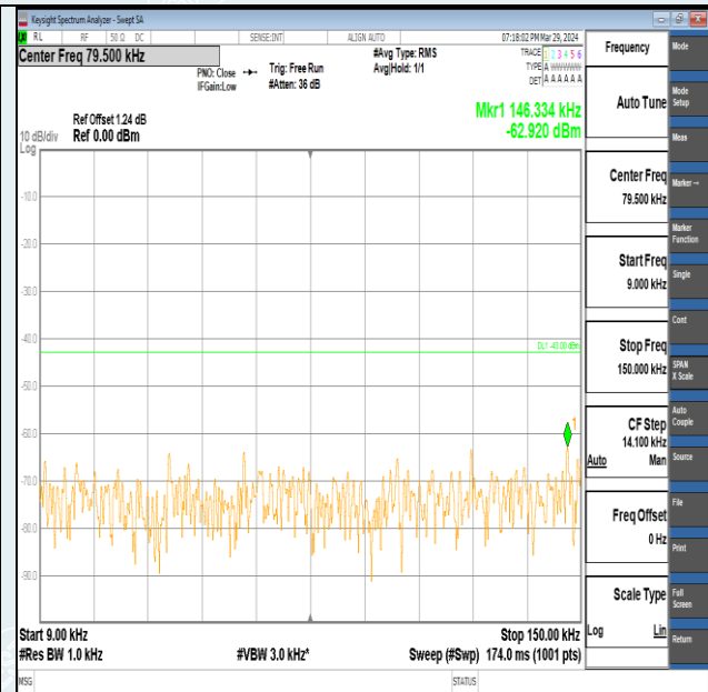
Band2-20MHz-QPSK-18900-1RB#0-0.009~0.15-PASS
