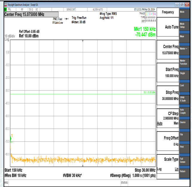
Band2-20MHz-QPSK-18900-100RB#0-0.15~30-PASS
