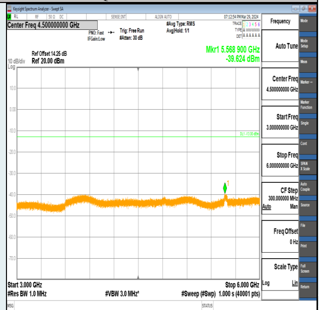
Band2-20MHz-QPSK-18700-100RB#0-3000~6000-PASS
