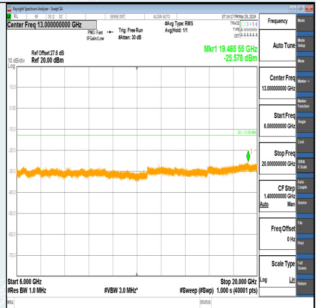
Band2-20MHz-QPSK-18900-100RB#0-6000~20000-PASS
