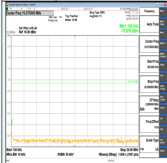
Band2-20MHz-QPSK-18900-1RB#99-0.15~30-PASS
