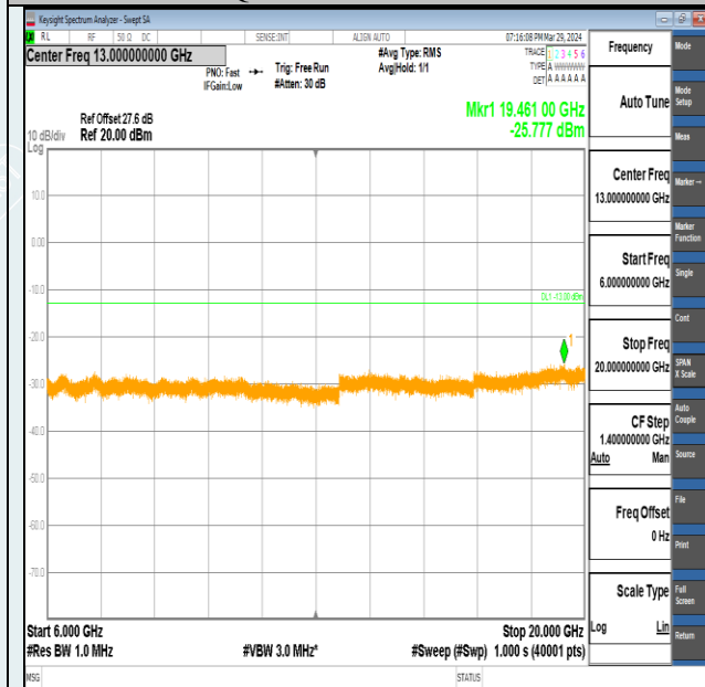
Band2-20MHz-QPSK-18700-1RB#0-6000~20000-PASS
