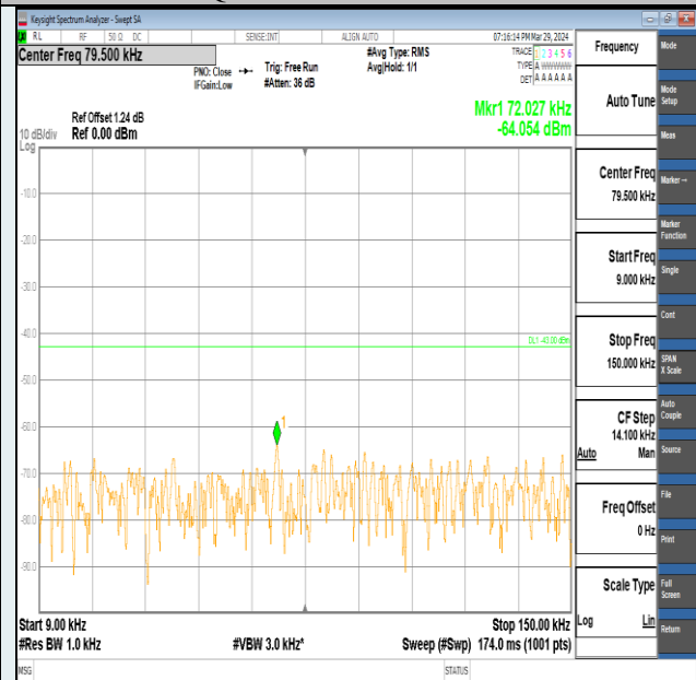
Band2-20MHz-16QAM-18700-1RB#0-0.009~0.15-PASS
