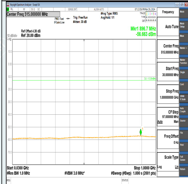
Band2-20MHz-QPSK-18900-100RB#0-30~1000-PASS
