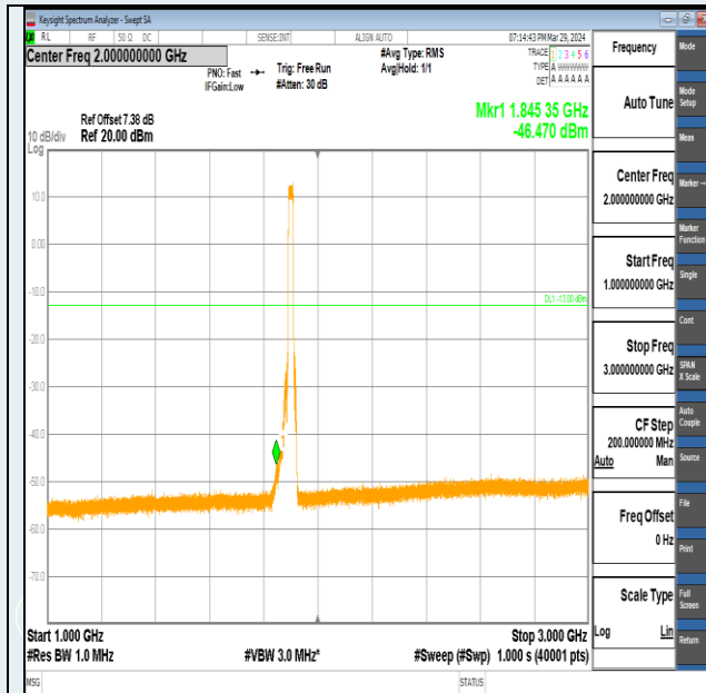
Band2-20MHz-QPSK-19100-100RB#0-1000~3000-PASS
