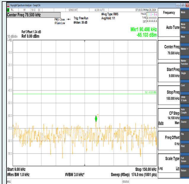
Band2-20MHz-QPSK-18900-1RB#99-0.009~0.15-PASS
