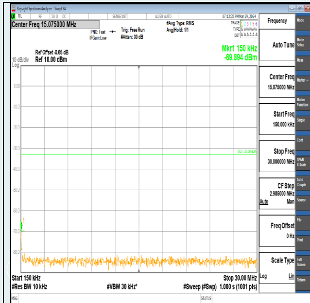
Band2-20MHz-QPSK-18700-100RB#0-0.15~30-PASS
