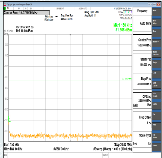
Band2-20MHz-QPSK-18700-1RB#99-0.15~30-PASS
