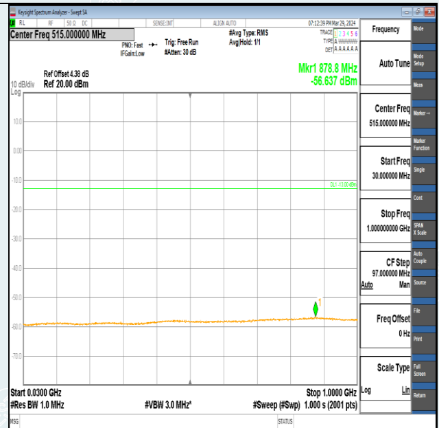
Band2-20MHz-QPSK-18700-100RB#0-30~1000-PASS
