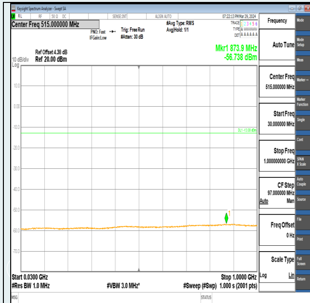
Band2-20MHz-QPSK-19100-1RB#99-30~1000-PASS
