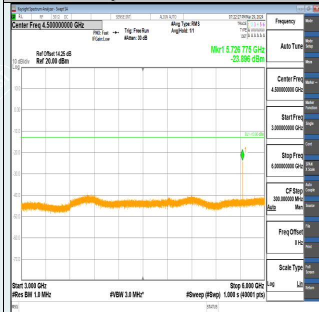
Band2-20MHz-QPSK-19100-1RB#99-3000~6000-PASS
