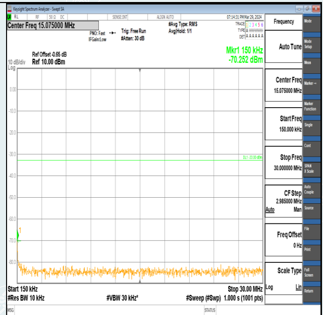
Band2-20MHz-QPSK-19100-100RB#0-0.15~30-PASS
