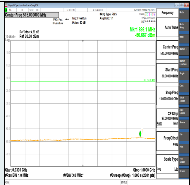
Band2-20MHz-QPSK-18900-1RB#99-30~1000-PASS
