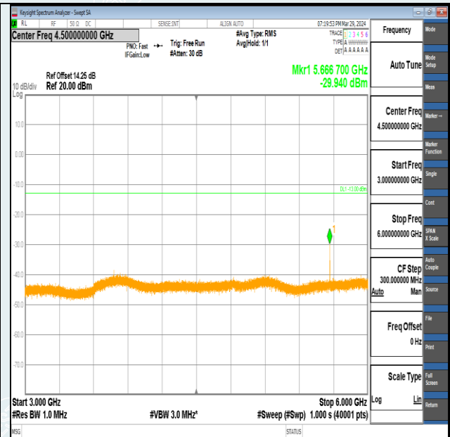
Band2-20MHz-QPSK-18900-1RB#99-3000~6000-PASS
