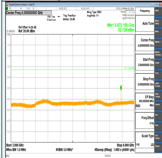
Band2-20MHz-QPSK-19100-1RB#0-3000~6000-PASS
