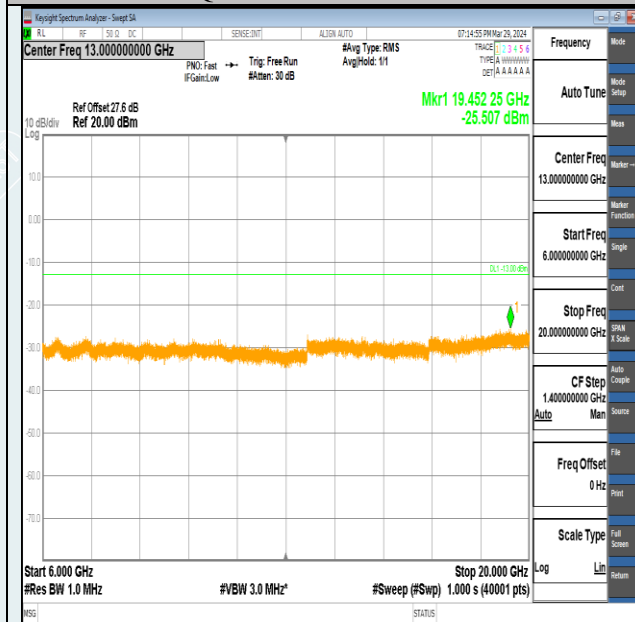
Band2-20MHz-QPSK-19100-100RB#0-6000~20000-PASS
