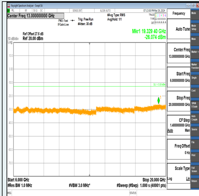
Band2-20MHz-QPSK-18700-100RB#0-6000~20000-PASS
