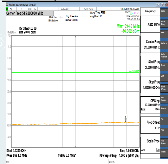
Band2-20MHz-QPSK-19100-100RB#0-30~1000-PASS
