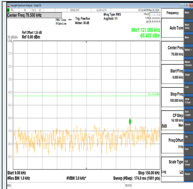
Band2-20MHz-QPSK-18700-1RB#99-0.009~0.15-PASS
