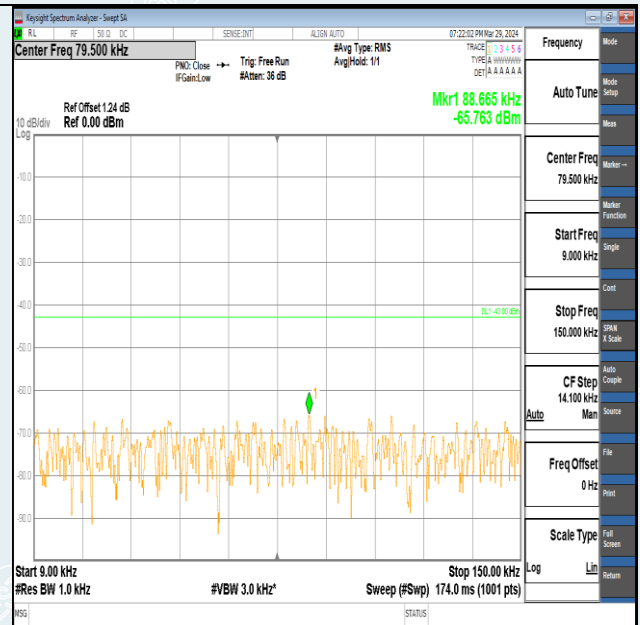
Band2-20MHz-QPSK-19100-1RB#99-0.009~0.15-PASS
