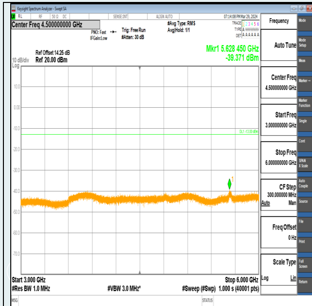
Band2-20MHz-QPSK-18900-100RB#0-3000~6000-PASS
