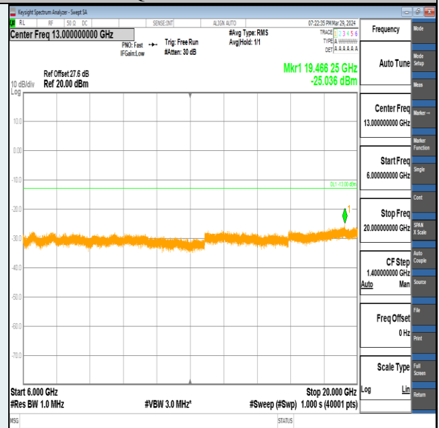
Band2-20MHz-QPSK-19100-1RB#99-6000~20000-PASS
