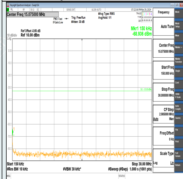
Band2-20MHz-QPSK-19100-1RB#99-0.15~30-PASS
