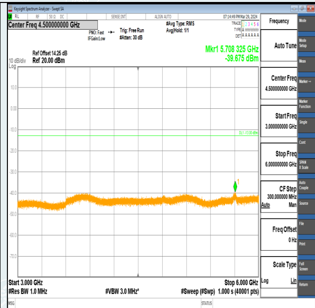
Band2-20MHz-QPSK-19100-100RB#0-3000~6000-PASS
