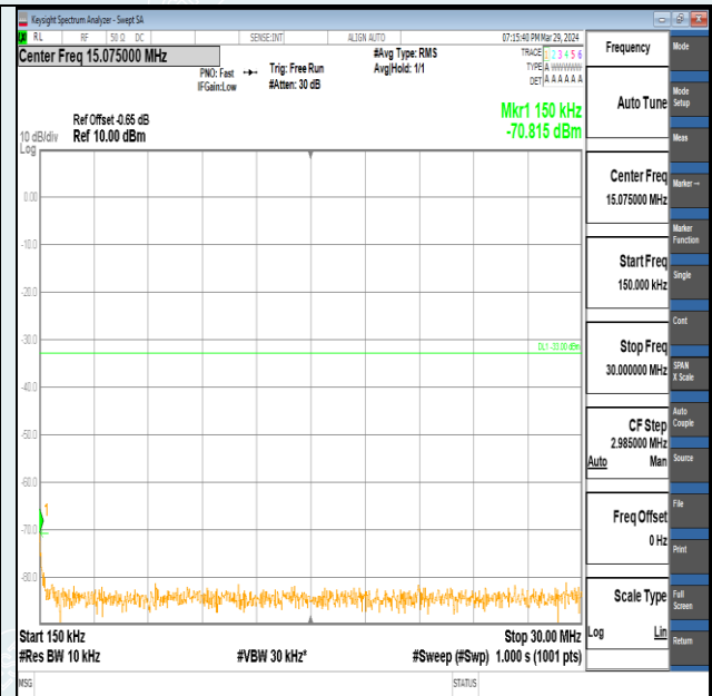
Band2-20MHz-QPSK-18700-1RB#0-0.15~30-PASS
