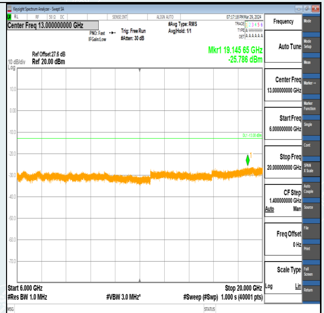
Band2-20MHz-QPSK-18700-1RB#99-6000~20000-PASS
