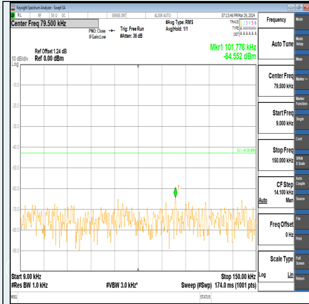
Band2-20MHz-QPSK-18900-100RB#0-0.009~0.15-PASS
