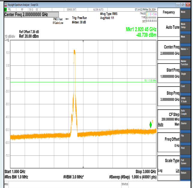
Band2-20MHz-QPSK-18900-100RB#0-1000~3000-PASS
