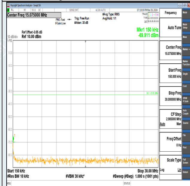
Band2-20MHz-QPSK-18900-1RB#0-0.15~30-PASS
