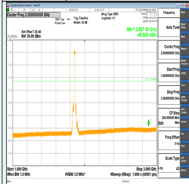
Band2-20MHz-QPSK-18700-100RB#0-1000~3000-PASS
