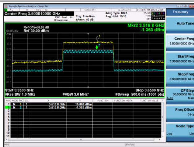
NTNT-n77(3450-3550)-PC2-30-100-M-CP-256QAM-Out_ _ Full-Ant1-PASS
