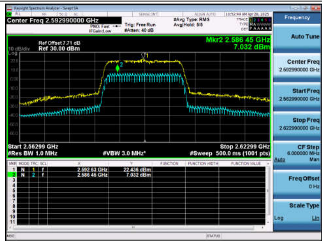
NTNT-n41-PC2-30-30-M-DFT-256QAM-Outet_Full-Ant1-PA
