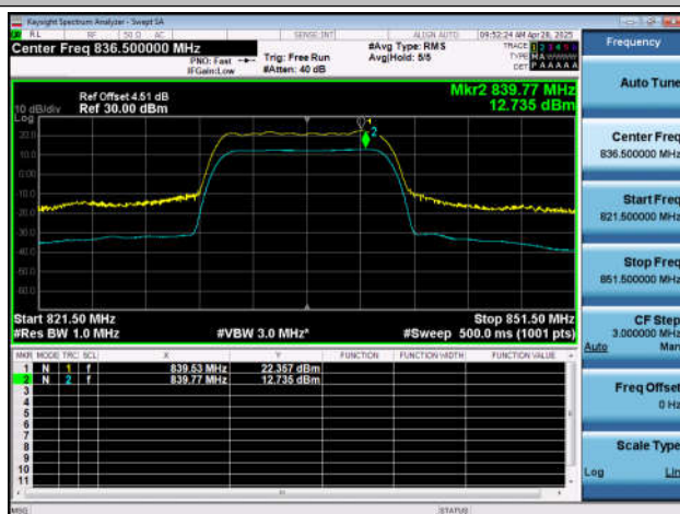
NTNT-n5-PC3-15-10-M-DFT-256QAM-Outer_Full-Ant1-PAS
