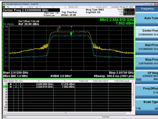
NTNT-n7-PC3-15-20-M-DFT-256QAM-Outer_Full-Ant1-PAS
