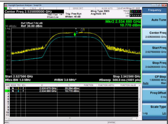
NTNT-n7-PC3-15-5-M-CP-256QAM-Outer_Full-Ant1-PASS
