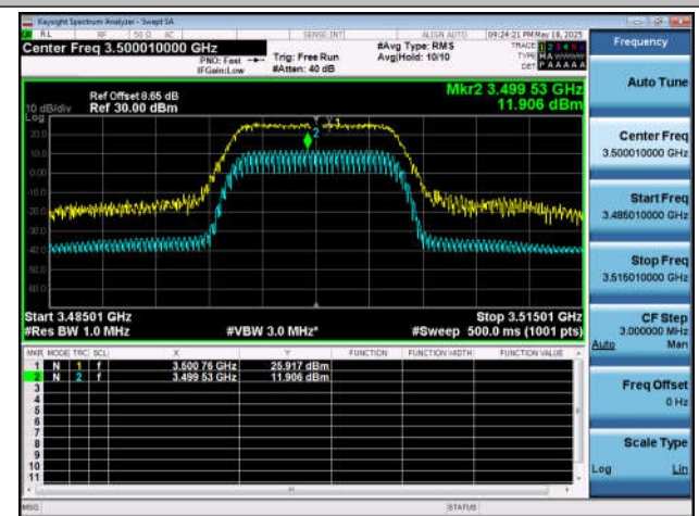
NTNT-n78(3450-3550)-PC2-30-10-M-DFT-256QAM-Out_ _ Full-Ant1-PASS
