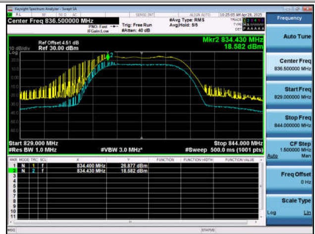
NTNT-n26(824-849)-PC3-15-10-M-DFT-256QAM-Outer_Full-I-Ant1-PASS
