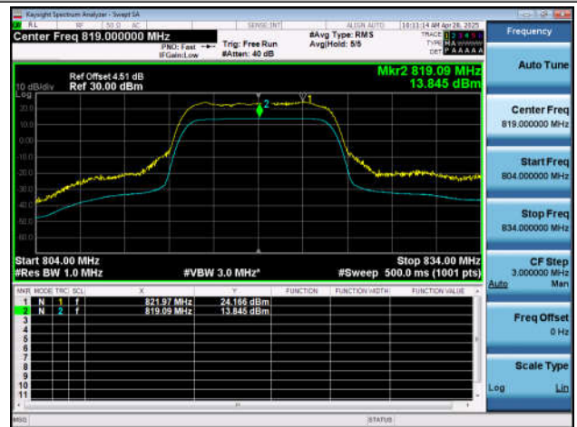
NTNT-n26(814-824)-PC3-15-10-M-CP-QPSK-Outer_Full-A
