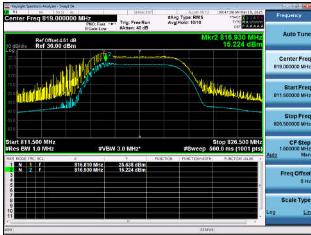
NTNT-n26(814-824)-PC3-15-10-M-DFT-256QAM-Outer_Full
