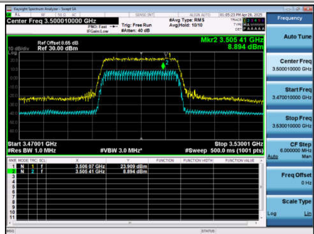
NTNT-n77(3450-3550)-PC2-30-20-M-DFT-256QAM-Outer_
