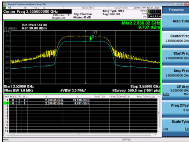
NTNT-n7-PC3-15-15-M-DFT-256QAM-Outer_Full-Ant1-PAS
