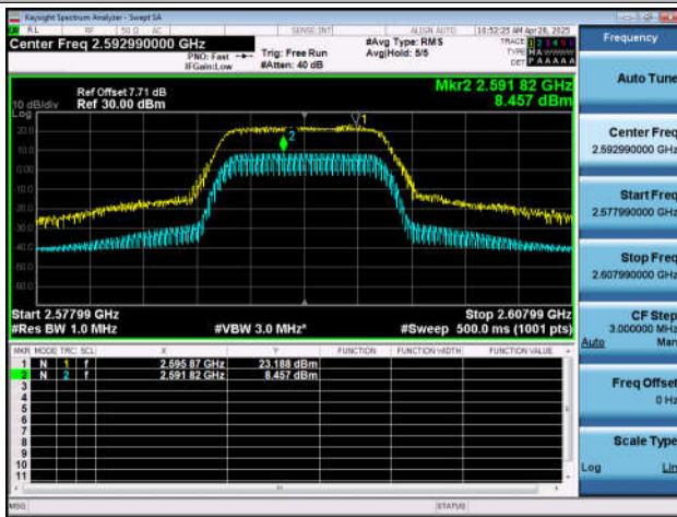
NTNT-n41-PC2-30-20-M-CP-256QAM-Outet_Full-Ant1-PA
