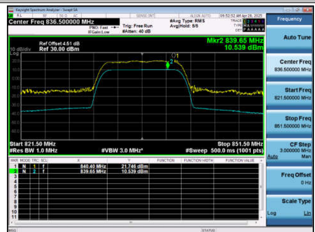
NTNT-n5-PC3-15-10-M-CP-256QAM-Outer_Full-Ant1-PAS
