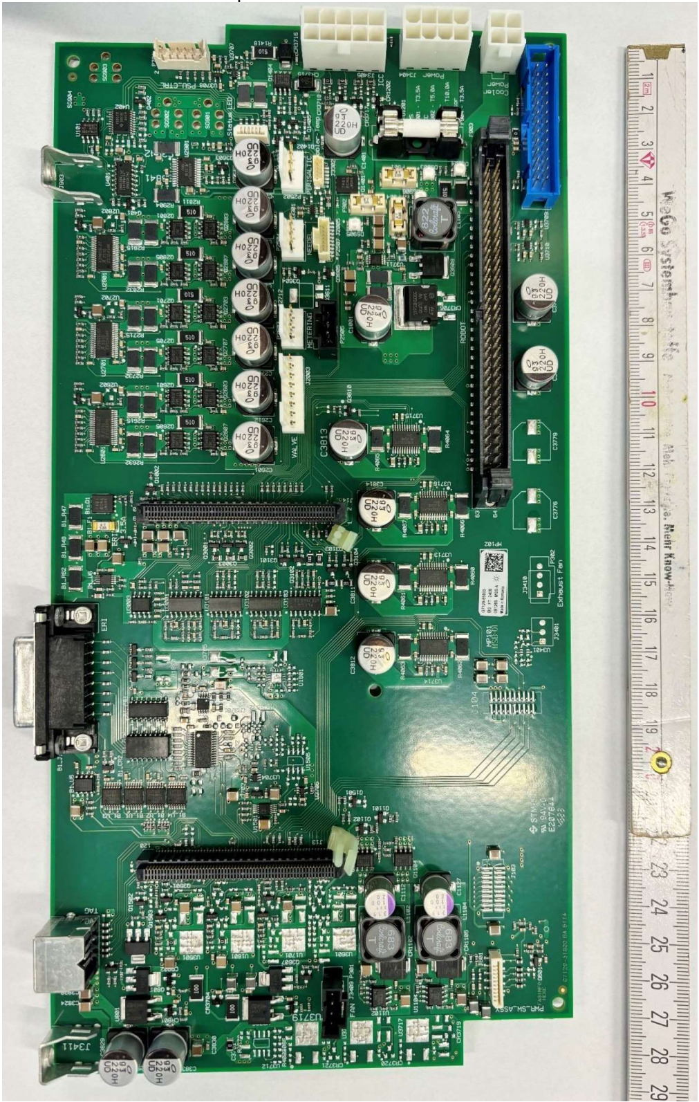
Top view of the Main-Board PCB
