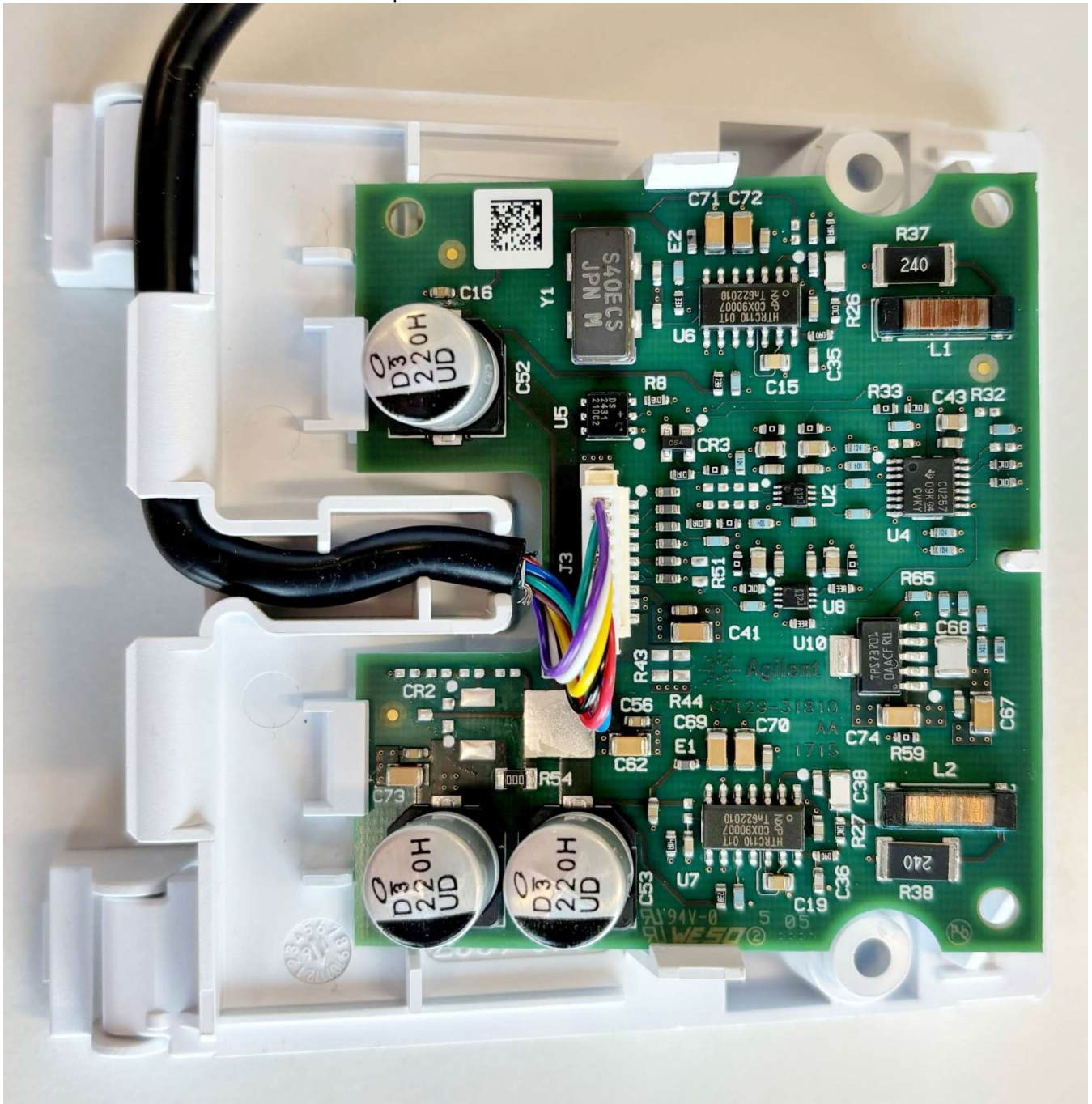
Top view of the ext. TAG reader PCB
