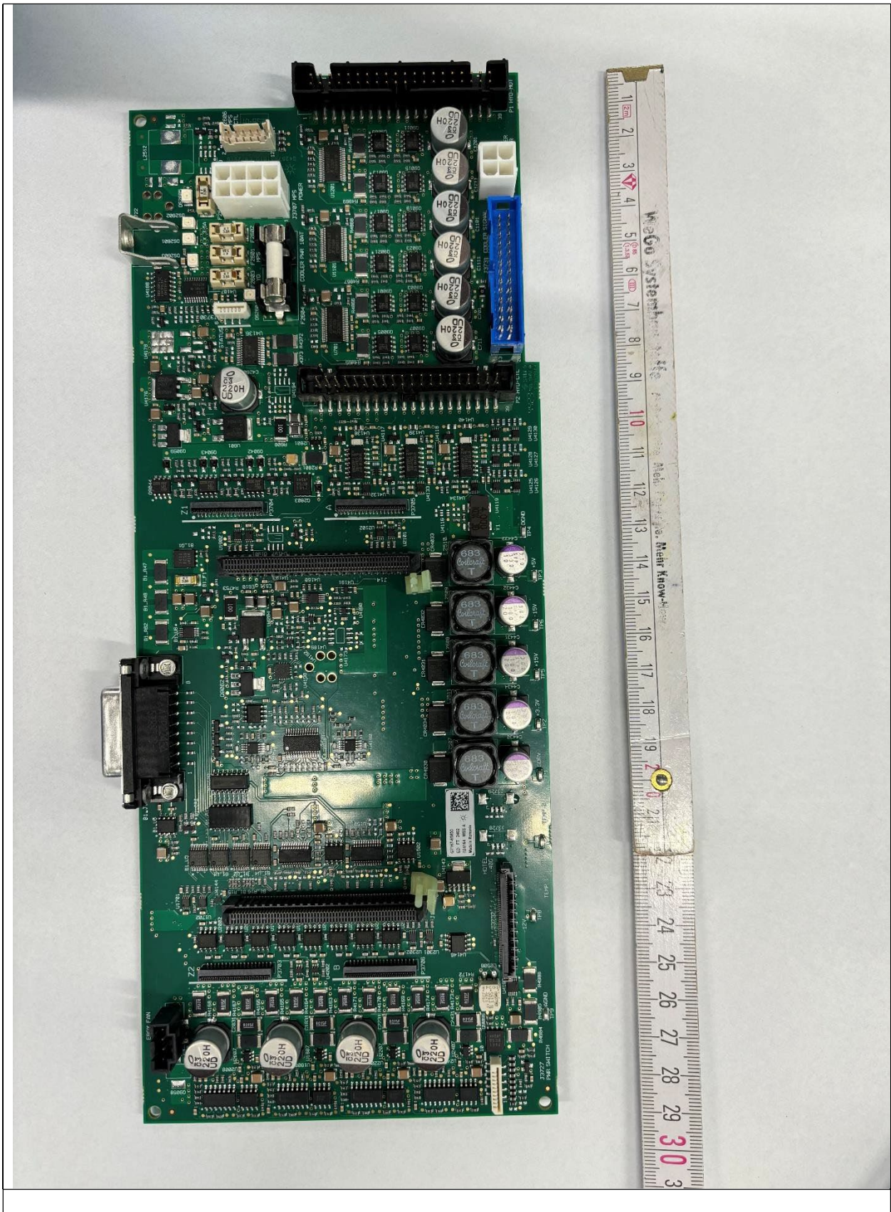
Main-Board top
