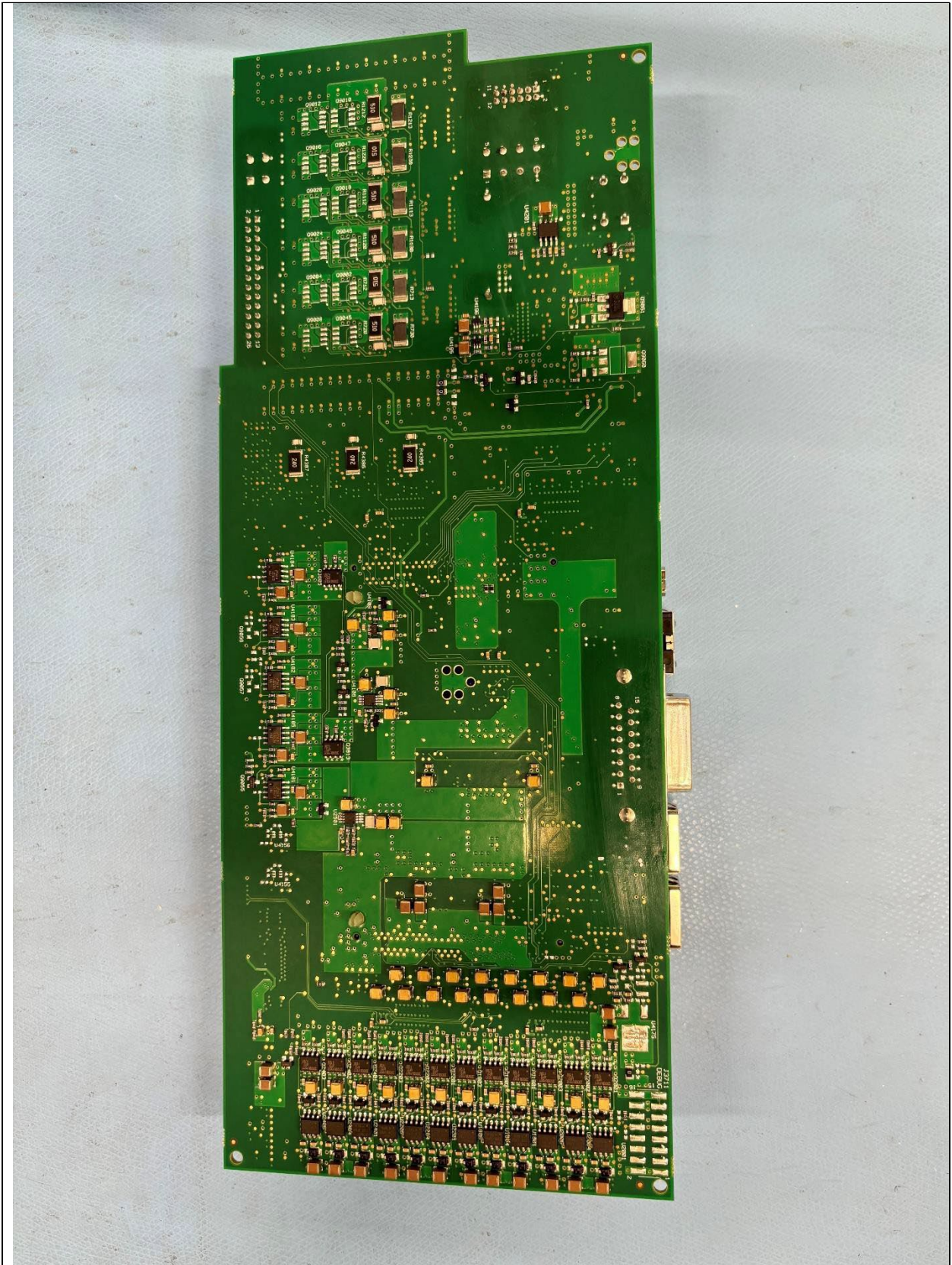
Main-Board bottom
