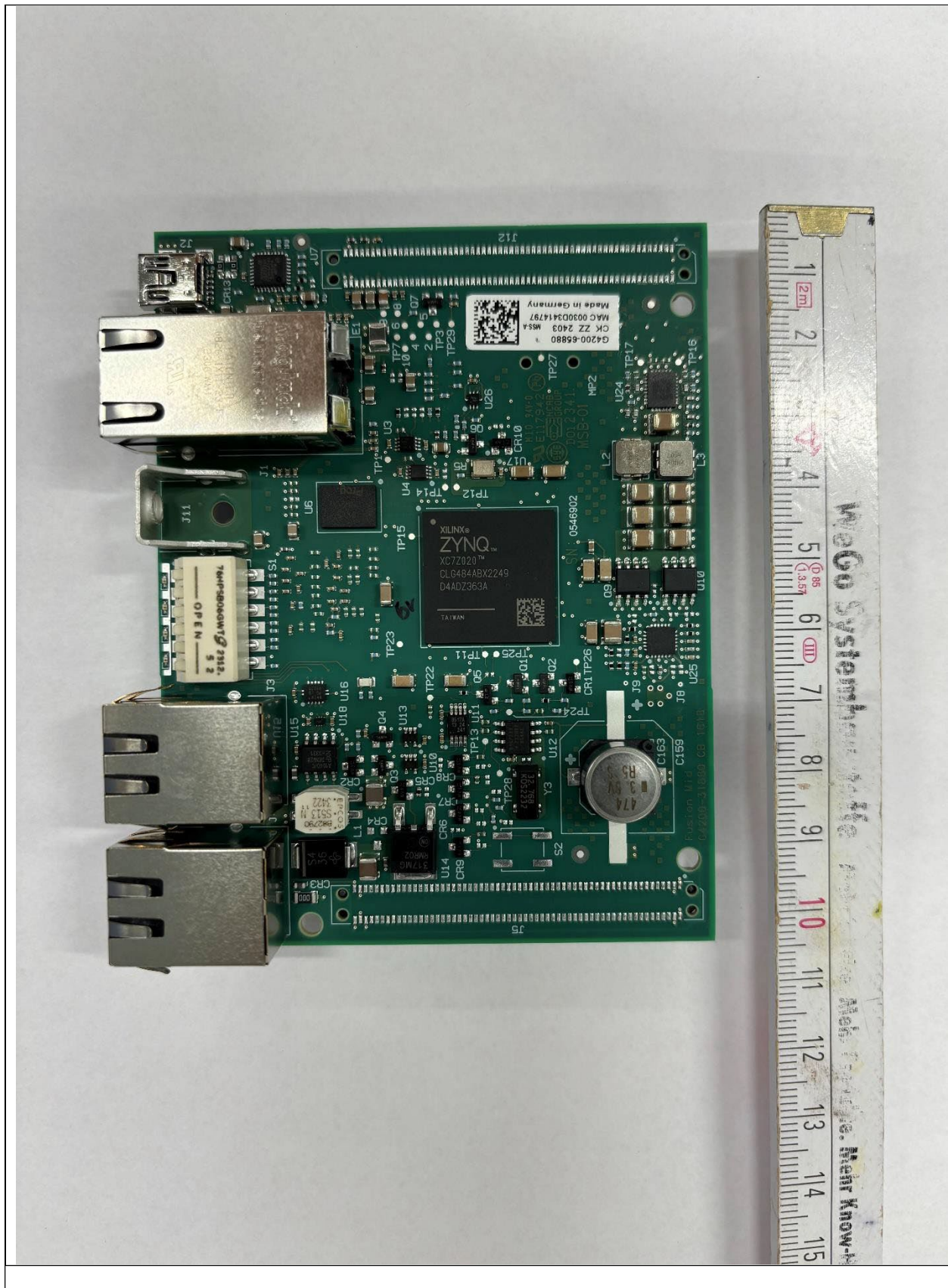
Processor board top
