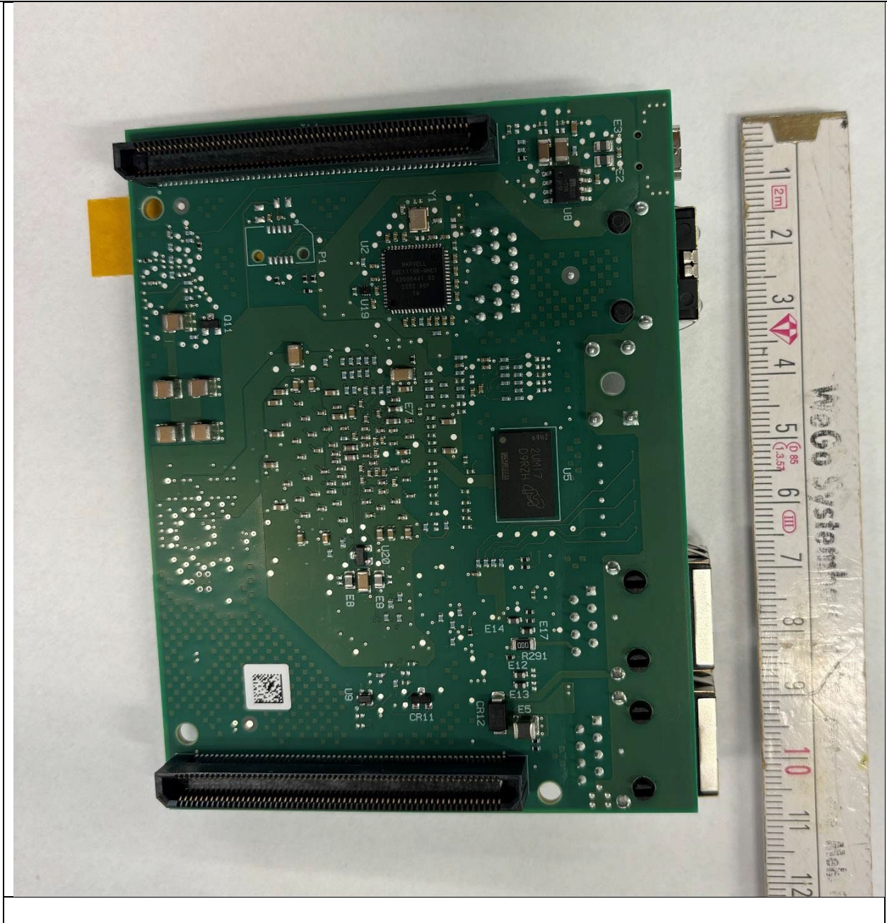
Processor board bottom
