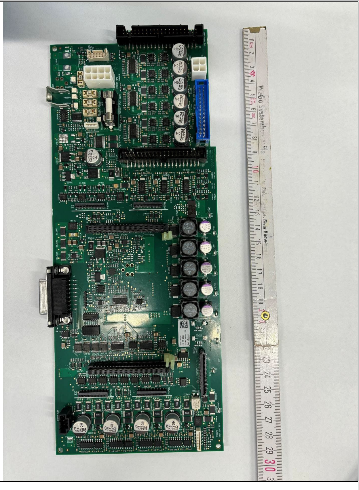
Main-Board top
