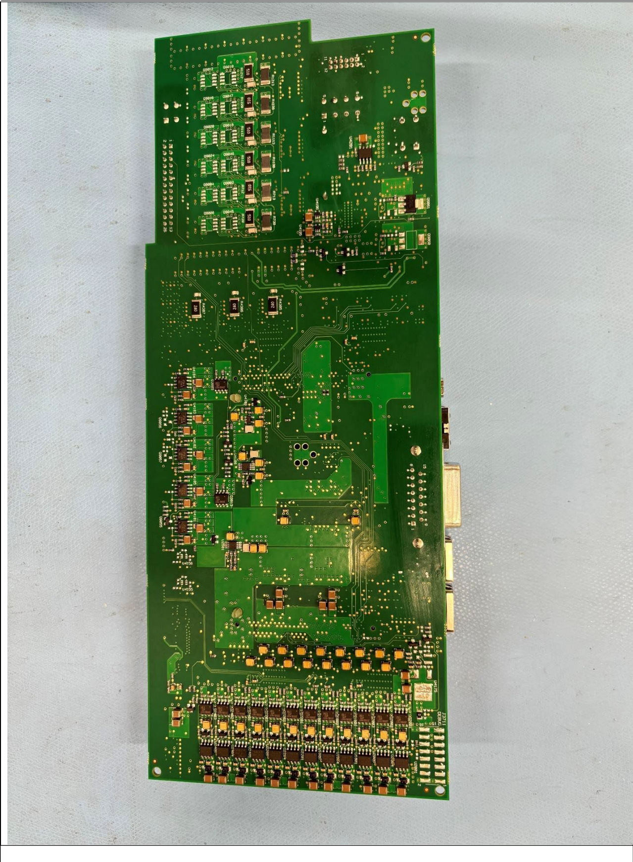
Main-Board bottom
