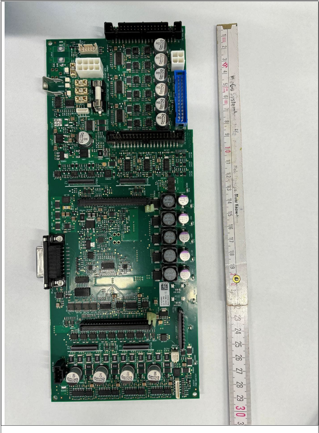
Main-Board top
