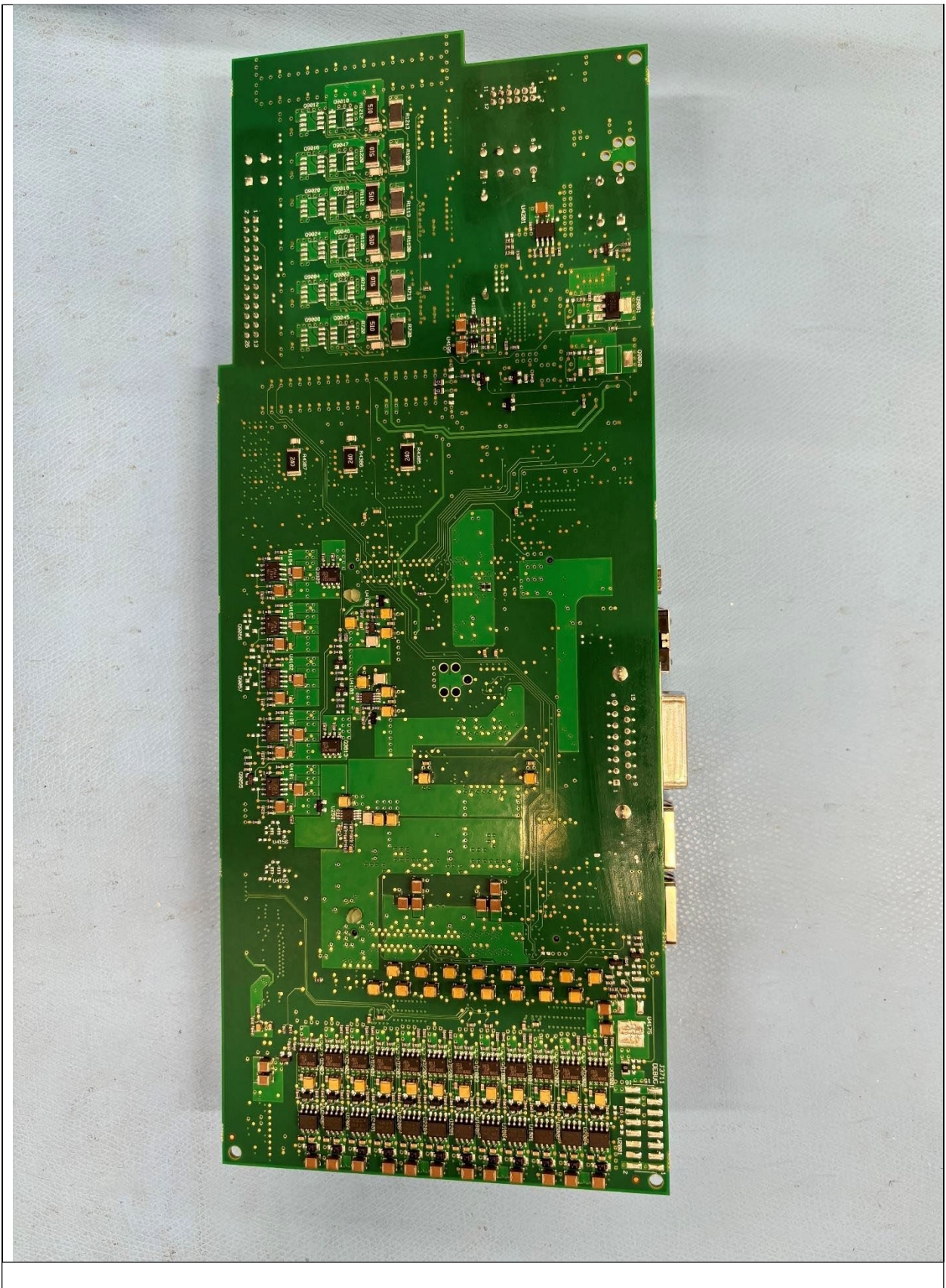
Main-Board bottom
