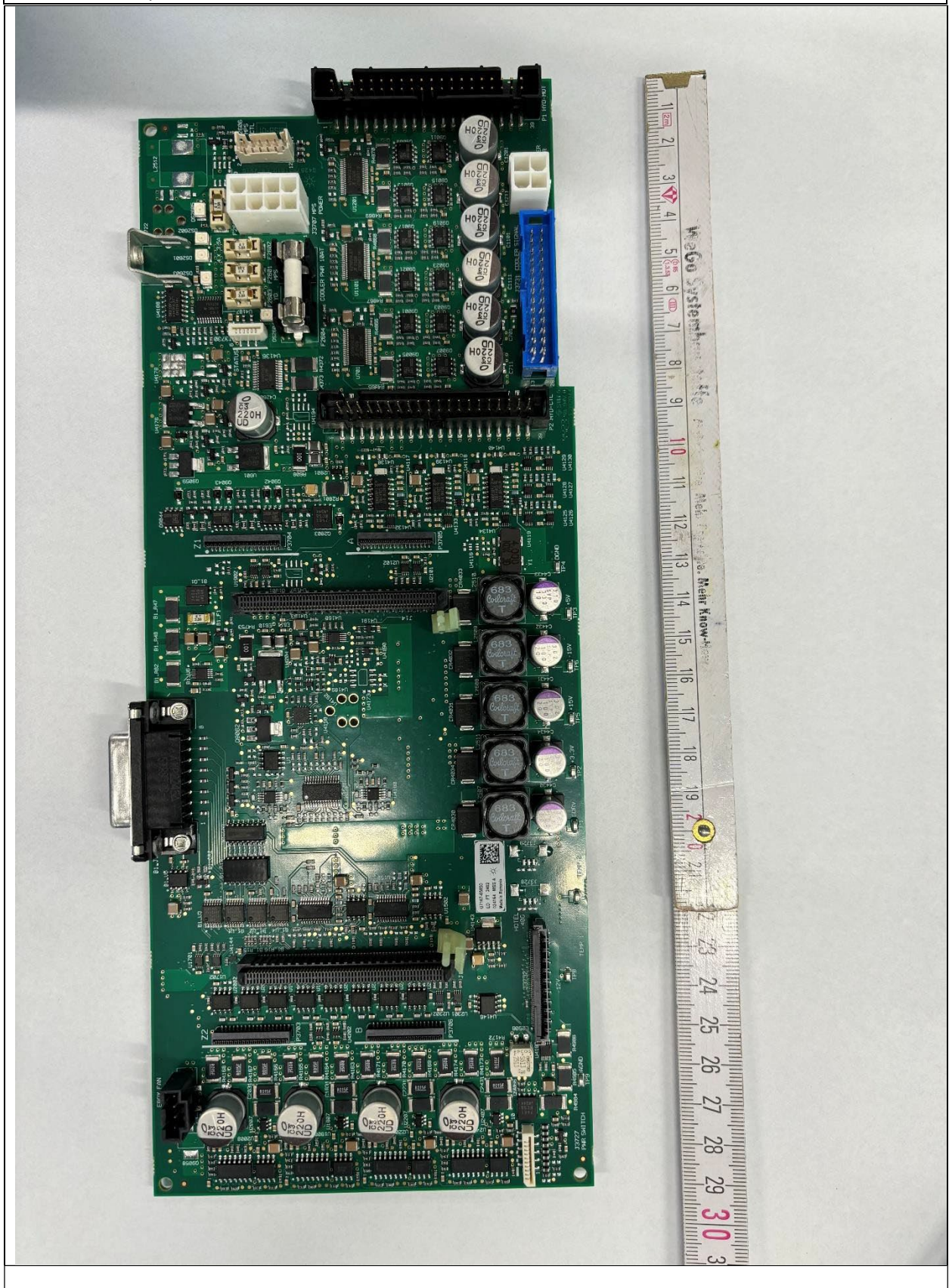
Main-Board top
