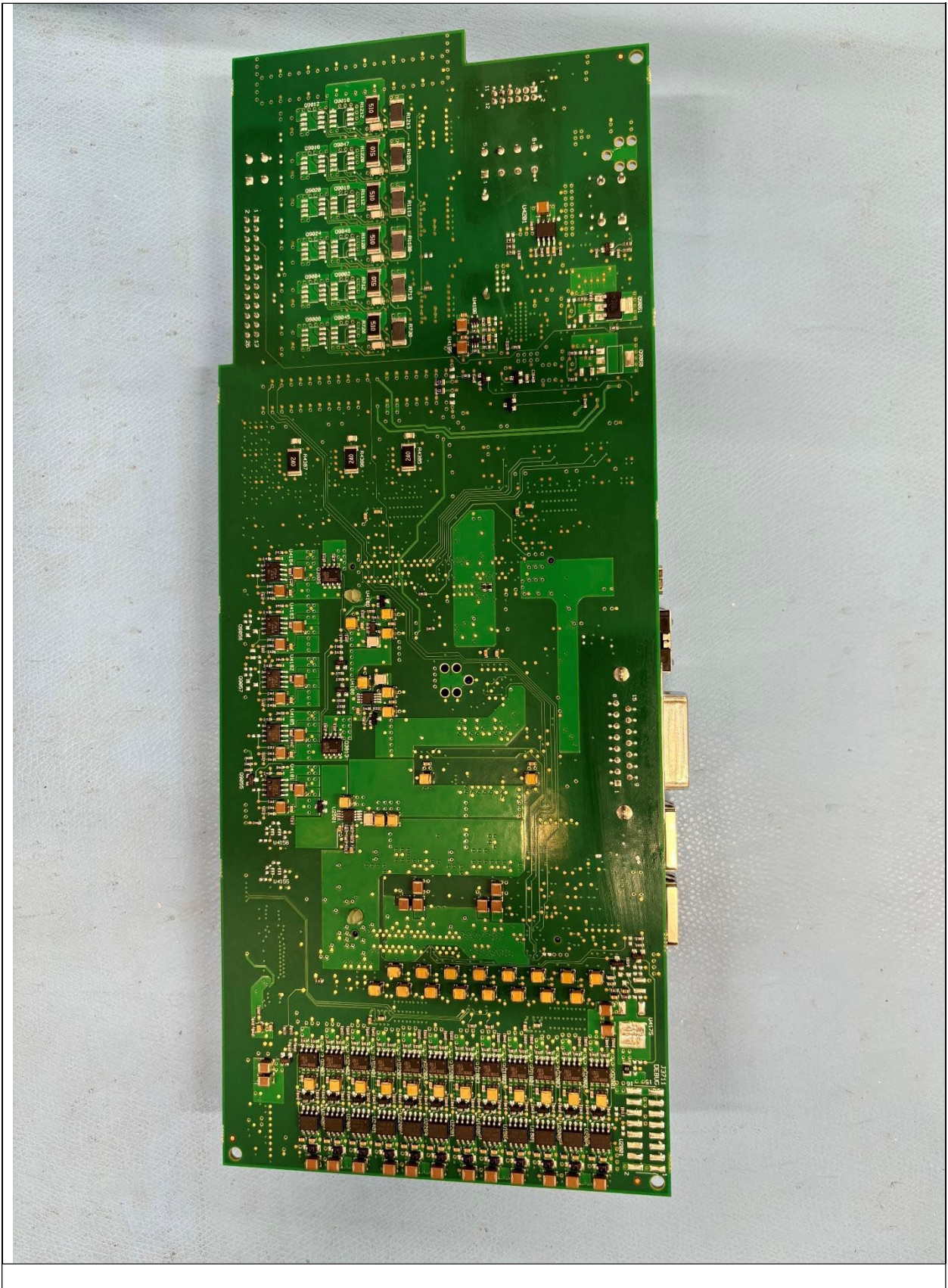
Main-Board bottom
