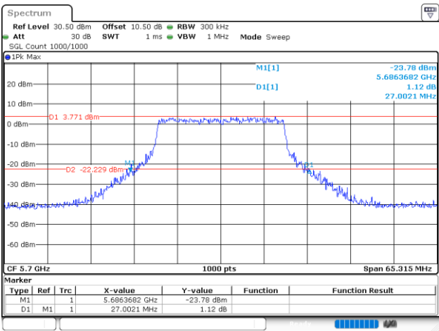
802.11ax20_5700MHz_RU_Full
