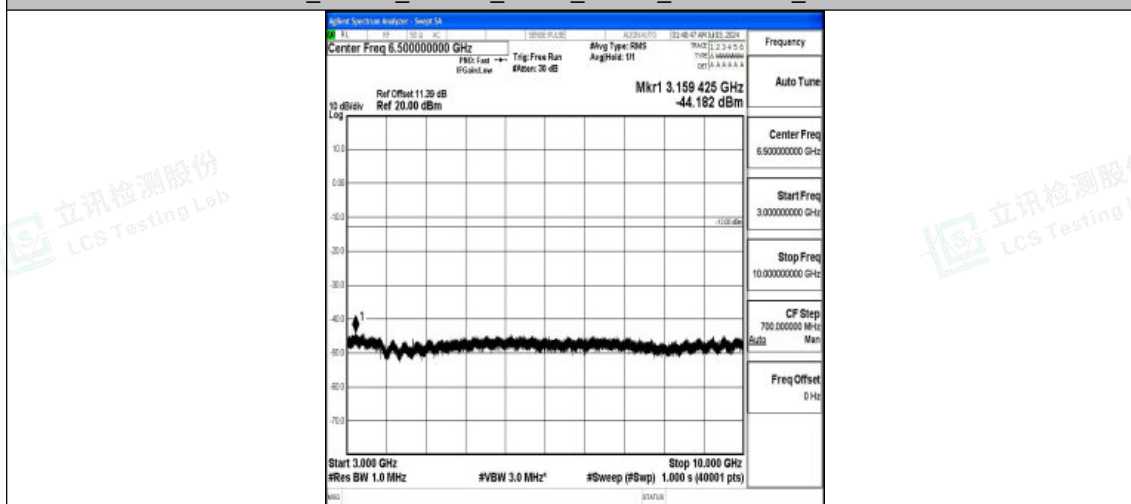
Band26_15MHz_16QAM_26965_1RB#0_3000~10000_3000~10000
