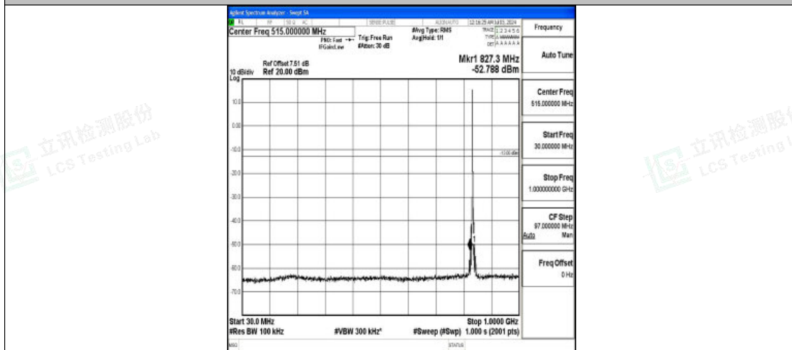
Band26_3MHz_16QAM_26915_1RB#0_30~1000_30~1000
