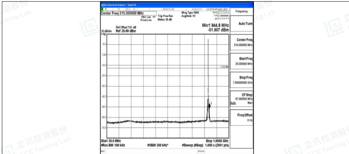
Band26_3MHz_QPSK_26915_1RB#0_30~1000_30~1000
