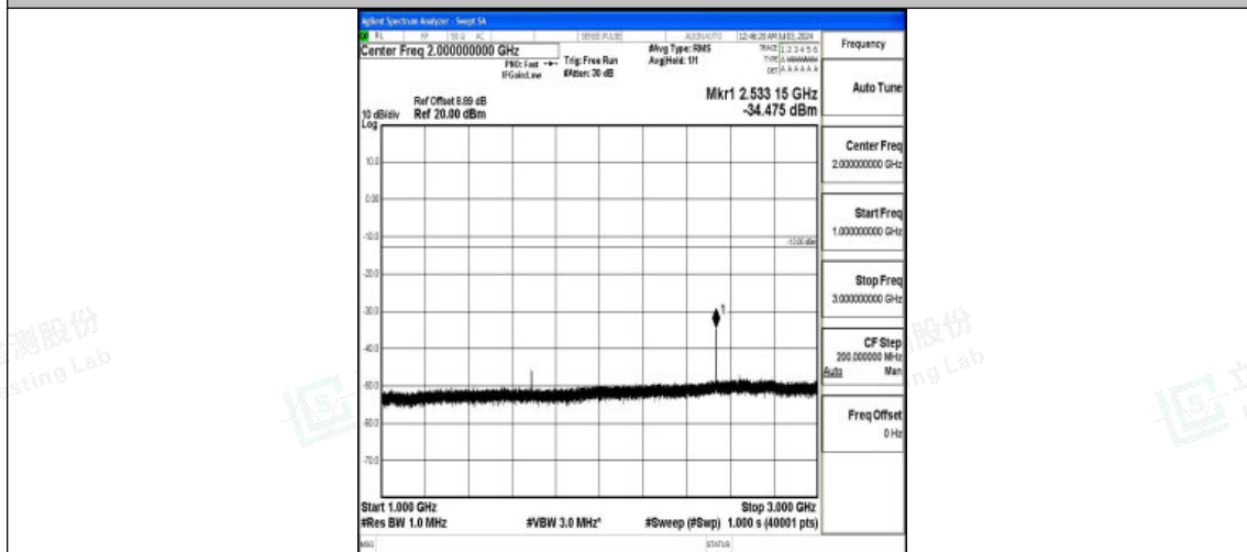
Band26_5MHz_16QAM_27015_1RB#0_1000~3000_1000~3000
