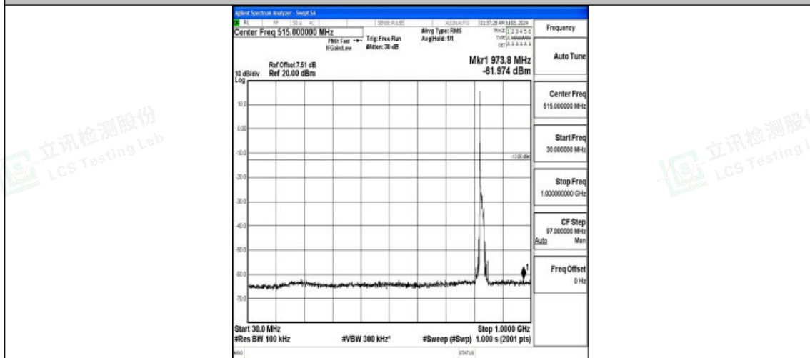
Band26_15MHz_QPSK_26865_1RB#0_30~1000_30~1000
