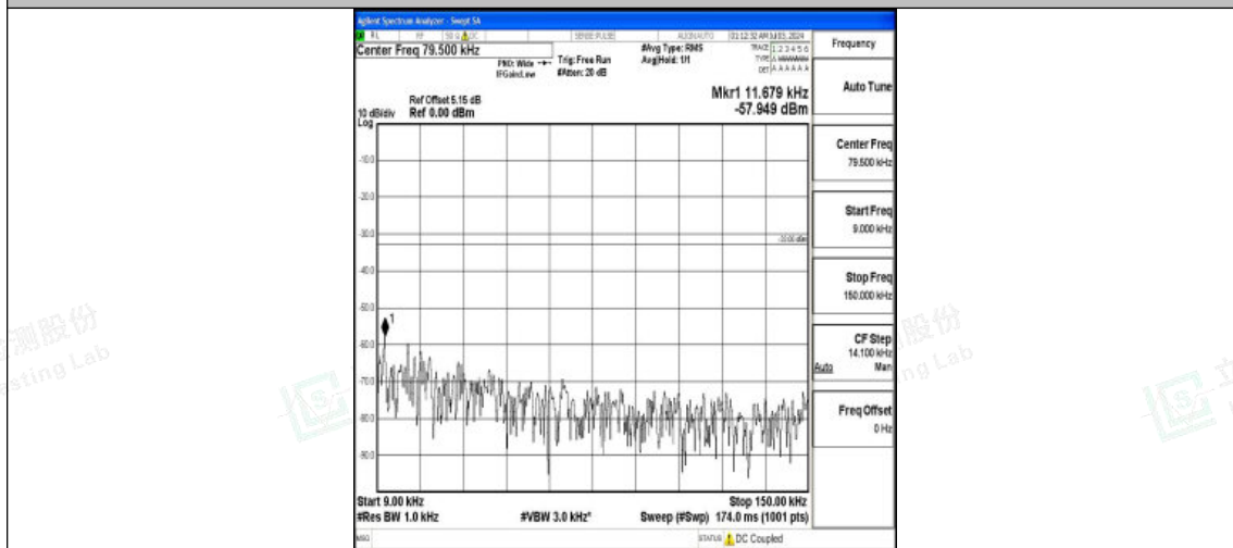
Band26_10MHz_QPSK_26915_1RB#0_0.009~0.15_0.009~0.15
