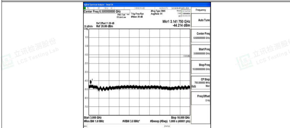
Band26_3MHz_QPSK_26915_1RB#0_3000~10000_3000~10000
