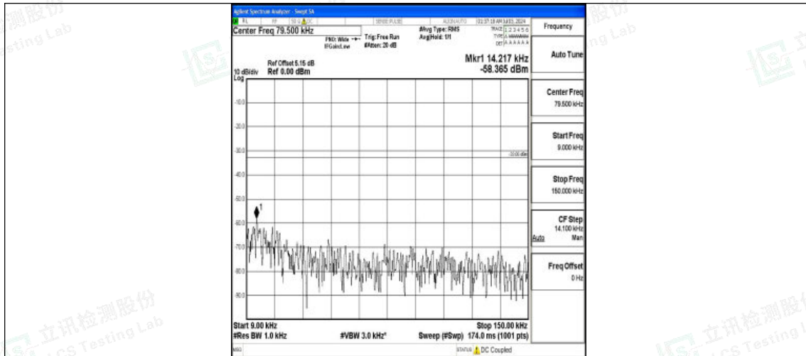
Band26_15MHz_QPSK_26865_1RB#0_0.009~0.15_0.009~0.15
