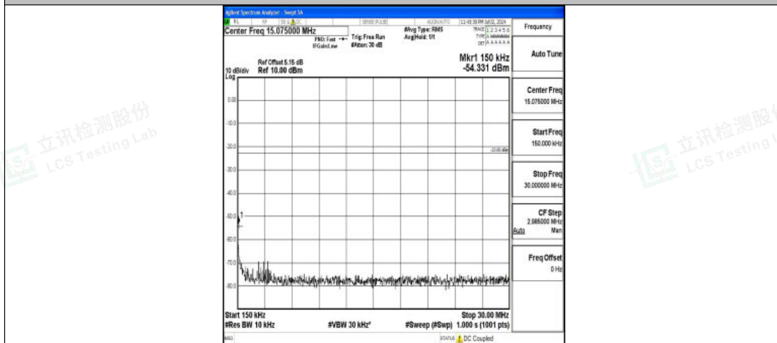
Band26_1.4MHz_16QAM_27033_1RB#0_0.15~30_0.15~30
