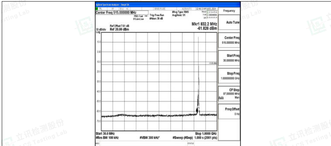
Band26_5MHz_16QAM_27015_1RB#0_30~1000_30~1000
