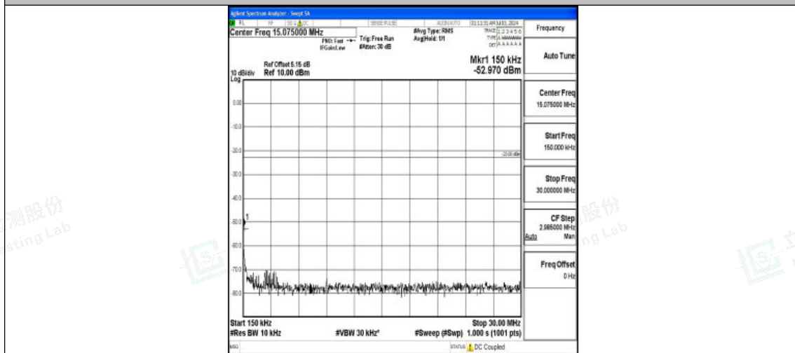
Band26_10MHz_QPSK_26840_1RB#0_0.15~30_0.15~30
