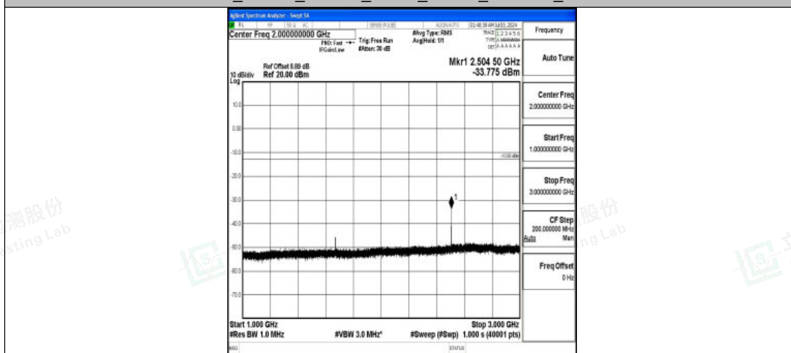
Band26_15MHz_16QAM_26965_1RB#0_1000~3000_1000~3000
