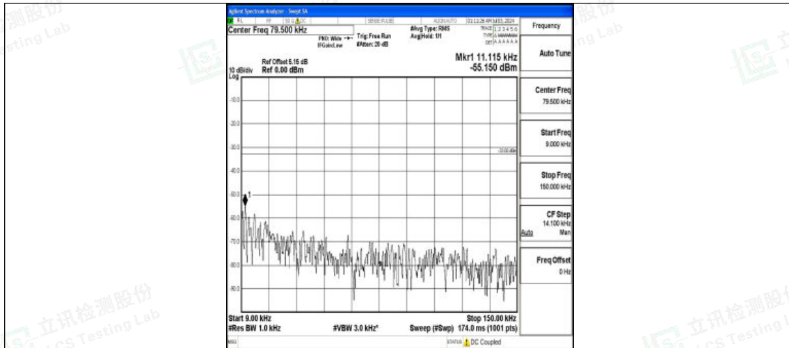
Band26_10MHz_QPSK_26840_1RB#0_0.009~0.15_0.009~0.15
