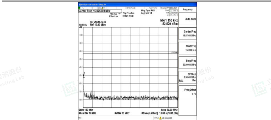
Band26_10MHz_16QAM_26915_1RB#0_0.15~30_0.15~30
