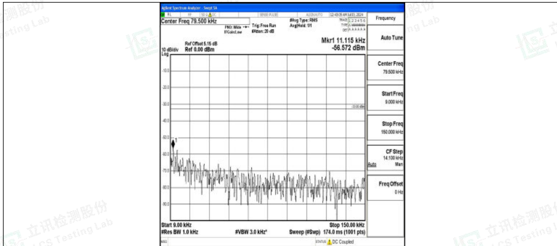
Band26_5MHz_QPSK_26815_1RB#0_0.009~0.15_0.009~0.15
