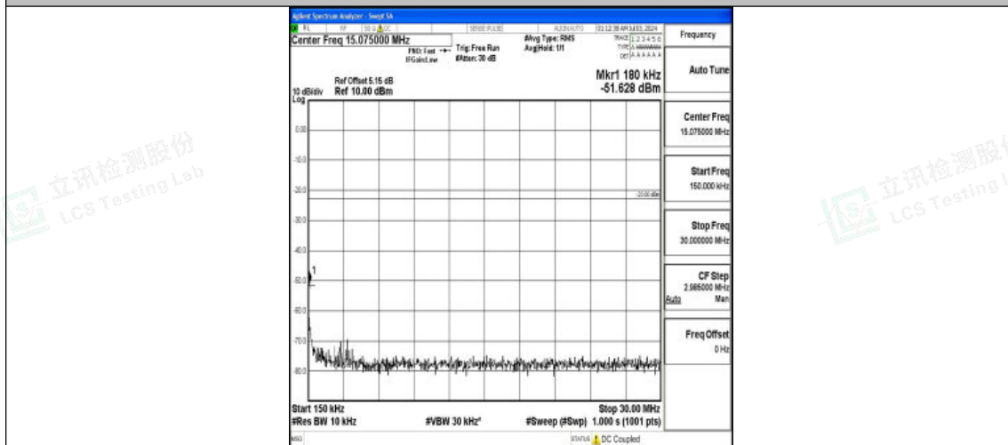
Band26_10MHz_QPSK_26915_1RB#0_0.15~30_0.15~30
