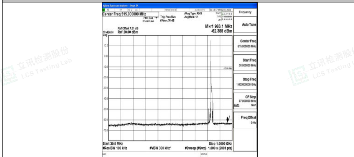
Band26_10MHz_16QAM_26915_1RB#0_30~1000_30~1000
