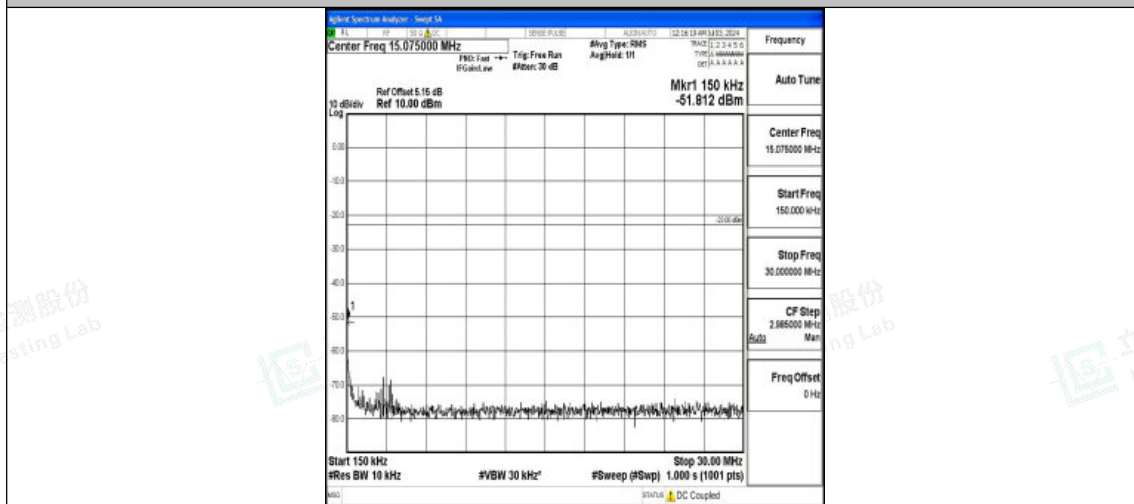
Band26_3MHz_16QAM_26915_1RB#0_0.15~30_0.15~30
