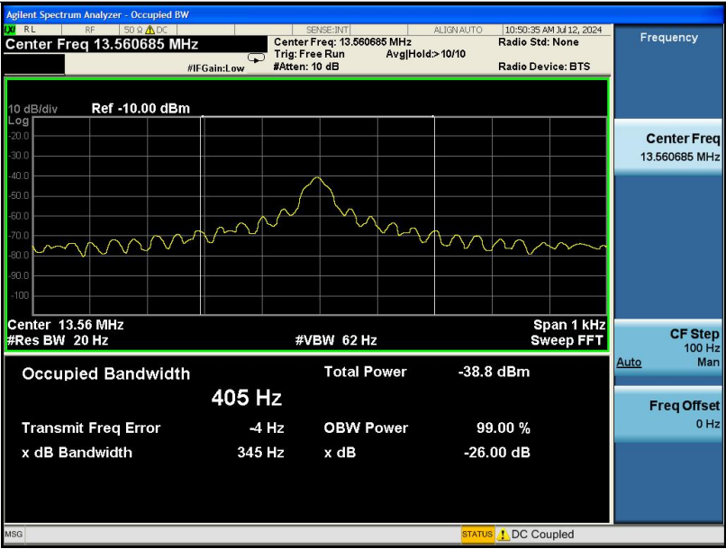
Occupied Bandwidth
