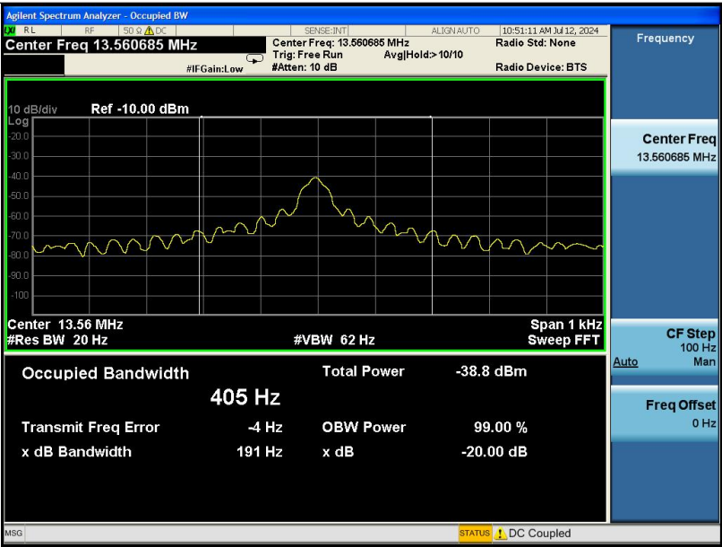
20dB Bandwidth
