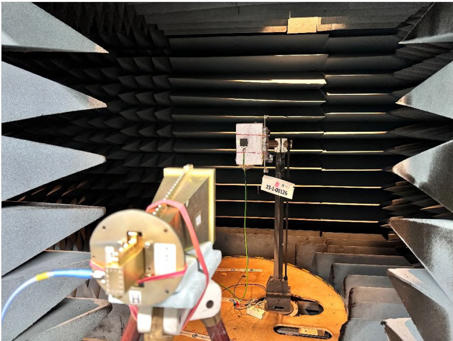
Photograph 4: EUT test setup in the fully anechoic chamber
