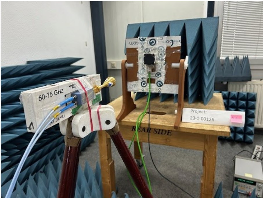
Photograph 6: EUT test setup higher frequency range, Mixer set-up
