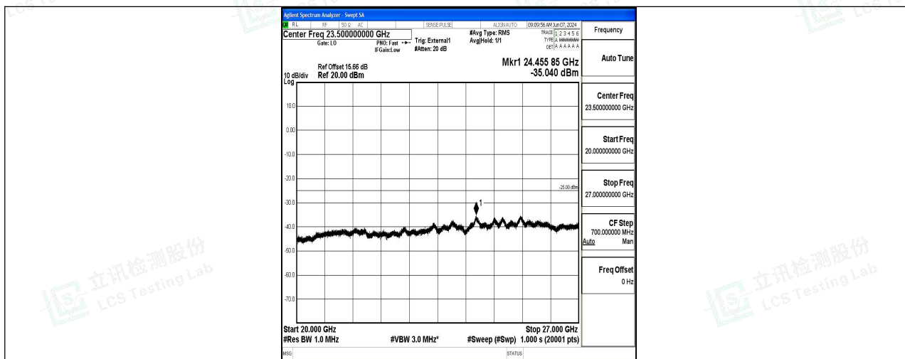
Band41_15MHz_QPSK_41515_1RB#0_20000~27000_20000~27000
