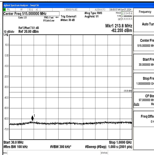
Band41_5MHz_QPSK_40620_1RB#0_30~1000_30~1000
