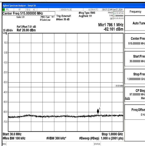
Band41_10MHz_QPSK_40620_1RB#0_30~1000_30~1000
