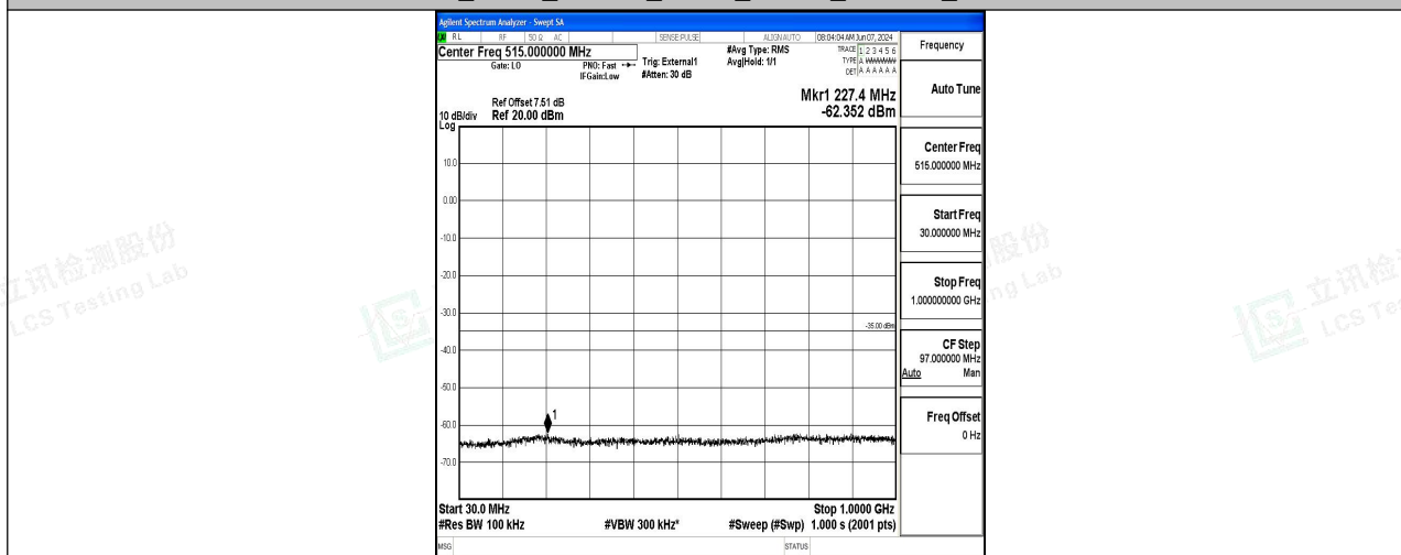
Band41_5MHz_16QAM_39675_1RB#0_30~1000_30~1000
