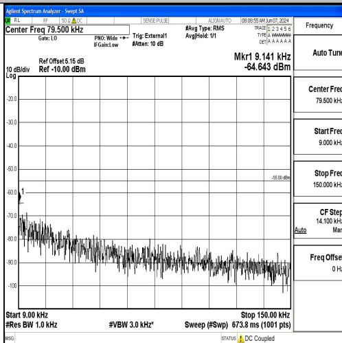
Band41_5MHz_QPSK_41565_1RB#0_0.009~0.15_0.009~0.15
