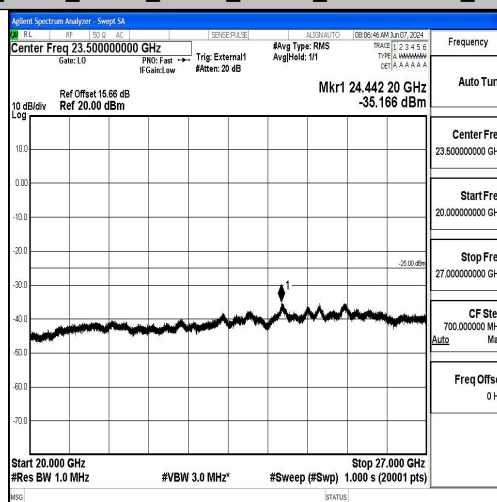
Band41_5MHz_QPSK_40620_1RB#0_20000~27000_20000~27000
