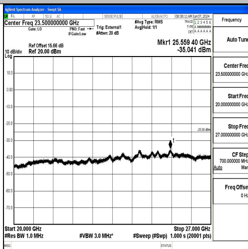
Band41_10MHz_QPSK_40620_1RB#0_20000~27000_20000~27000
