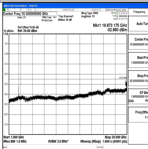
Band41_5MHz_QPSK_40620_1RB#0_1000~20000_1000~20000
