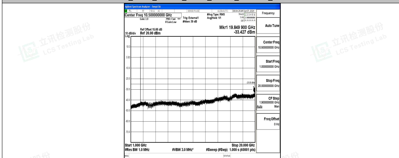
Band41_5MHz_16QAM_39675_1RB#0_1000~20000_1000~20000
