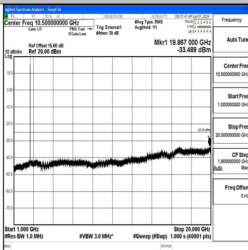
Band41_10MHz_QPSK_40620_1RB#0_1000~20000_1000~20000
