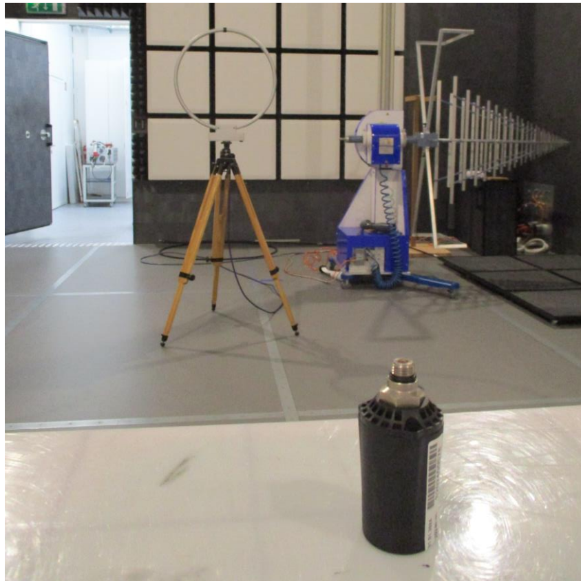
Figure 1: 9 kHz- 30 MHz Radiated emission
