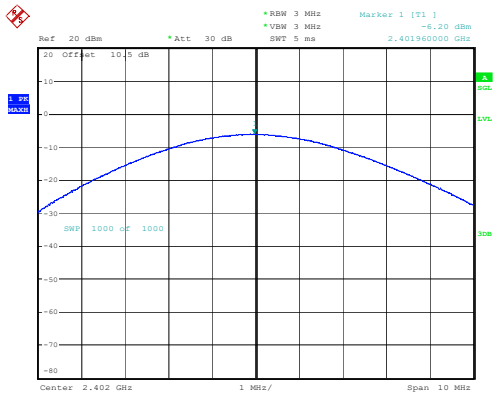
GFSK_Low -6.20dBm
