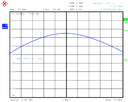
GFSK_High -5.13dBm
