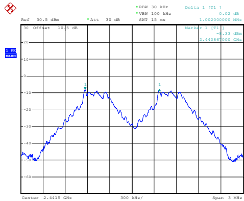
GFSK_Middle 1.002MHz
