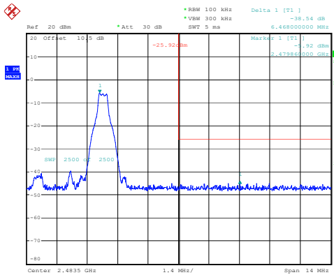
GFSK_High
