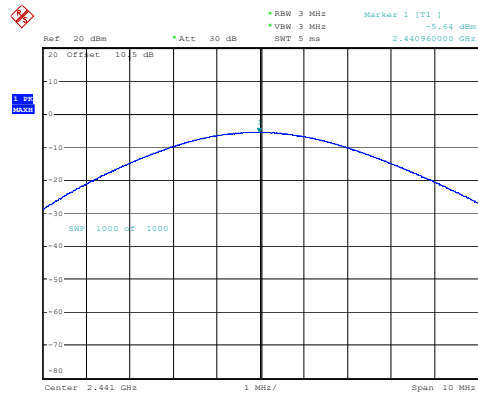
GFSK_Middle -5.64dBm
