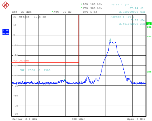
GFSK_Low
