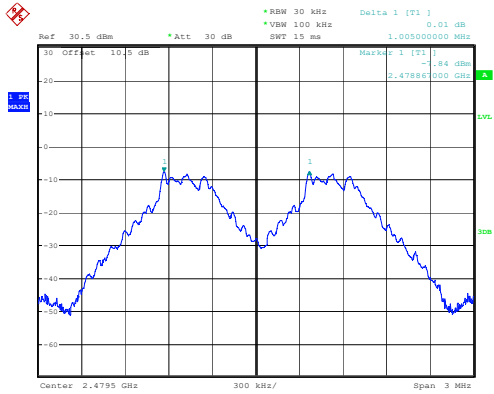
GFSK_High 1.005MHz
