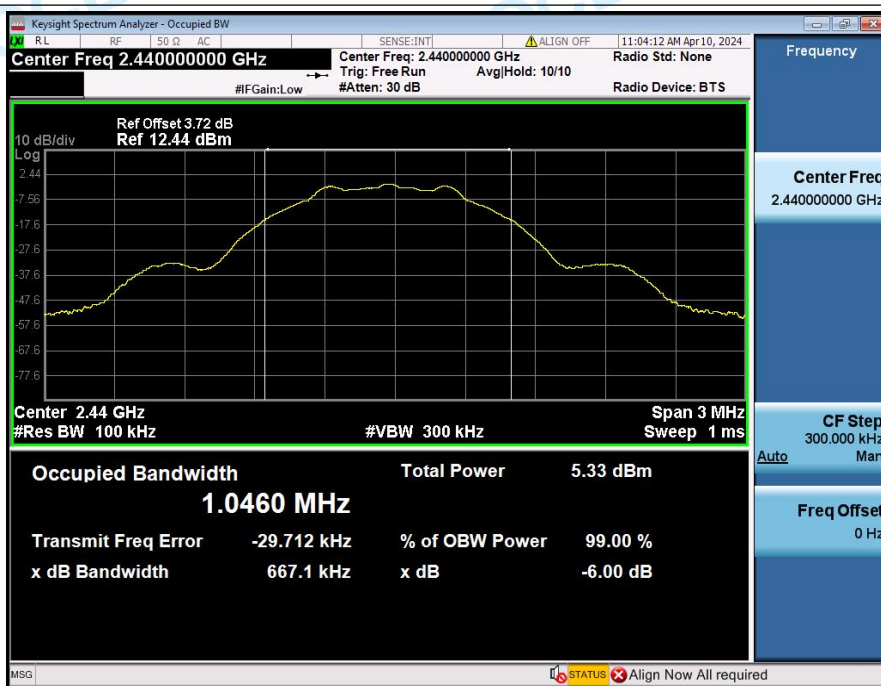
-6dB_Bandwidth_NVNT_ANT1_1Mbps_2440
