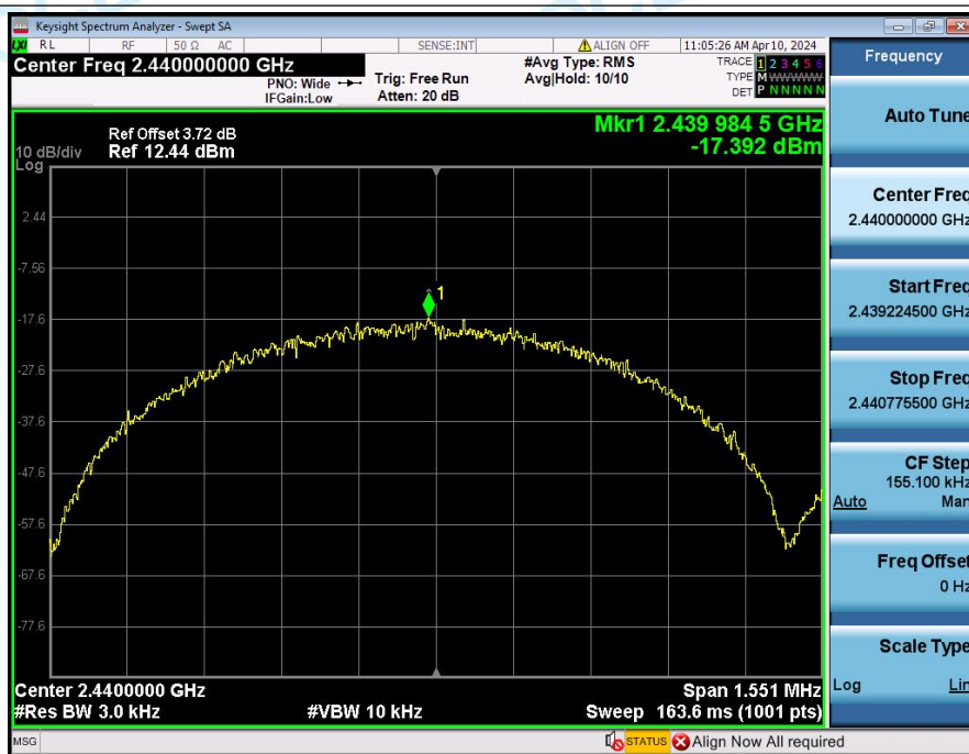
Power_Spectral_Density_NVNT_ANT1_1Mbps_2440
