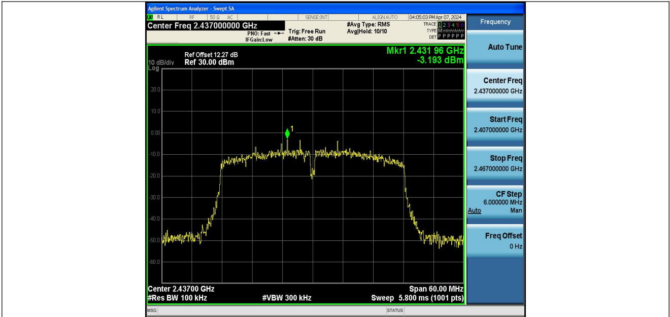
11N40SISO-Ant1-2437-0~Reference-PASS
