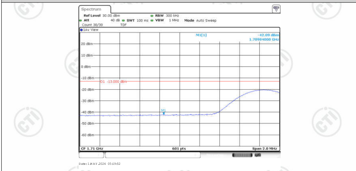
Band66-15MHz-QPSK-132047-1RB#74
