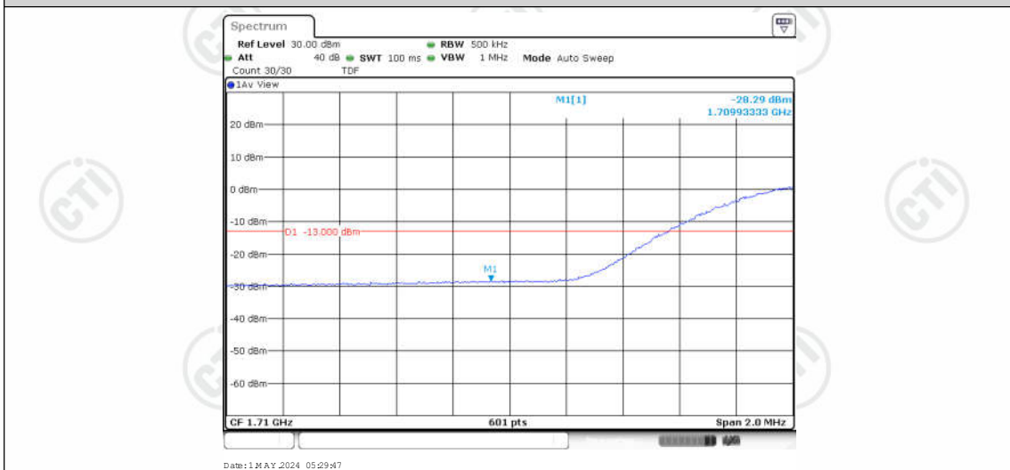
Band66-20MHz-16QAM-132572-1RB#0
