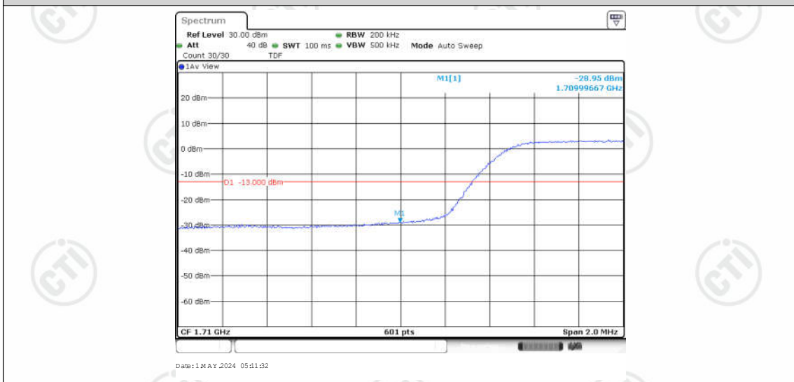
Band66-10MHz-16QAM-132022-50RB#0
