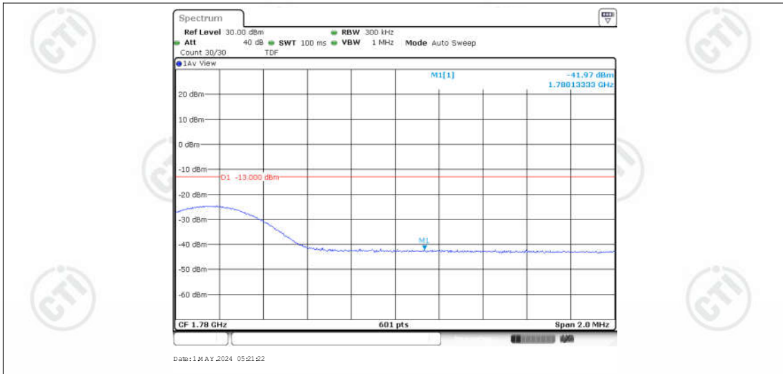
Band66-15MHz-16QAM-132597-1RB#74
