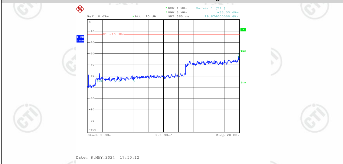
Band66-1.4MHz-16QAM-132322-1RB#0-Range3:2000~20000MHz
