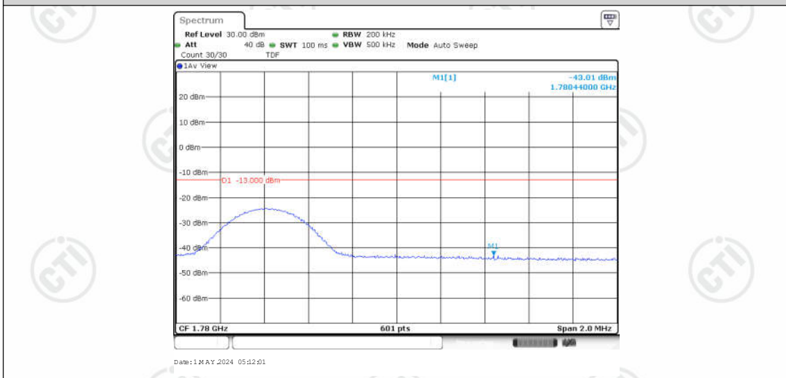
Band66-10MHz-QPSK-132622-1RB#0
