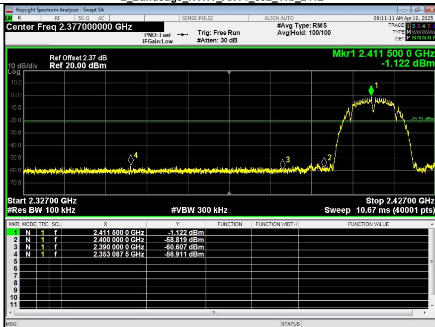
2 Bandedge_NVNT_ANT1_802_11b_2412
