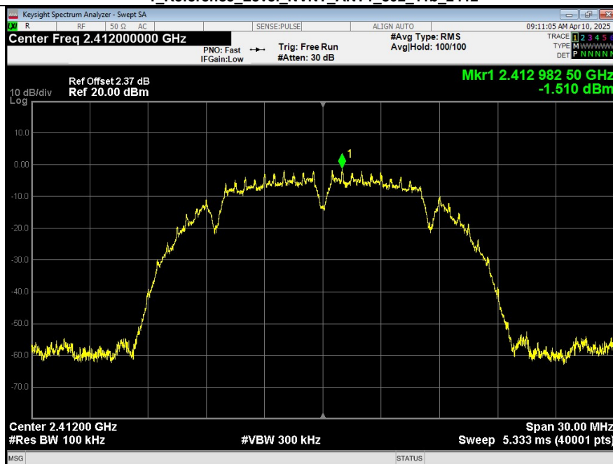
2 Bandedge_NVNT_ANT1_802_11b_2412
