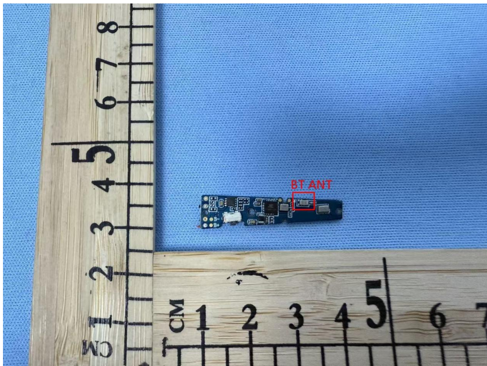
Internal Photos(Right glasses leg)
