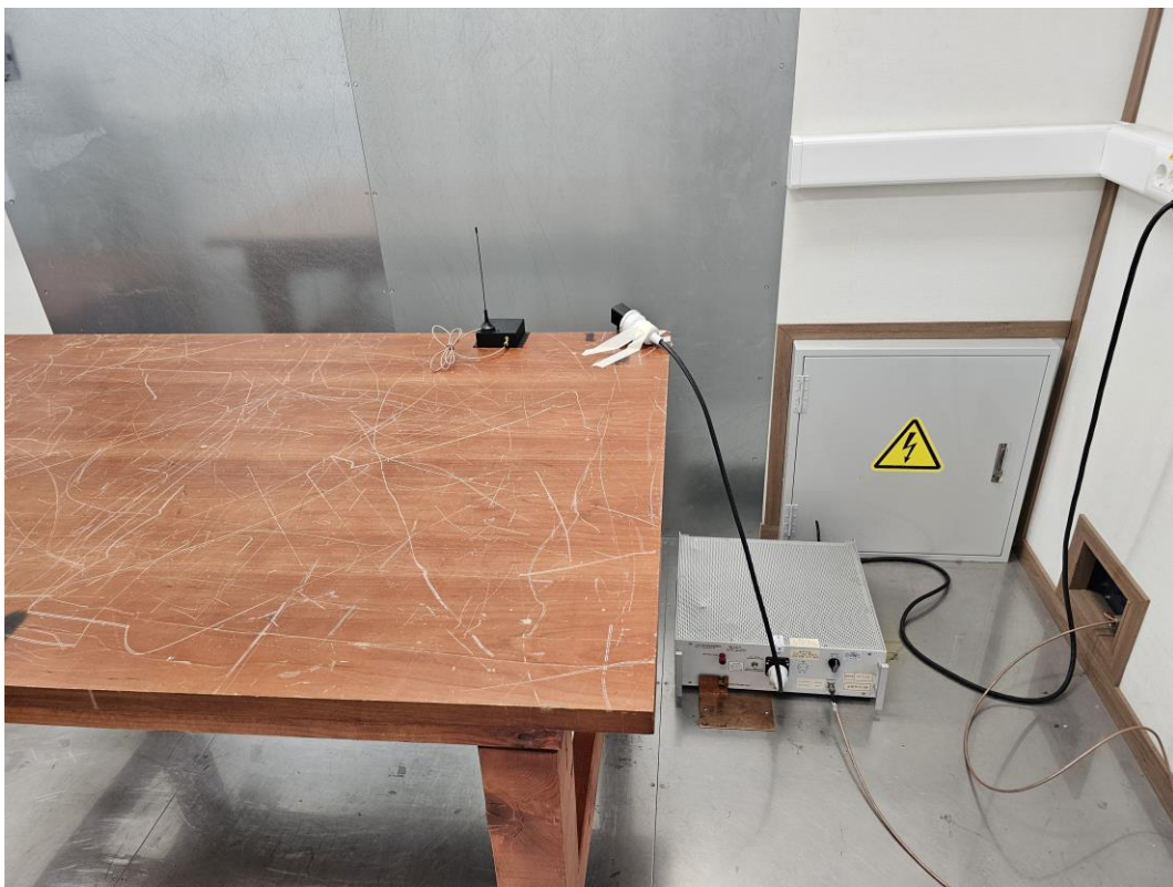
Conducted Emission
