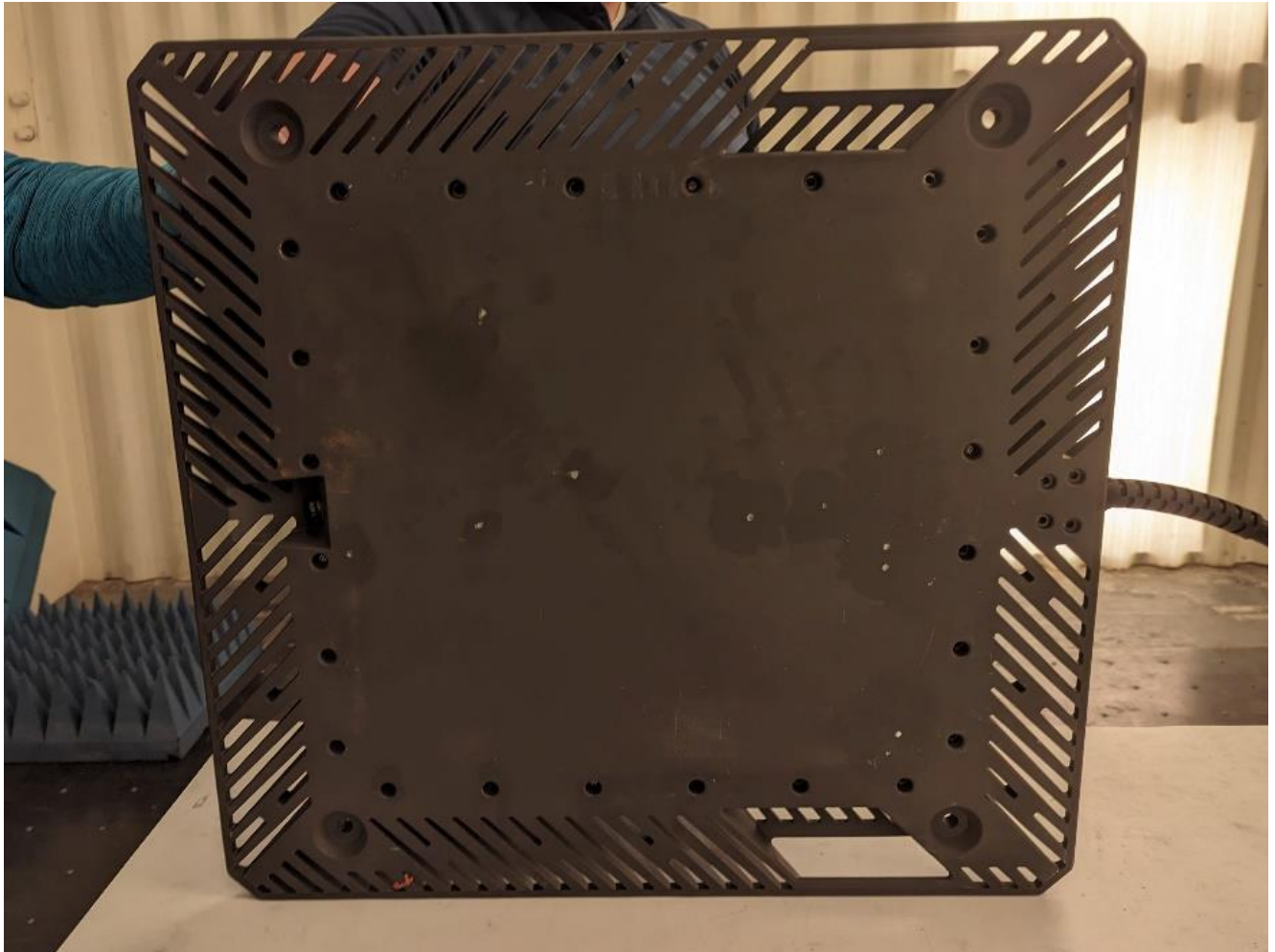
Photograph 2 – Bottom View of the EUT
