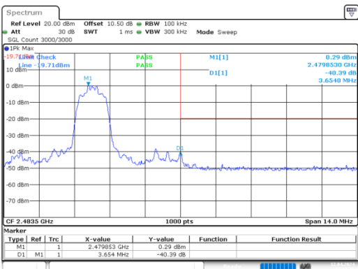
8DPSK_High_3DH1
