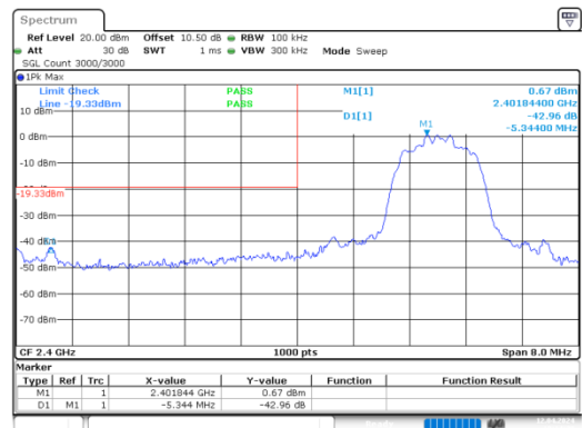
8DPSK_Low_3DH1
