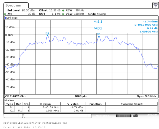
8DPSK_Low_3DH1
