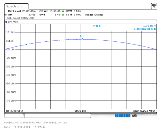
8DPSK_High_3DH1
