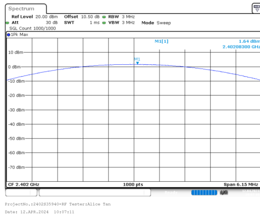
PI/4-DQPSK_Low_2DH1
