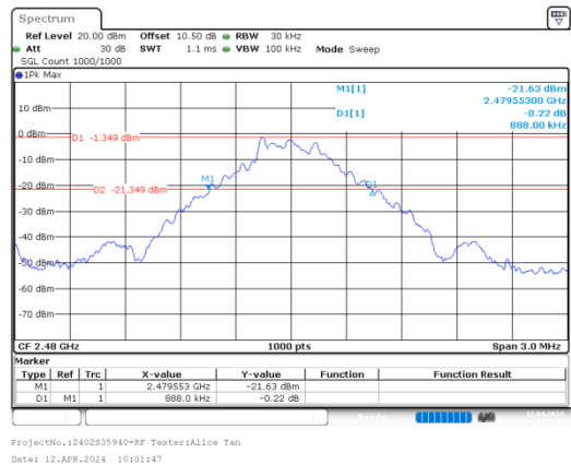
GFSK_High_DH1
