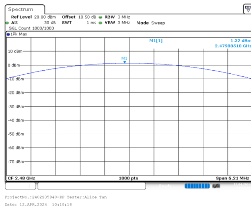
PI/4-DQPSK_High_2DH1
