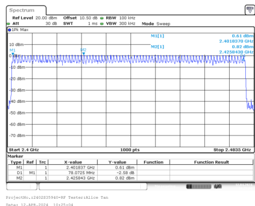
PI/4-DQPSK_Hopping_2DH1
