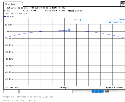
PI/4-DQPSK_Mid_2DH1
