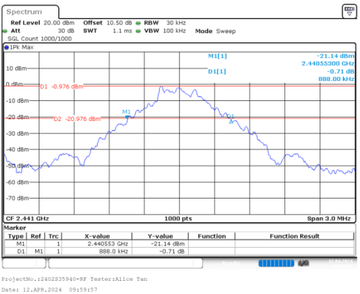
GFSK_Mid_DH1
