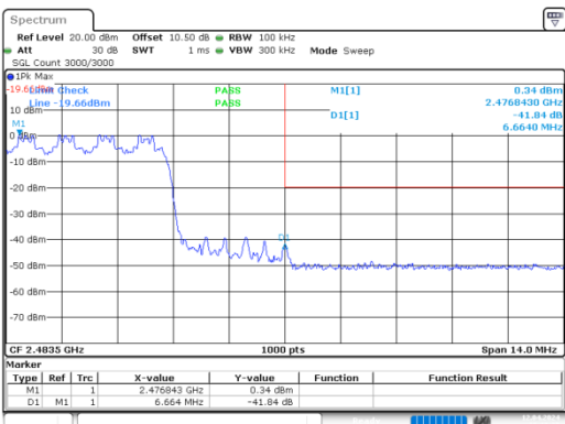
8DPSK_Hopping_Upper_3DH1
