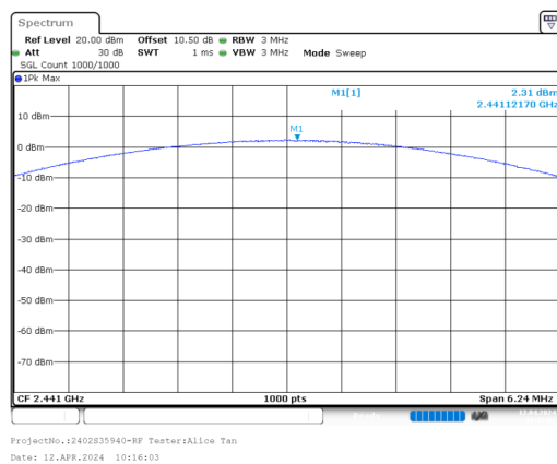
8DPSK_Mid_3DH1
