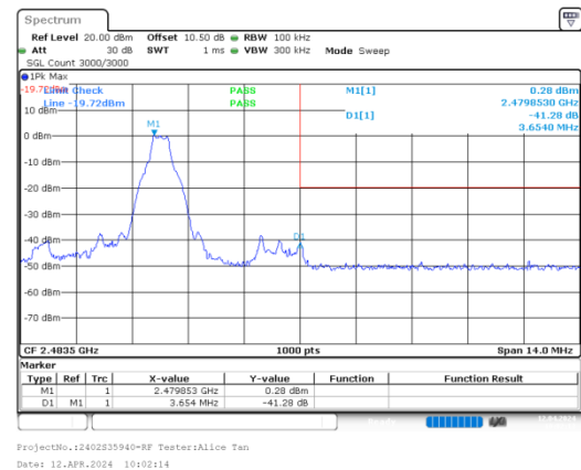
GFSK_High_DH1
