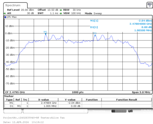
8DPSK_High_3DH1
